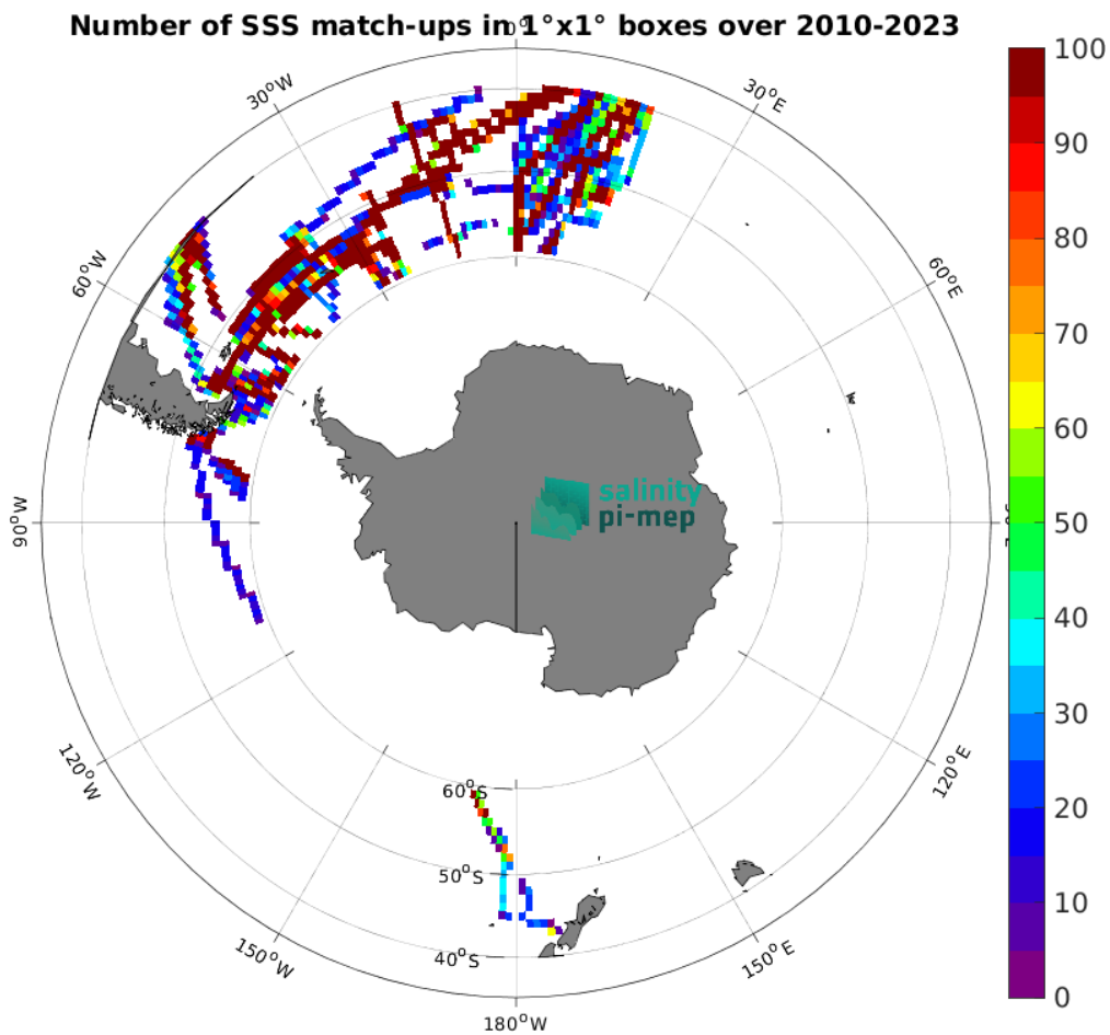
Figure 5: Number of SSS match-ups between TSG (Polarstern) SSS and the CCI SSS L4 Merged-OI v5.5 - 30-day running (ESA) SSS product for the Roaring Forties and Furious Fifties Pi-MEP region over 1^{\circ} \times 1^{\circ} boxes and for the full satellite product period.
