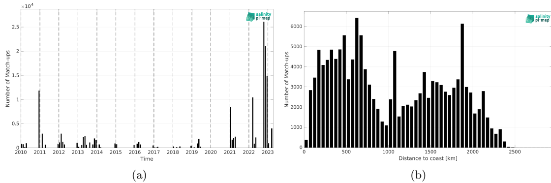
Figure 2: Number of match-ups between TSG (Polarstern) and CCI SSS L4 Merged-OI v5.5 - 30-day running (ESA) SSS as a function of time (a) and as function of the distance to coast (b) over the Roaring Forties and Furious Fifties Pi-MEP region and for the full satellite product period.
