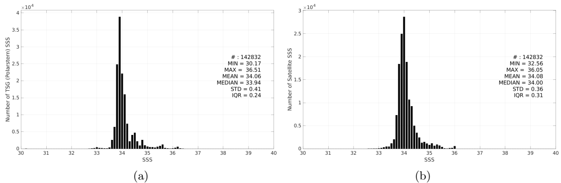
Figure 3: Histograms of SSS from TSG (Polarstern) (a) and CCI SSS L4 Merged-OI v5.5 - 30-day running (ESA) (b) considering all match-up pairs per bins of 0.1 over the Roaring Forties and Furious Fifties Pi-MEP region and for the full satellite product period.
