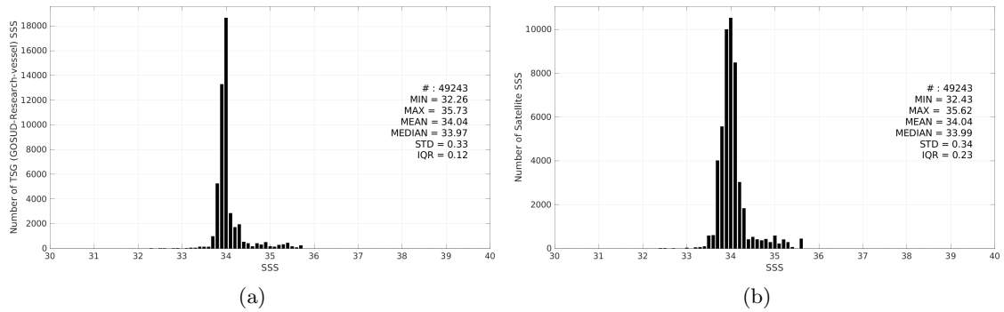
Figure 3: Histograms of SSS from TSG (GOSUD-Research-vessel) (a) and CCI SSS L4 Merged-OI v5.5 - 30-day running (ESA) (b) considering all match-up pairs per bins of 0.1 over the Roaring Forties and Furious Fifties Pi-MEP region and for the full satellite product period.
