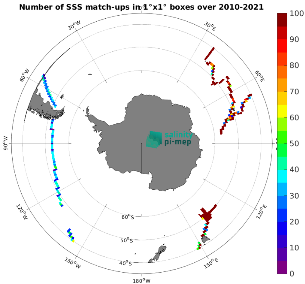
Figure 5: Number of SSS match-ups between TSG (GOSUD-Research-vessel) SSS and the CCI SSS L4 Merged-OI v5.5 - 30-day running (ESA) SSS product for the Roaring Forties and Furious Fifties Pi-MEP region over 1^\circ \times 1^\circ boxes and for the full satellite product period.
