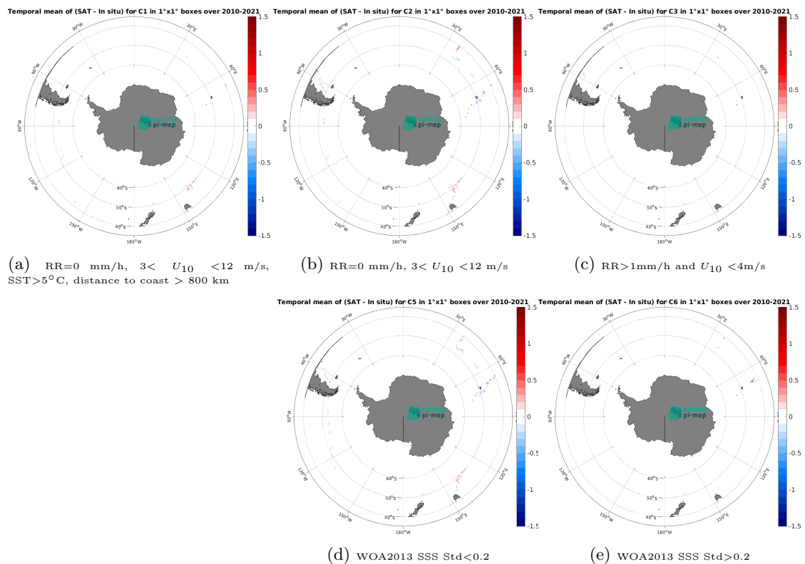
Figure 14: Temporal mean gridded over spatial boxes of size 1^\circ \times 1^\circ of \Delta\text{SSS} (CCI SSS L4 Merged-OI v5.5 - 30-day running (ESA) - TSG (GOSUD-Research-vessel)) for 5 different subdatasets corresponding to:RR=0 mm/h, 3 < U_{10} < 12 m/s, SST>5°C, distance to coast > 800 km (a), RR=0 mm/h, 3 < U_{10} < 12 m/s (b), RR>1mm/h and U_{10} < 4 m/s (c), WOA2013 SSS Std<0.2 (d), WOA2013 SSS Std>0.2 (e).
