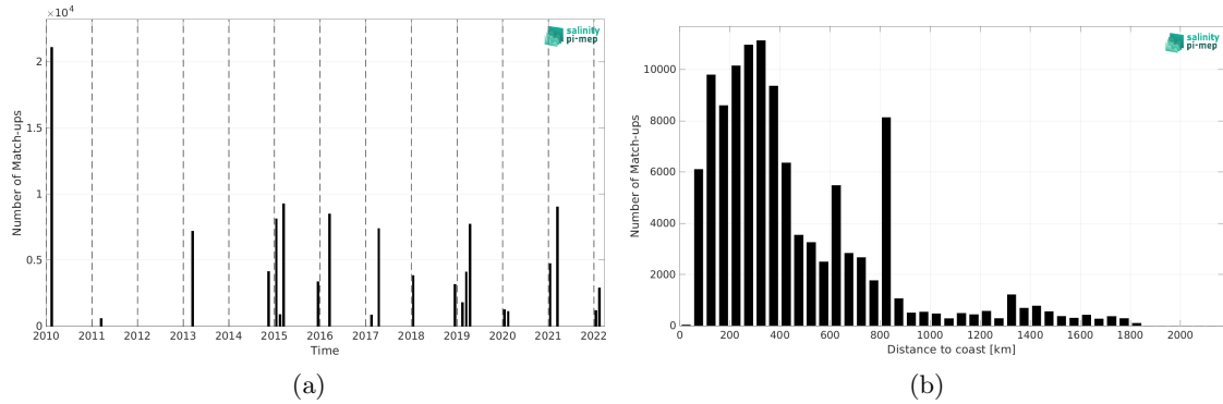
Figure 2: Number of match-ups between TSG (CSIC-UTM) and CCI SSS L4 Merged-OI v5.5 - 30-day running (ESA) SSS as a function of time (a) and as function of the distance to coast (b) over the Roaring Forties and Furious Fifties Pi-MEP region and for the full satellite product period.
