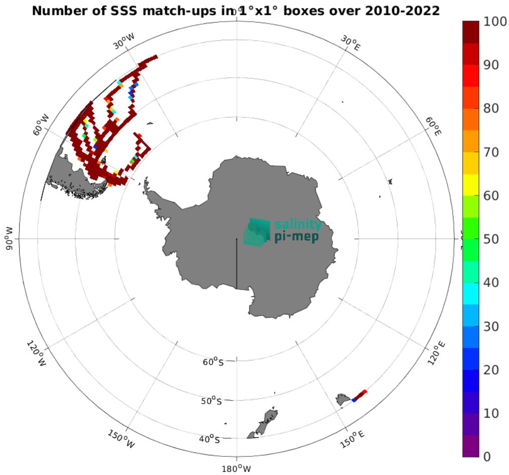
Figure 5: Number of SSS match-ups between TSG (CSIC-UTM) SSS and the CCI SSS L4 Merged-OI v5.5 - 30-day running (ESA) SSS product for the Roaring Forties and Furious Fifties Pi-MEP region over 1^\circ \times 1^\circ boxes and for the full satellite product period.
