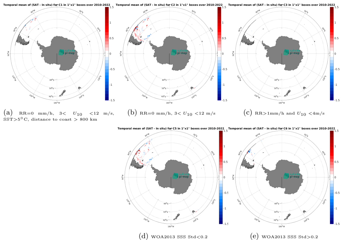
Figure 14: Temporal mean gridded over spatial boxes of size 1^\circ \times 1^\circ of \Delta SSS (CCI SSS L4 Merged-OI v5.5 - 30-day running (ESA) - TSG (CSIC-UTM)) for 5 different subdatasets corresponding to: RR=0 mm/h, 3 < U_{10} < 12 m/s, SST > 5^\circ\text{C} , distance to coast > 800 km (a), RR=0 mm/h, 3 < U_{10} < 12 m/s (b), RR > 1 mm/h and U_{10} < 4 m/s (c), WOA2013 SSS Std < 0.2 (d), WOA2013 SSS Std > 0.2 (e).
