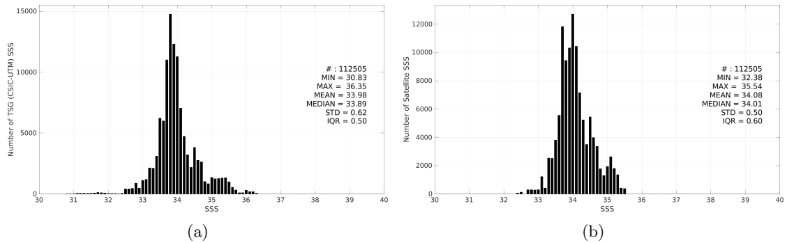
Figure 3: Histograms of SSS from TSG (CSIC-UTM) (a) and CCI SSS L4 Merged-OI v5.5 - 30-day running (ESA) (b) considering all match-up pairs per bins of 0.1 over the Roaring Forties and Furious Fifties Pi-MEP region and for the full satellite product period.
