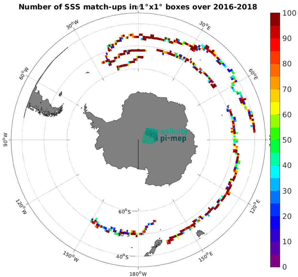
Figure 4: Number of SSS match-ups between Surface drifters SSS and the CCI SSS L4 Merged-OI v5.5 - 30-day running (ESA) SSS product for the Roaring Forties and Furious Fifties Pi-MEP region over 1^\circ \times 1^\circ boxes and for the full satellite product period.
