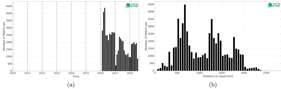
Figure 2: Number of match-ups between Surface drifters and CCI SSS L4 Merged-OI v5.5 - 30-day running (ESA) SSS as a function of time (a) and as function of the distance to coast (b) over the Roaring Forties and Furious Fifties Pi-MEP region and for the full satellite product period.
