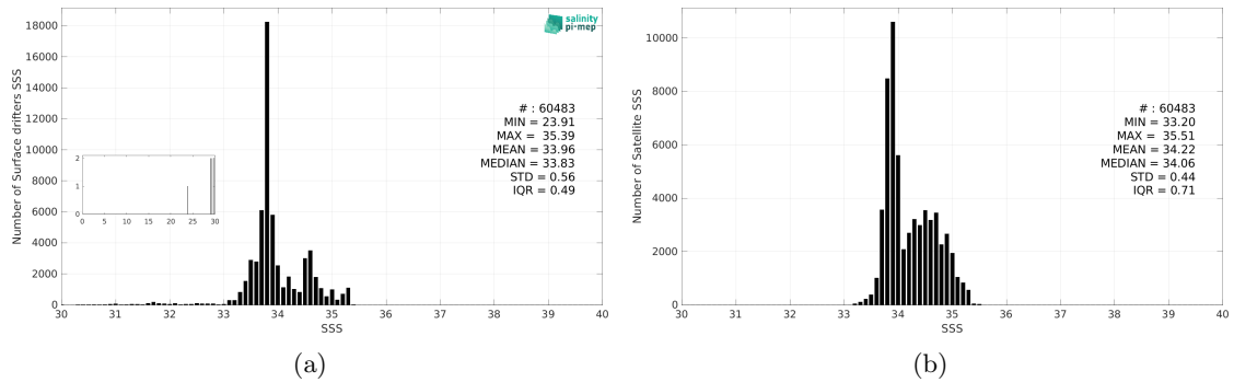
Figure 3: Histograms of SSS from Surface drifters (a) and CCI SSS L4 Merged-OI v5.5 - 30-day running (ESA) (b) considering all match-up pairs per bins of 0.1 over the Roaring Forties and Furious Fifties Pi-MEP region and for the full satellite product period.
