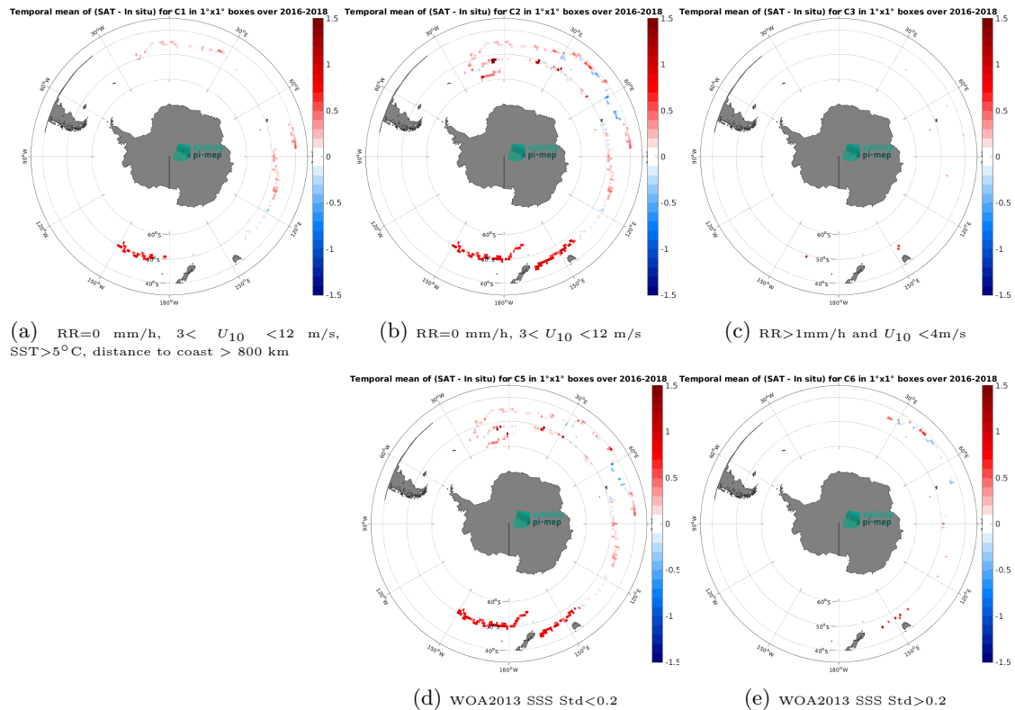
Figure 13: Temporal mean gridded over spatial boxes of size 1^\circ \times 1^\circ of \Delta SSS (CCI SSS L4 Merged-OI v5.5 - 30-day running (ESA) - Surface drifters) for 5 different subdatasets corresponding to: RR=0 mm/h, 3 < U_{10} < 12 m/s, SST > 5^\circ\text{C} , distance to coast > 800 km (a), RR=0 mm/h, 3 < U_{10} < 12 m/s (b), RR > 1 mm/h and U_{10} < 4 m/s (c), WOA2013 SSS Std < 0.2 (d), WOA2013 SSS Std > 0.2 (e).
