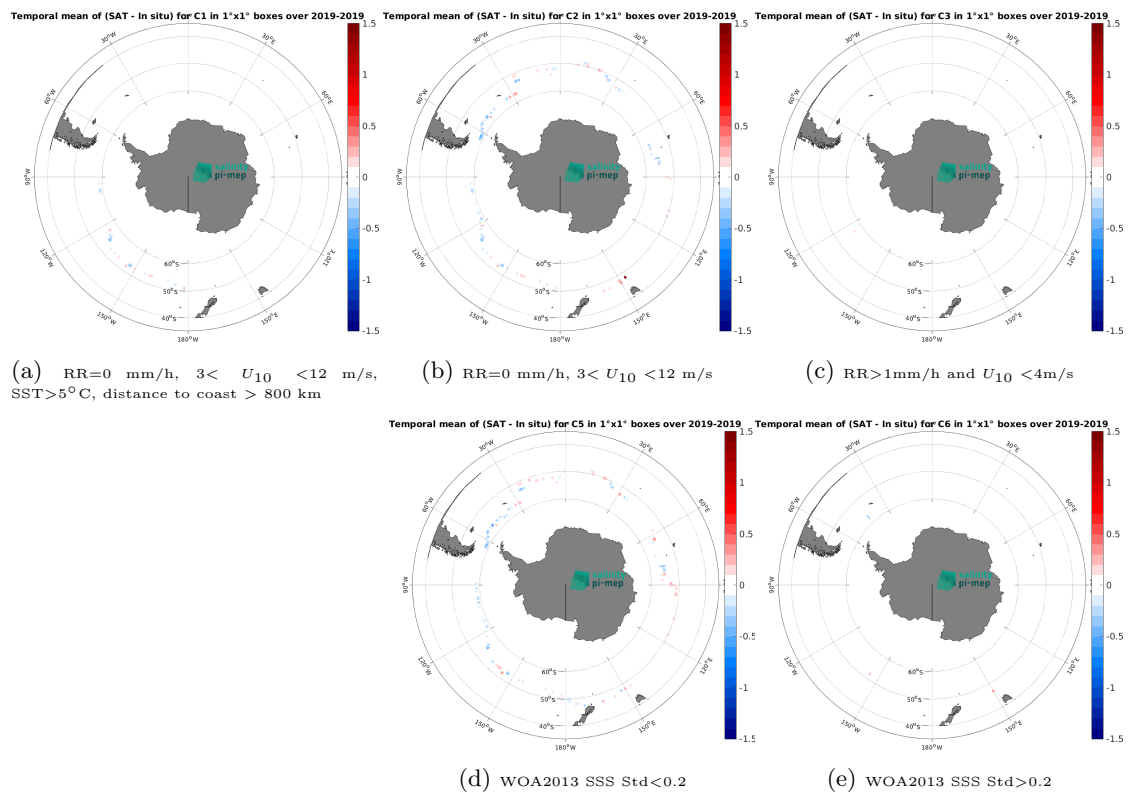
Figure 14: Temporal mean gridded over spatial boxes of size 1^\circ \times 1^\circ of \Delta\text{SSS} (CCI SSS L4 Merged-OI v4.41 - 7-day running (ESA) - Saildrone) for 5 different subdatasets corresponding to:RR=0 mm/h, 3 < U_{10} < 12 m/s, SST > 5°C, distance to coast > 800 km (a), RR=0 mm/h, 3 < U_{10} < 12 m/s (b), RR > 1mm/h and U_{10} < 4 m/s (c), WOA2013 SSS Std < 0.2 (d), WOA2013 SSS Std > 0.2 (e).
