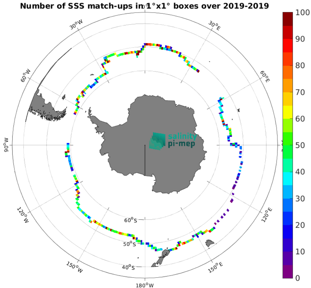
Figure 5: Number of SSS match-ups between Saildrone SSS and the CCI SSS L4 Merged-OI v4.41 - 7-day running (ESA) SSS product for the Roaring Forties and Furious Fifties Pi-MEP region over 1^\circ \times 1^\circ boxes and for the full satellite product period.
