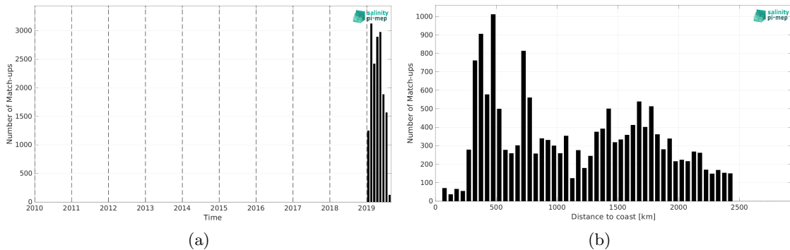
Figure 2: Number of match-ups between Saildrone and CCI SSS L4 Merged-OI v4.41 - 7-day running (ESA) SSS as a function of time (a) and as function of the distance to coast (b) over the Roaring Forties and Furious Fifties Pi-MEP region and for the full satellite product period.
