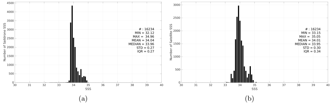
Figure 3: Histograms of SSS from Saildrone (a) and CCI SSS L4 Merged-OI v4.41 - 7-day running (ESA) (b) considering all match-up pairs per bins of 0.1 over the Roaring Forties and Furious Fifties Pi-MEP region and for the full satellite product period.
