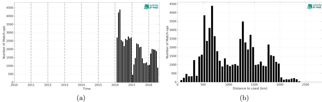
Figure 2: Number of match-ups between Surface drifters and CCI SSS L4 Merged-OI v4.41 - 7-day running (ESA) SSS as a function of time (a) and as function of the distance to coast (b) over the Roaring Forties and Furious Fifties Pi-MEP region and for the full satellite product period.
