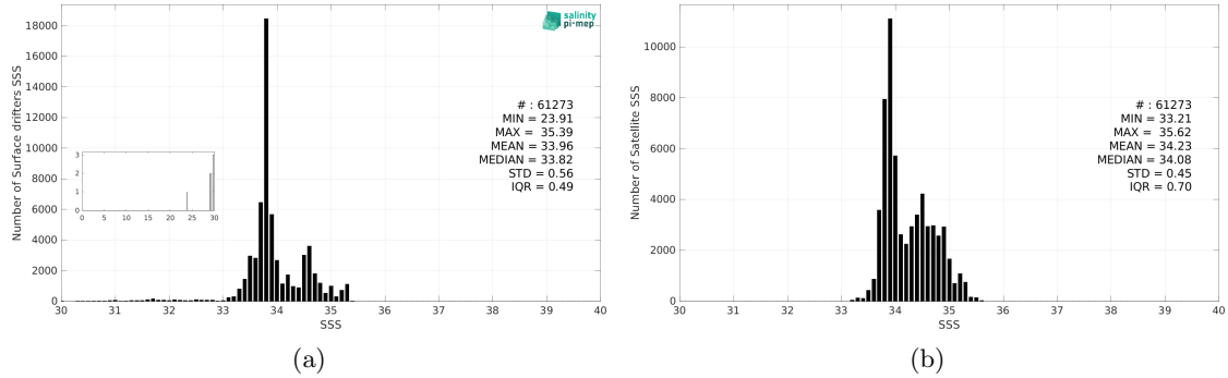
Figure 3: Histograms of SSS from Surface drifters (a) and CCI SSS L4 Merged-OI v4.41 - 7-day running (ESA) (b) considering all match-up pairs per bins of 0.1 over the Roaring Forties and Furious Fifties Pi-MEP region and for the full satellite product period.
