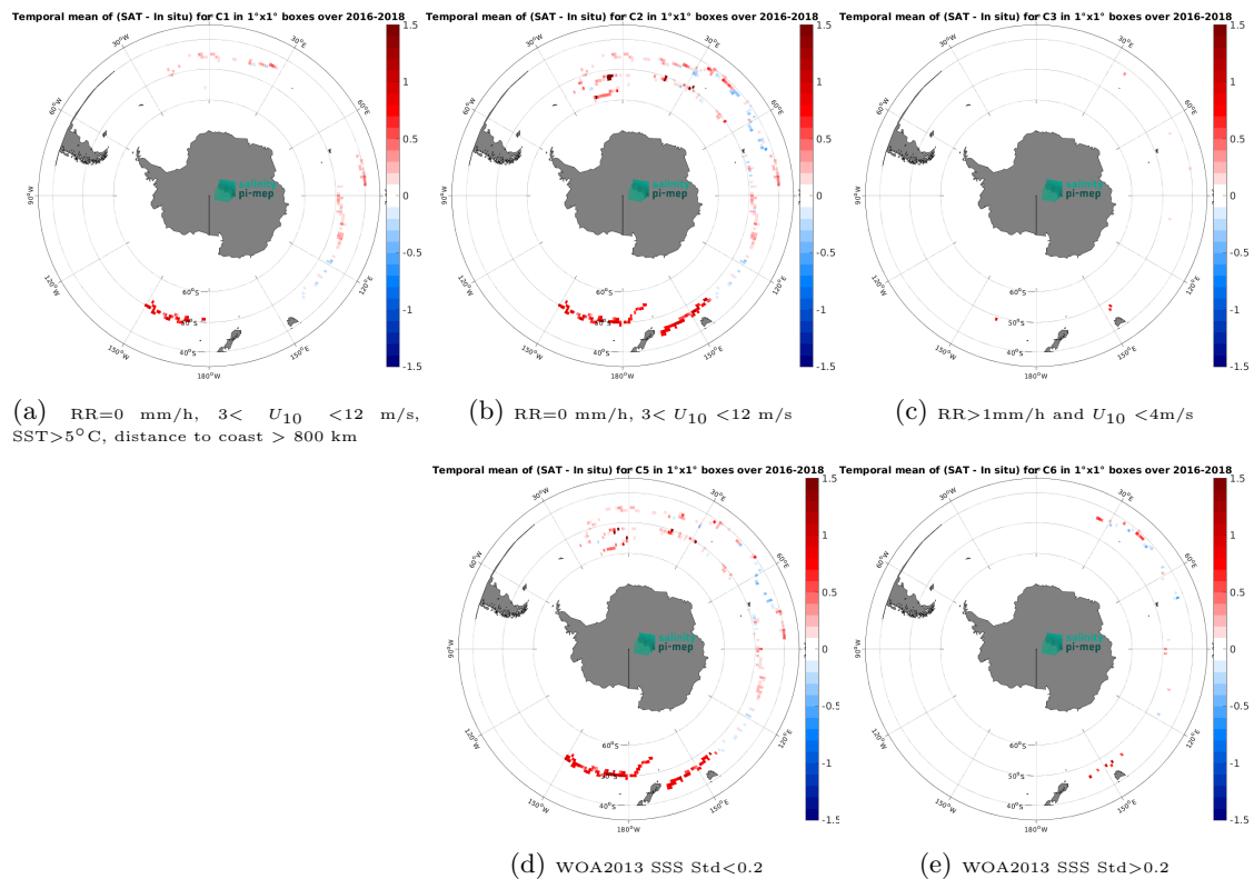
Figure 13: Temporal mean gridded over spatial boxes of size 1^\circ \times 1^\circ of \Delta SSS (CCI SSS L4 Merged-OI v4.41 - 7-day running (ESA) - Surface drifters) for 5 different subdatasets corresponding to:RR=0 mm/h, 3 < U_{10} < 12 m/s, SST >5^\circ C, distance to coast > 800 km (a), RR=0 mm/h, 3 < U_{10} < 12 m/s (b), RR >1 mm/h and U_{10} < 4 m/s (c), WOA2013 SSS Std <0.2 (d), WOA2013 SSS Std >0.2 (e).
