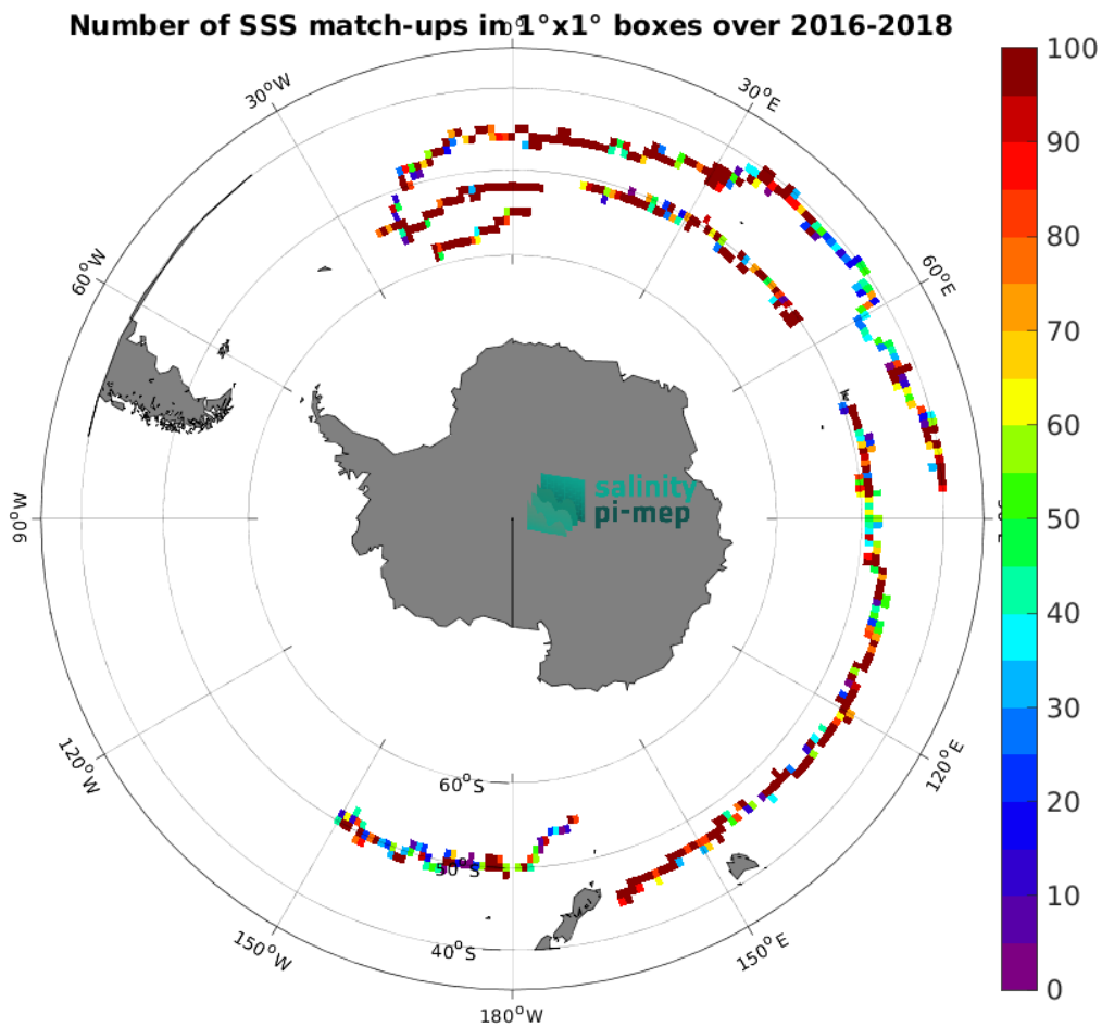
Figure 4: Number of SSS match-ups between Surface drifters SSS and the CCI SSS L4 Merged-OI v4.41 - 7-day running (ESA) SSS product for the Roaring Forties and Furious Fifties Pi-MEP region over 1^\circ \times 1^\circ boxes and for the full satellite product period.
