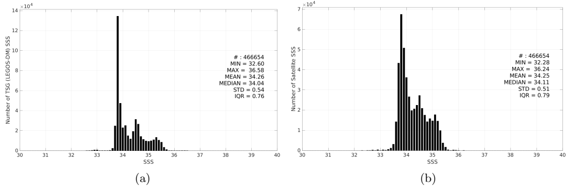
Figure 3: Histograms of SSS from TSG (LEGOS-DM) (a) and CCI SSS L4 Merged-OI v4.41 - 30-day running (ESA) (b) considering all match-up pairs per bins of 0.1 over the Roaring Forties and Furious Fifties Pi-MEP region and for the full satellite product period.
