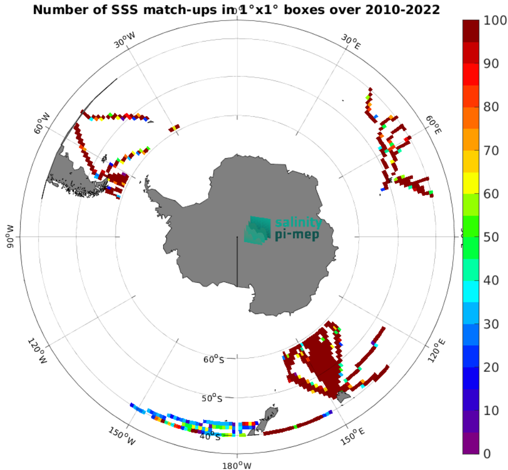
Figure 5: Number of SSS match-ups between TSG (LEGOS-DM) SSS and the CCI SSS L4 Merged-OI v4.41 - 30-day running (ESA) SSS product for the Roaring Forties and Furious Fifties Pi-MEP region over 1^\circ \times 1^\circ boxes and for the full satellite product period.
