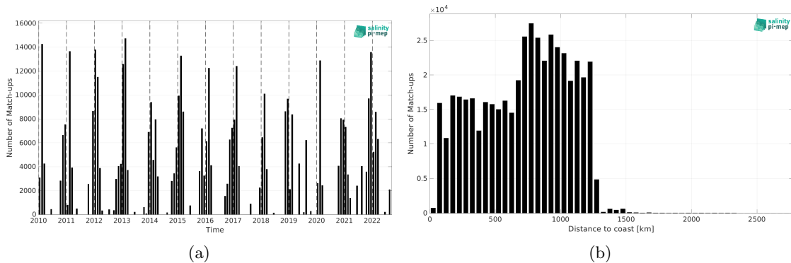
Figure 2: Number of match-ups between TSG (LEGOS-DM) and CCI SSS L4 Merged-OI v4.41 - 30-day running (ESA) SSS as a function of time (a) and as function of the distance to coast (b) over the Roaring Forties and Furious Fifties Pi-MEP region and for the full satellite product period.
