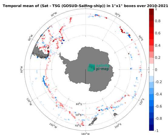
(e) MEAN( \Delta SSS) (Satellite - TSG (GOSUD-Sailing-ship))
