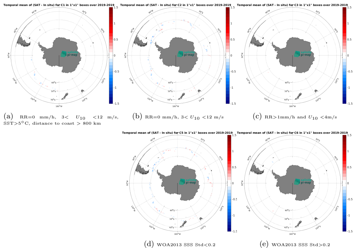
Figure 14: Temporal mean gridded over spatial boxes of size 1^\circ \times 1^\circ of \Delta\text{SSS} (CCI SSS L4 Merged-OI v4.41 - 30-day running (ESA) - Saildrone) for 5 different subdatasets corresponding to:RR=0 mm/h, 3 < U_{10} < 12 m/s, SST>5°C, distance to coast > 800 km (a), RR=0 mm/h, 3 < U_{10} < 12 m/s (b), RR>1mm/h and U_{10} < 4 m/s (c), WOA2013 SSS Std<0.2 (d), WOA2013 SSS Std>0.2 (e).
