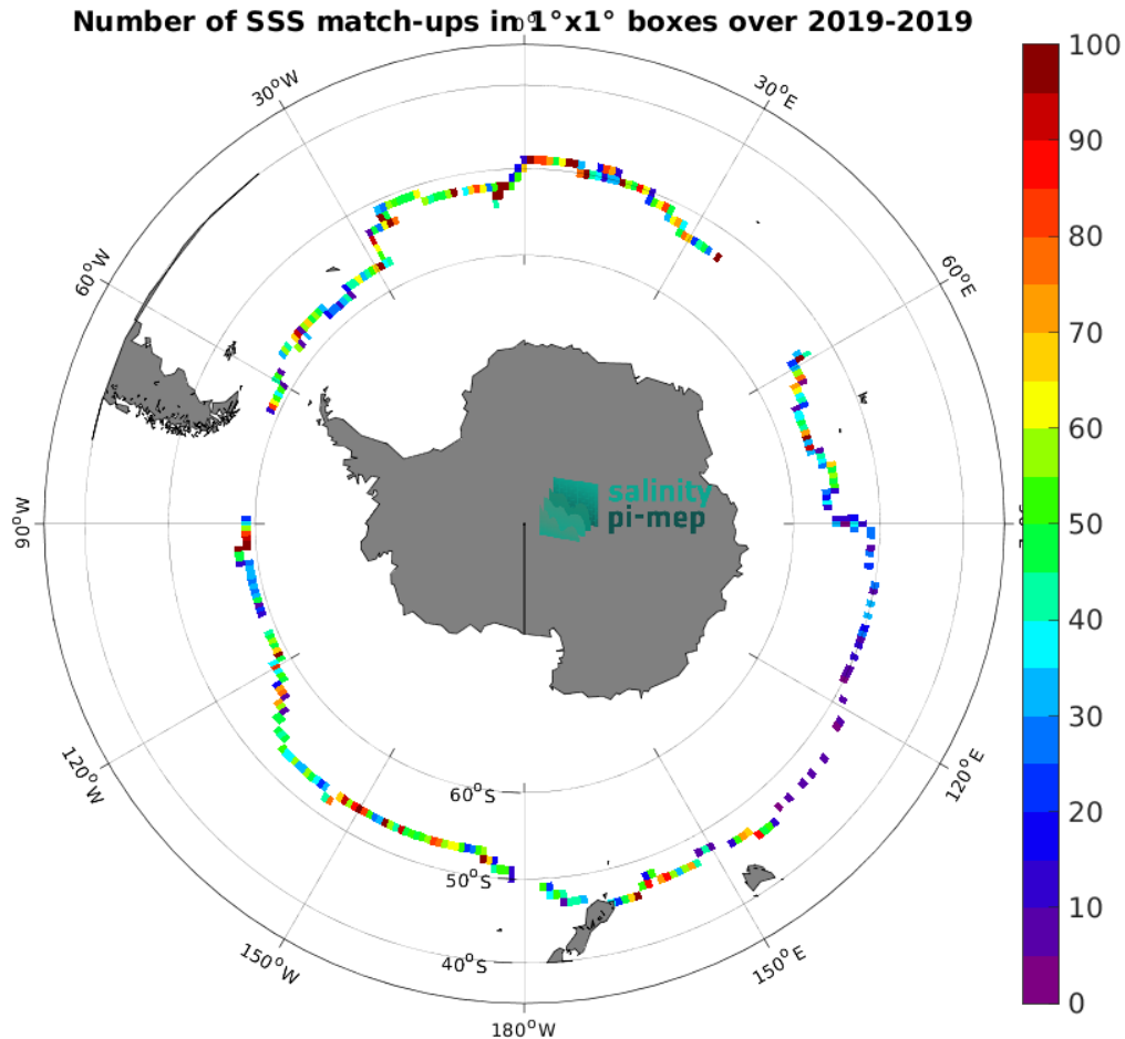
Figure 5: Number of SSS match-ups between Saildrone SSS and the CCI SSS L4 Merged-OI v4.41 - 30-day running (ESA) SSS product for the Roaring Forties and Furious Fifties Pi-MEP region over 1^\circ \times 1^\circ boxes and for the full satellite product period.
