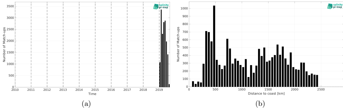
Figure 2: Number of match-ups between Saildrone and CCI SSS L4 Merged-OI v4.41 - 30-day running (ESA) SSS as a function of time (a) and as function of the distance to coast (b) over the Roaring Forties and Furious Fifties Pi-MEP region and for the full satellite product period.
