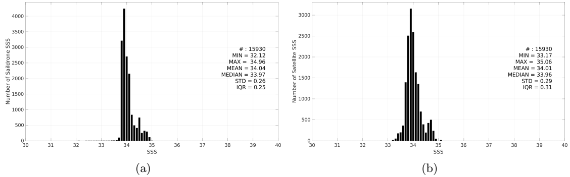
Figure 3: Histograms of SSS from Saildrone (a) and CCI SSS L4 Merged-OI v4.41 - 30-day running (ESA) (b) considering all match-up pairs per bins of 0.1 over the Roaring Forties and Furious Fifties Pi-MEP region and for the full satellite product period.
