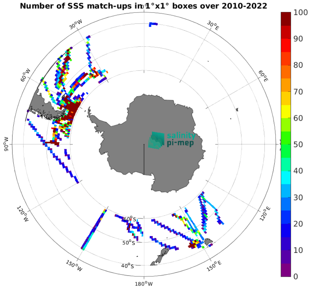
Figure 4: Number of SSS match-ups between TSG (SAMOS) SSS and the CCI SSS L4 Merged-OI v4.4 - 7-day running (ESA) SSS product for the Roaring Forties and Furious Fifties Pi-MEP region over 1^\circ \times 1^\circ boxes and for the full satellite product period.
