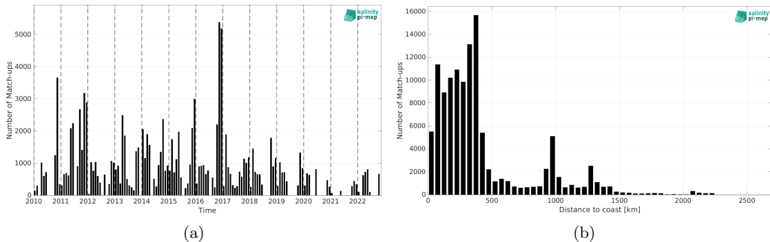
Figure 1: Number of match-ups between TSG (SAMOS) and CCI SSS L4 Merged-OI v4.4 - 7-day running (ESA) SSS as a function of time (a) and as function of the distance to coast (b) over the Roaring Forties and Furious Fifties Pi-MEP region and for the full satellite product period.
