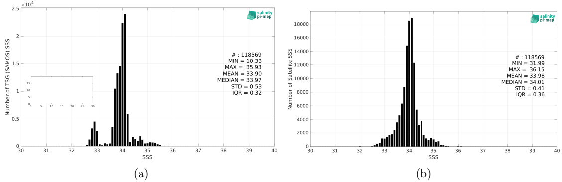
Figure 2: Histograms of SSS from TSG (SAMOS) (a) and CCI SSS L4 Merged-OI v4.4 - 7-day running (ESA) (b) considering all match-up pairs per bins of 0.1 over the Roaring Forties and Furious Fifties Pi-MEP region and for the full satellite product period.
