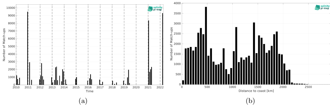
Figure 1: Number of match-ups between TSG (Polarstern) and CCI SSS L4 Merged-OI v4.4 - 7-day running (ESA) SSS as a function of time (a) and as function of the distance to coast (b) over the Roaring Forties and Furious Fifties Pi-MEP region and for the full satellite product period.
