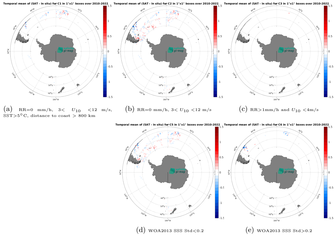
Figure 12: Temporal mean gridded over spatial boxes of size 1^{\circ}\times 1^{\circ} of \Delta\text{SSS} (CCI SSS L4 Merged-OI v4.4 - 7-day running (ESA) - TSG (Polarstern)) for 5 different subdatasets corresponding to:RR=0 mm/h, 3 < U_{10} < 12 m/s, SST >5^{\circ}\text{C} , distance to coast > 800 km (a), RR=0 mm/h, 3 < U_{10} < 12 m/s (b), RR >1 mm/h and U_{10} < 4 m/s (c), WOA2013 SSS Std <0.2 (d), WOA2013 SSS Std >0.2 (e).
