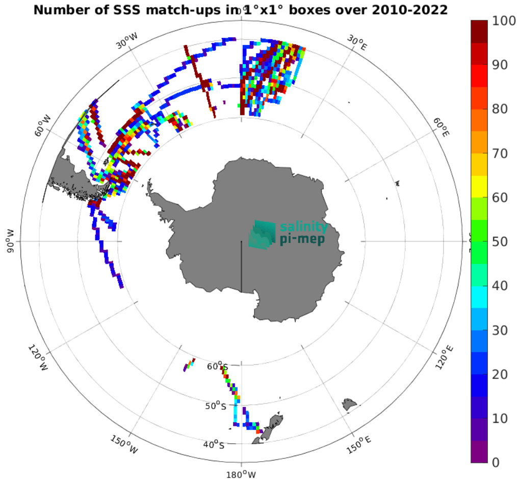
Figure 4: Number of SSS match-ups between TSG (Polarstern) SSS and the CCI SSS L4 Merged-OI v4.4 - 7-day running (ESA) SSS product for the Roaring Forties and Furious Fifties Pi-MEP region over 1^\circ \times 1^\circ boxes and for the full satellite product period.
