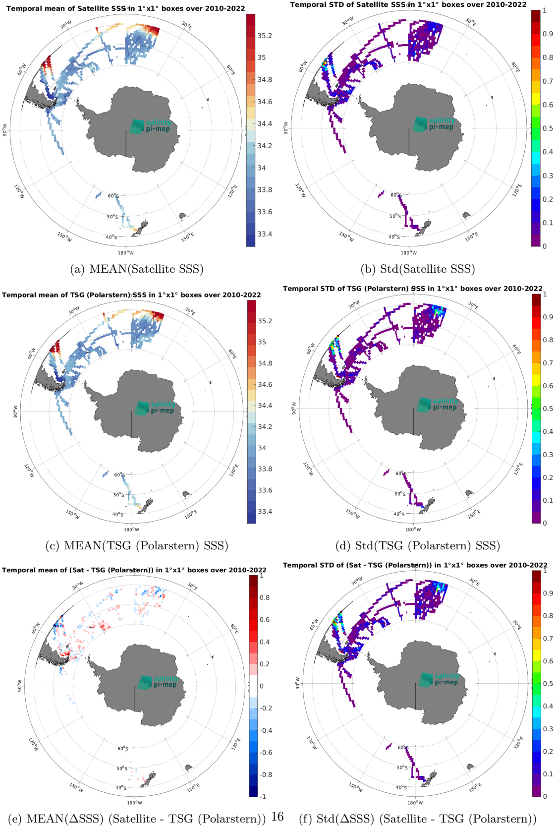
Figure 6: Temporal mean (left) and Std (right) of SSS from CCI SSS L4 Merged-OI v4.4 - 7-day running (ESA) (top), TSG (Polarstern) (middle), and of \Delta SSS (Satellite - TSG (Polarstern)). Only match-up pairs are used to generate these maps.
