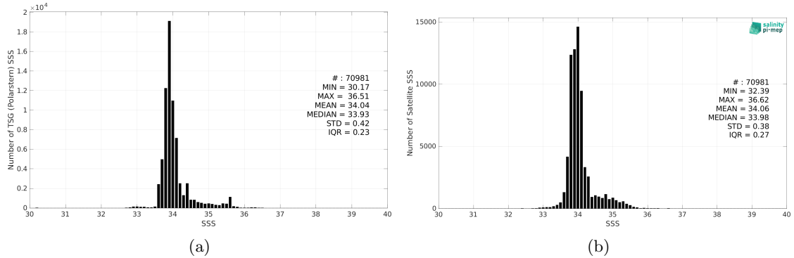
Figure 2: Histograms of SSS from TSG (Polarstern) (a) and CCI SSS L4 Merged-OI v4.4 - 7-day running (ESA) (b) considering all match-up pairs per bins of 0.1 over the Roaring Forties and Furious Fifties Pi-MEP region and for the full satellite product period.
