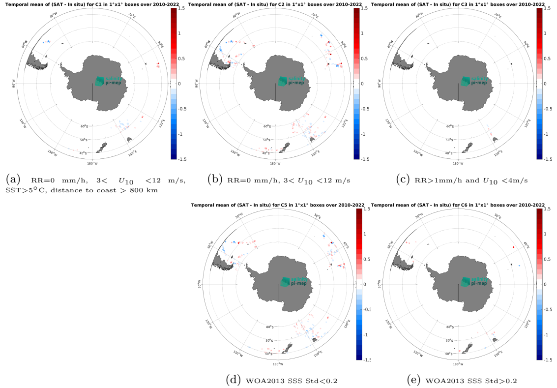
Figure 12: Temporal mean gridded over spatial boxes of size 1^{\circ}\times 1^{\circ} of \Delta\text{SSS} (CCI SSS L4 Merged-OI v4.4 - 7-day running (ESA) - TSG (LEGOS-DM)) for 5 different subdatasets corresponding to:RR=0 mm/h, 3 < U_{10} < 12 m/s, SST >5^{\circ}\text{C} , distance to coast > 800 km (a), RR=0 mm/h, 3 < U_{10} < 12 m/s (b), RR >1 mm/h and U_{10} < 4 m/s (c), WOA2013 SSS Std <0.2 (d), WOA2013 SSS Std >0.2 (e).
