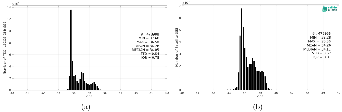
Figure 2: Histograms of SSS from TSG (LEGOS-DM) (a) and CCI SSS L4 Merged-OI v4.4 - 7-day running (ESA) (b) considering all match-up pairs per bins of 0.1 over the Roaring Forties and Furious Fifties Pi-MEP region and for the full satellite product period.
