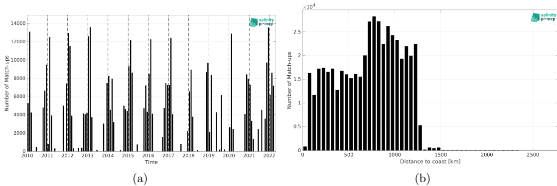
Figure 1: Number of match-ups between TSG (LEGOS-DM) and CCI SSS L4 Merged-OI v4.4 - 7-day running (ESA) SSS as a function of time (a) and as function of the distance to coast (b) over the Roaring Forties and Furious Fifties Pi-MEP region and for the full satellite product period.
