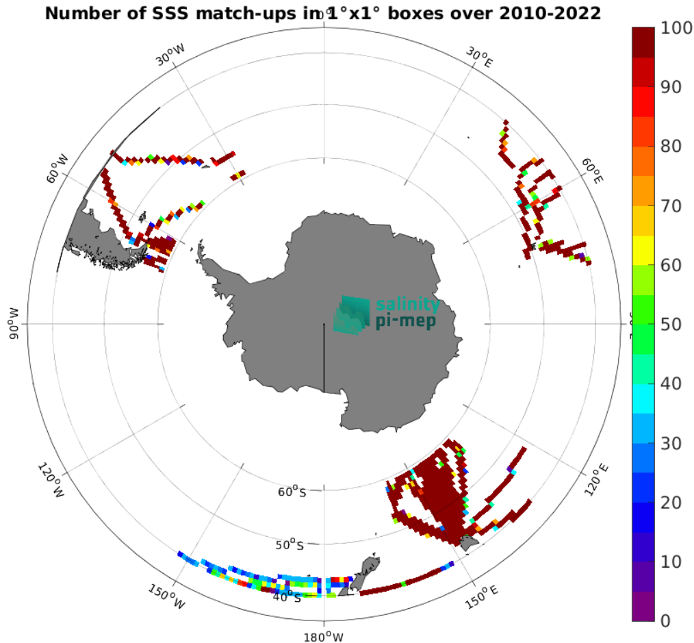
Figure 4: Number of SSS match-ups between TSG (LEGOS-DM) SSS and the CCI SSS L4 Merged-OI v4.4 - 7-day running (ESA) SSS product for the Roaring Forties and Furious Fifties Pi-MEP region over 1^\circ \times 1^\circ boxes and for the full satellite product period.
