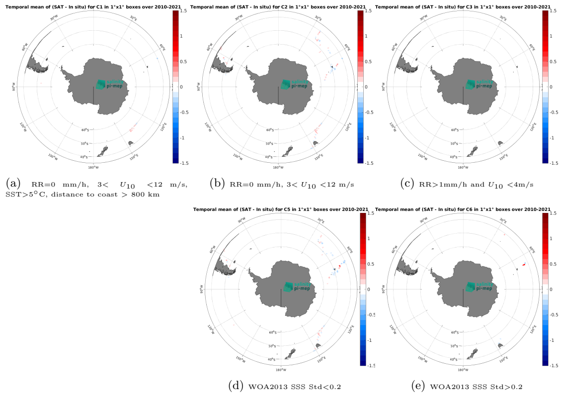
Figure 12: Temporal mean gridded over spatial boxes of size 1^\circ \times 1^\circ of \Delta\text{SSS} (CCI SSS L4 Merged-OI v4.4 - 7-day running (ESA) - TSG (GOSUD-Research-vessel)) for 5 different subdatasets corresponding to: RR=0 mm/h, 3 < U_{10} < 12 m/s, SST > 5^\circ\text{C} , distance to coast > 800 km (a), RR=0 mm/h, 3 < U_{10} < 12 m/s (b), RR > 1 mm/h and U_{10} < 4 m/s (c), WOA2013 SSS Std < 0.2 (d), WOA2013 SSS Std > 0.2 (e).
