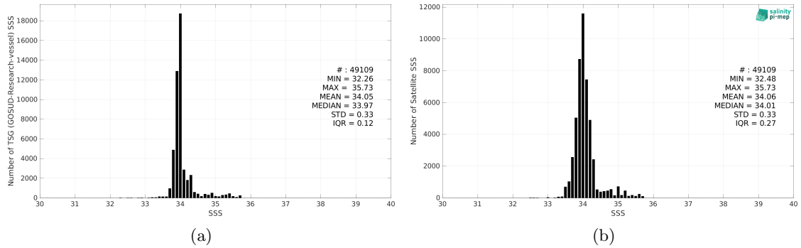
Figure 2: Histograms of SSS from TSG (GOSUD-Research-vessel) (a) and CCI SSS L4 Merged-OI v4.4 - 7-day running (ESA) (b) considering all match-up pairs per bins of 0.1 over the Roaring Forties and Furious Fifties Pi-MEP region and for the full satellite product period.
