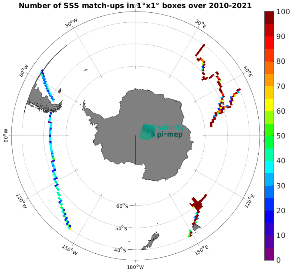
Figure 4: Number of SSS match-ups between TSG (GOSUD-Research-vessel) SSS and the CCI SSS L4 Merged-OI v4.4 - 7-day running (ESA) SSS product for the Roaring Forties and Furious Fifties Pi-MEP region over 1^\circ \times 1^\circ boxes and for the full satellite product period.
