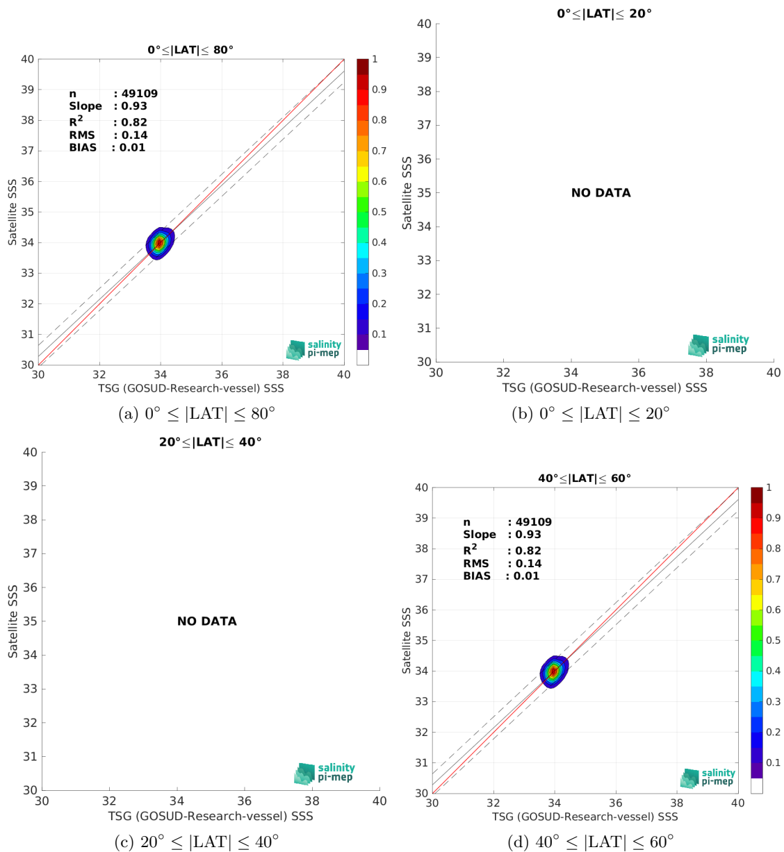
Figure 9: Contour maps of the concentration of CCI SSS L4 Merged-OI v4.4 - 7-day running (ESA) SSS (y-axis) versus TSG (GOSUD-Research-vessel) SSS (x-axis) at match-up pairs for different latitude bands. For each plot, the red line shows x=y . The black thin and dashed lines indicate a linear fit through the data cloud and the \pm 95\% confidence levels, respectively. The number match-up pairs n , the slope and R^2 coefficient of the linear fit, the root mean square (RMS) and the mean bias between satellite and in situ data are indicated for each latitude band in each plots.
