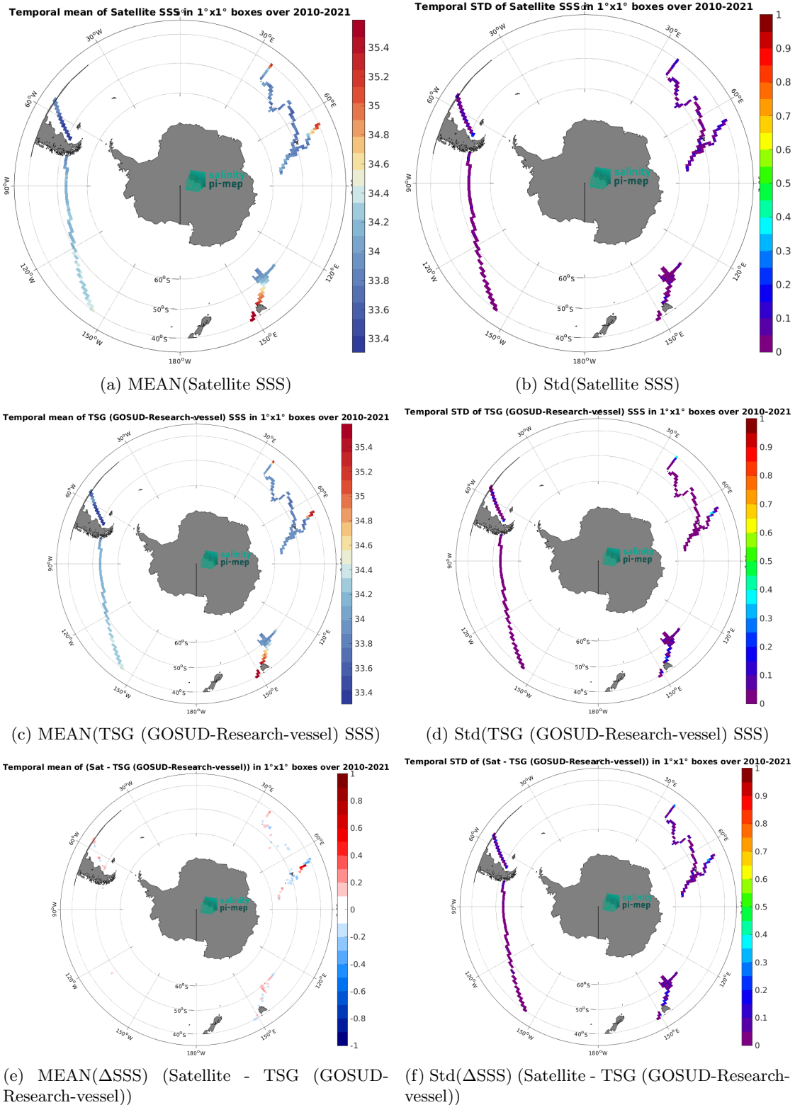
Figure 6: Temporal mean (left) and Std (right) of SSS from CCI SSS L4 Merged-OI v4.4 - 7-day running (ESA) (top), TSG (GOSUD-Research-vessel) (middle), and of \Delta SSS (Satellite - TSG (GOSUD-Research-vessel)). Only match-up pairs are used to generate these maps.
