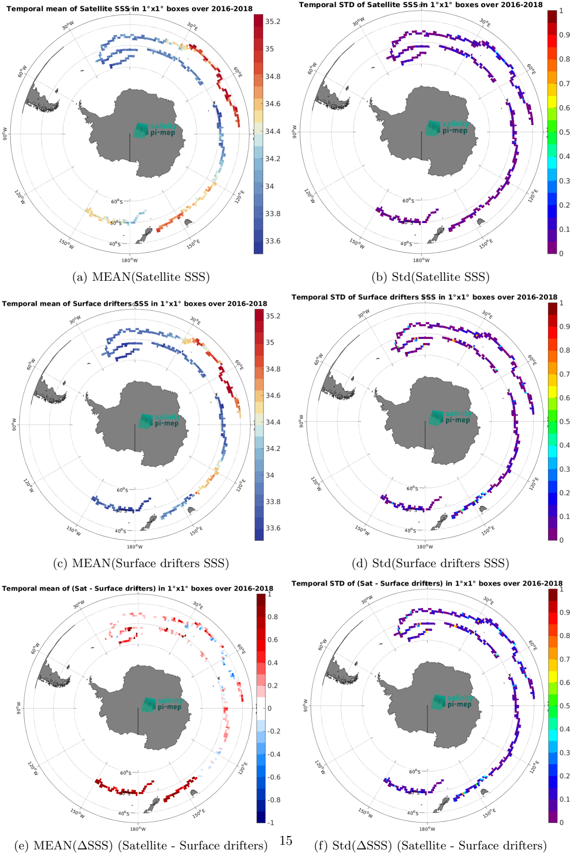
Figure 5: Temporal mean (left) and Std (right) of SSS from CCI SSS L4 Merged-OI v4.4 - 7-day running (ESA) (top), Surface drifters (middle), and of \Delta SSS (Satellite - Surface drifters). Only match-up pairs are used to generate these maps.
