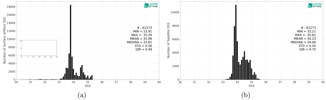
Figure 2: Histograms of SSS from Surface drifters (a) and CCI SSS L4 Merged-OI v4.4 - 7-day running (ESA) (b) considering all match-up pairs per bins of 0.1 over the Roaring Forties and Furious Fifties Pi-MEP region and for the full satellite product period.
