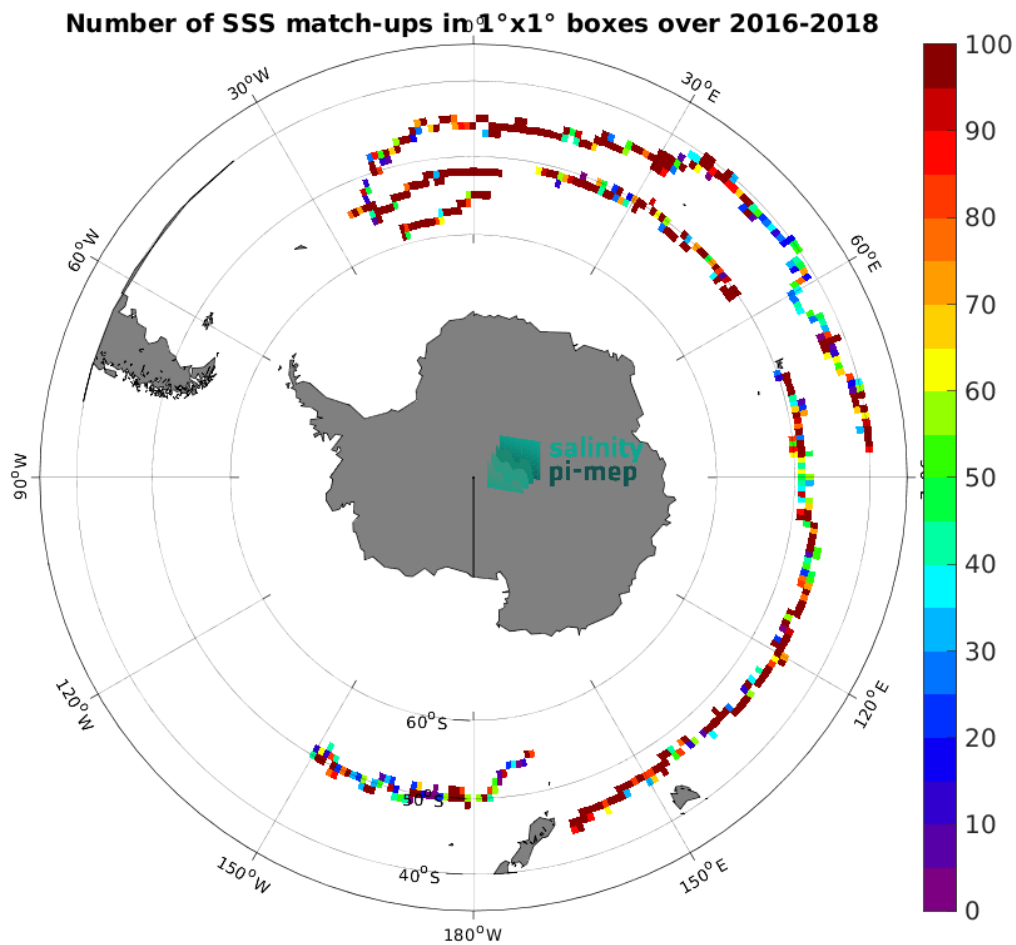
Figure 3: Number of SSS match-ups between Surface drifters SSS and the CCI SSS L4 Merged-OI v4.4 - 7-day running (ESA) SSS product for the Roaring Forties and Furious Fifties Pi-MEP region over 1^\circ \times 1^\circ boxes and for the full satellite product period.
