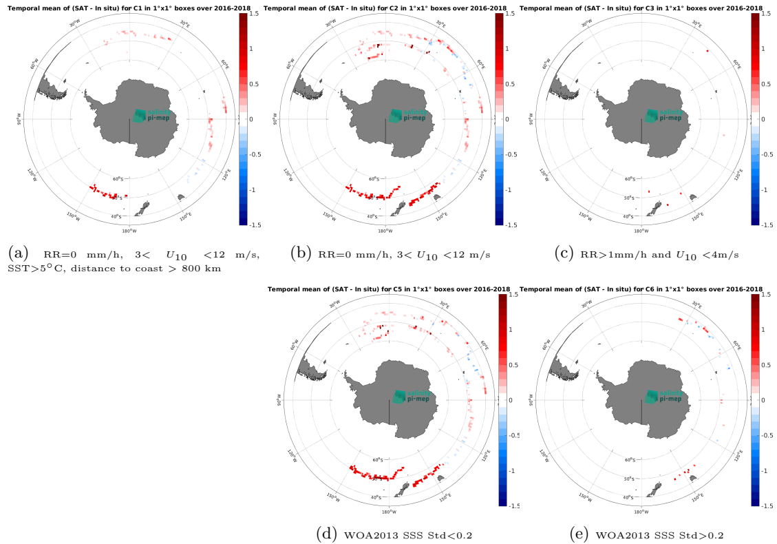
Figure 11: Temporal mean gridded over spatial boxes of size 1^{\circ}\times 1^{\circ} of \Delta\text{SSS} (CCI SSS L4 Merged-OI v4.4 - 7-day running (ESA) - Surface drifters) for 5 different subdatasets corresponding to:RR=0 mm/h, 3 < U_{10} < 12 m/s, SST >5^{\circ}\text{C} , distance to coast > 800 km (a), RR=0 mm/h, 3 < U_{10} < 12 m/s (b), RR >1 mm/h and U_{10} < 4 m/s (c), WOA2013 SSS Std <0.2 (d), WOA2013 SSS Std >0.2 (e).
