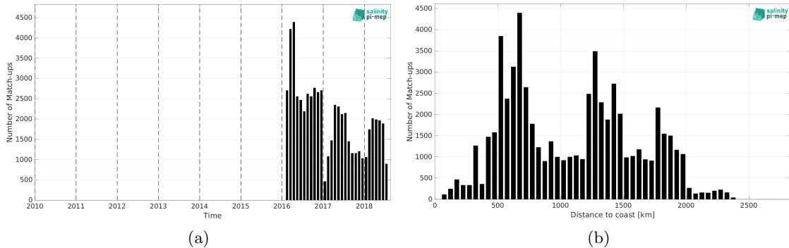
Figure 1: Number of match-ups between Surface drifters and CCI SSS L4 Merged-OI v4.4 - 7-day running (ESA) SSS as a function of time (a) and as function of the distance to coast (b) over the Roaring Forties and Furious Fifties Pi-MEP region and for the full satellite product period.
