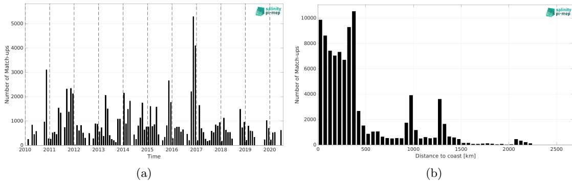
Figure 1: Number of match-ups between TSG (SAMOS) and CCI SSS L4 Merged-OI v3.2 - 7-day running (ESA) SSS as a function of time (a) and as function of the distance to coast (b) over the Roaring Forties and Furious Fifties Pi-MEP region and for the full satellite product period.
