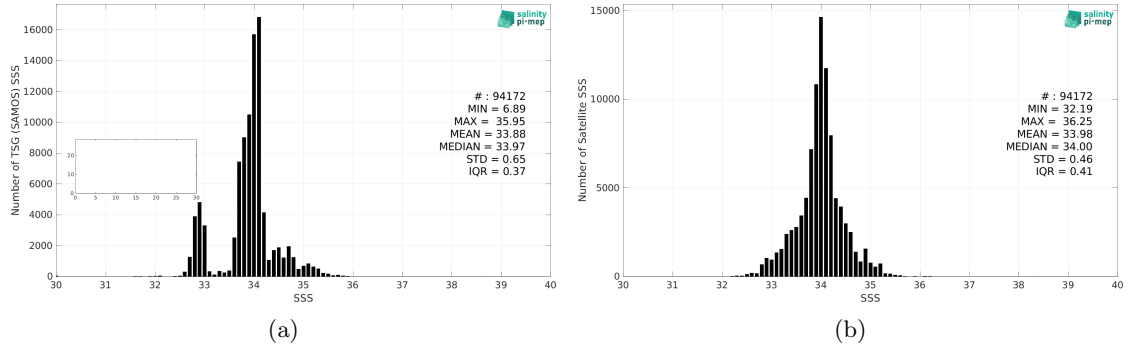
Figure 2: Histograms of SSS from TSG (SAMOS) (a) and CCI SSS L4 Merged-OI v3.2 - 7-day running (ESA) (b) considering all match-up pairs per bins of 0.1 over the Roaring Forties and Furious Fifties Pi-MEP region and for the full satellite product period.
