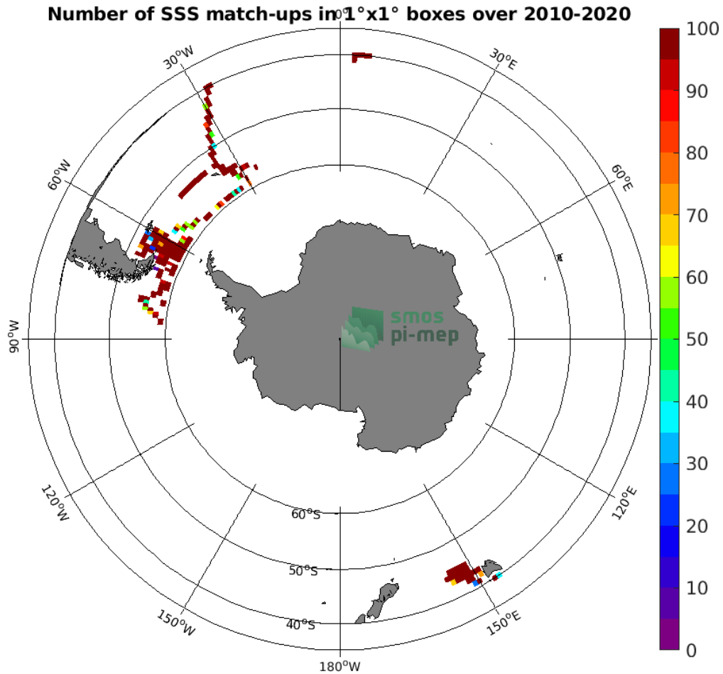
Figure 4: Number of SSS match-ups between TSG (SAMOS) SSS and the CCI SSS L4 Merged-OI v3.2 - 7-day running (ESA) SSS product for the Roaring Forties and Furious Fifties Pi-MEP region over 1^\circ \times 1^\circ boxes and for the full satellite product period.
