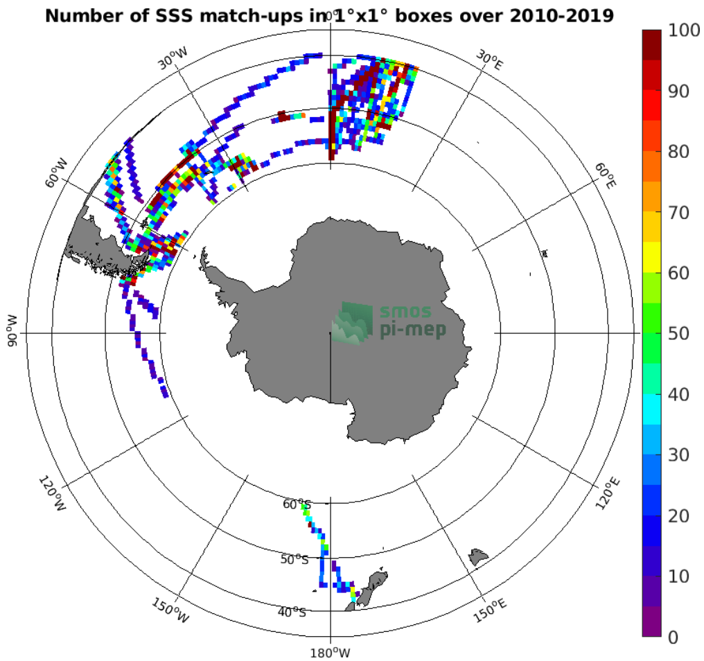
Figure 4: Number of SSS match-ups between TSG (Polarstern) SSS and the CCI SSS L4 Merged-OI v3.2 - 7-day running (ESA) SSS product for the Roaring Forties and Furious Fifties Pi-MEP region over 1^\circ \times 1^\circ boxes and for the full satellite product period.
