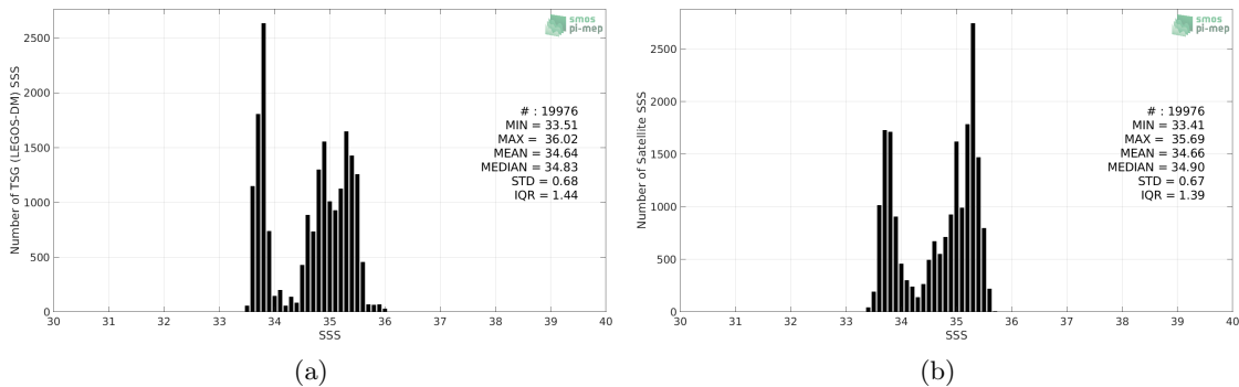
Figure 2: Histograms of SSS from TSG (LEGOS-DM) (a) and CCI SSS L4 Merged-OI v3.2 - 7-day running (ESA) (b) considering all match-up pairs per bins of 0.1 over the Roaring Forties and Furious Fifties Pi-MEP region and for the full satellite product period.
