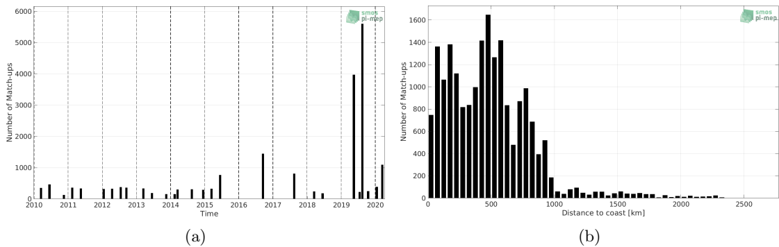
Figure 1: Number of match-ups between TSG (LEGOS-DM) and CCI SSS L4 Merged-OI v3.2 - 7-day running (ESA) SSS as a function of time (a) and as function of the distance to coast (b) over the Roaring Forties and Furious Fifties Pi-MEP region and for the full satellite product period.
