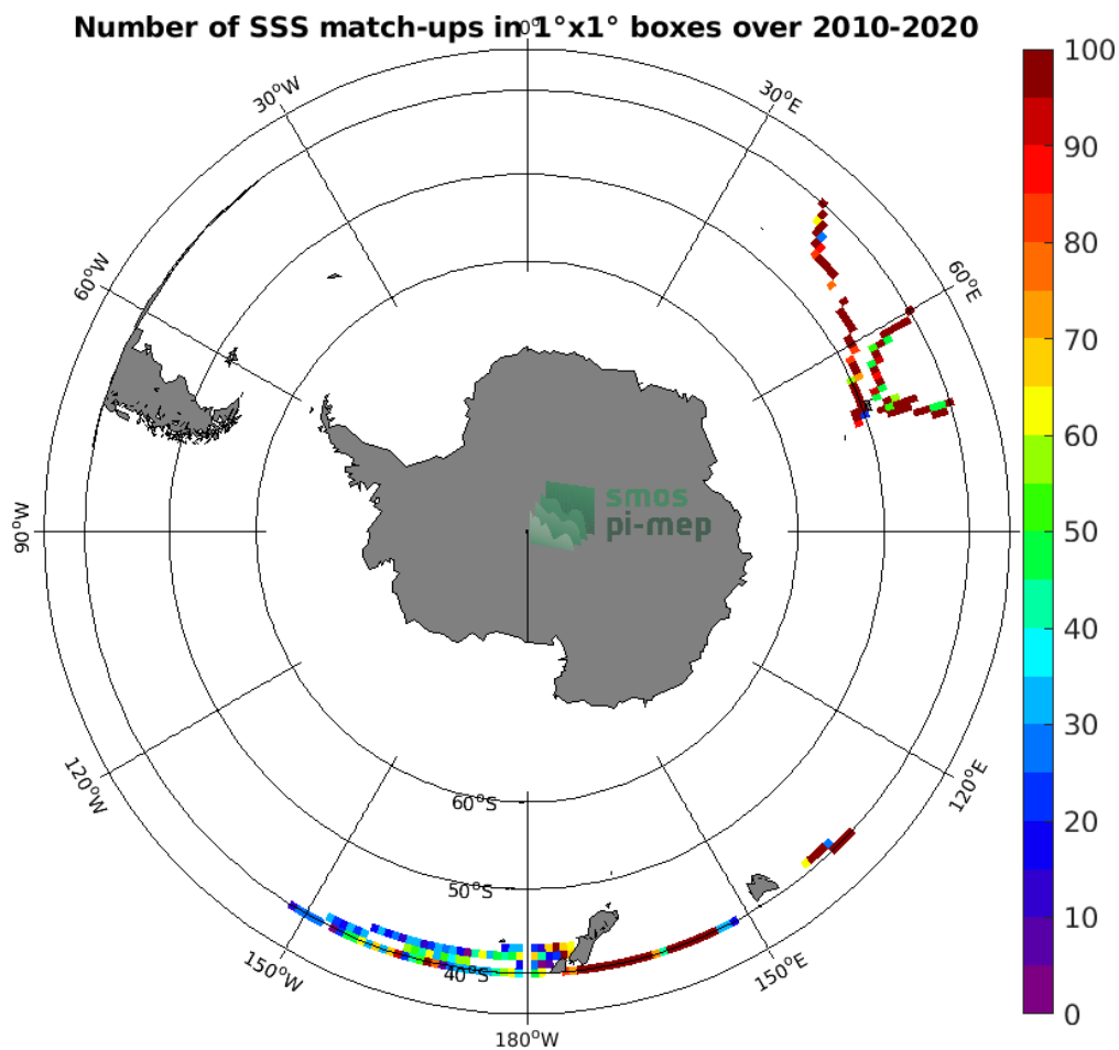
Figure 4: Number of SSS match-ups between TSG (LEGOS-DM) SSS and the CCI SSS L4 Merged-OI v3.2 - 7-day running (ESA) SSS product for the Roaring Forties and Furious Fifties Pi-MEP region over 1^\circ \times 1^\circ boxes and for the full satellite product period.
