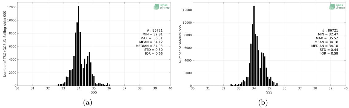
Figure 2: Histograms of SSS from TSG (GOSUD-Sailing-ship) (a) and CCI SSS L4 Merged-OI v3.2 - 7-day running (ESA) (b) considering all match-up pairs per bins of 0.1 over the Roaring Forties and Furious Fifties Pi-MEP region and for the full satellite product period.
