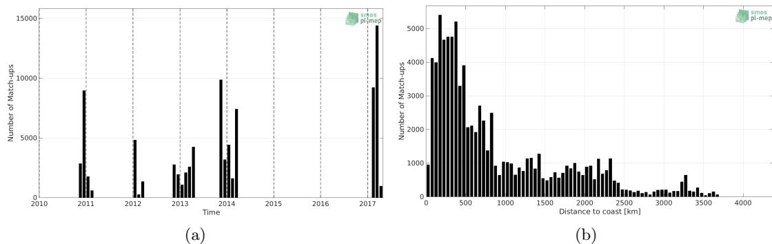
Figure 1: Number of match-ups between TSG (GOSUD-Sailing-ship) and CCI SSS L4 Merged-OI v3.2 - 7-day running (ESA) SSS as a function of time (a) and as function of the distance to coast (b) over the Roaring Forties and Furious Fifties Pi-MEP region and for the full satellite product period.
