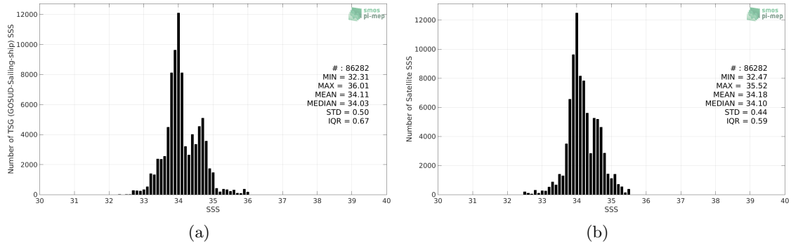
Figure 2: Histograms of SSS from TSG (GOSUD-Sailing-ship) (a) and CCI SSS L4 Merged-OI v3.2 - 7-day running (ESA) (b) considering all match-up pairs per bins of 0.1 over the Roaring Forties and Furious Fifties Pi-MEP region and for the full satellite product period.
