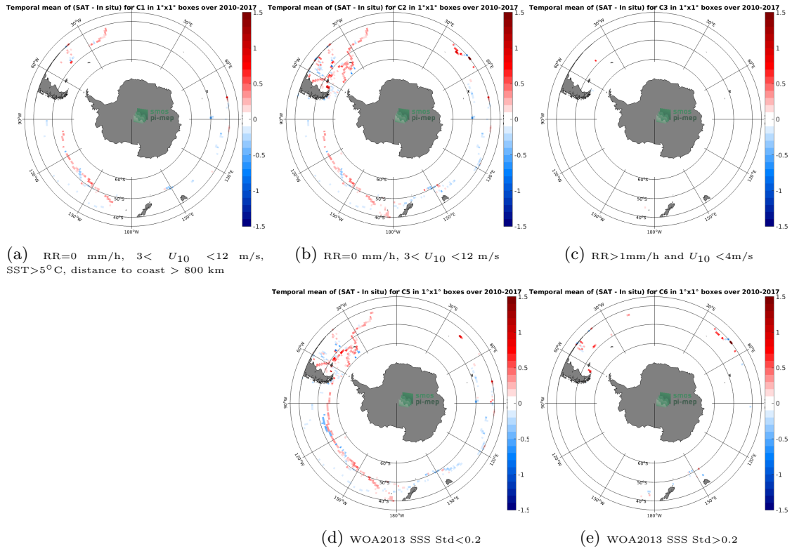
Figure 12: Temporal mean gridded over spatial boxes of size 1^\circ \times 1^\circ of \Delta SSS (CCI SSS L4 Merged-OI v3.2 - 7-day running (ESA) - TSG (GOSUD-Sailing-ship)) for 5 different subdatasets corresponding to:RR=0 mm/h, 3 < U_{10} < 12 m/s, SST>5°C, distance to coast > 800 km (a), RR=0 mm/h, 3 < U_{10} < 12 m/s (b), RR>1mm/h and U_{10} < 4 m/s (c), WOA2013 SSS Std<0.2 (d), WOA2013 SSS Std>0.2 (e).
