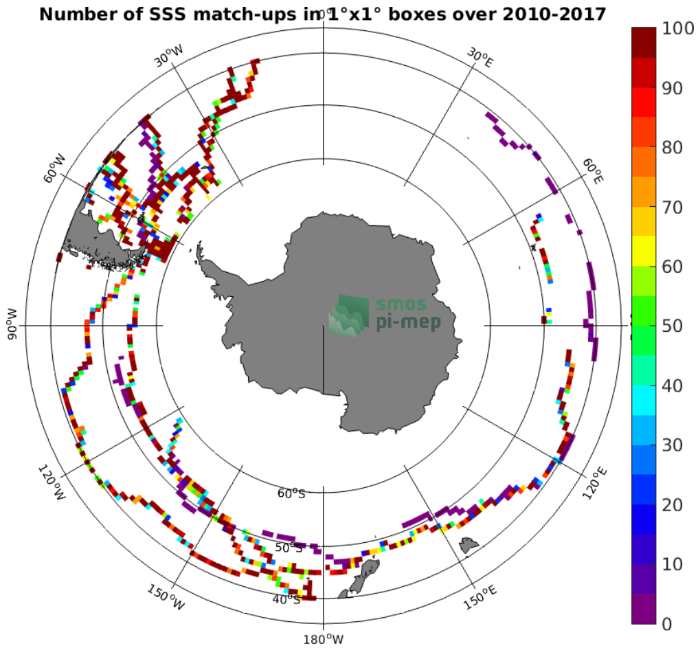
Figure 4: Number of SSS match-ups between TSG (GOSUD-Sailing-ship) SSS and the CCI SSS L4 Merged-OI v3.2 - 7-day running (ESA) SSS product for the Roaring Forties and Furious Fifties Pi-MEP region over 1^\circ \times 1^\circ boxes and for the full satellite product period.
