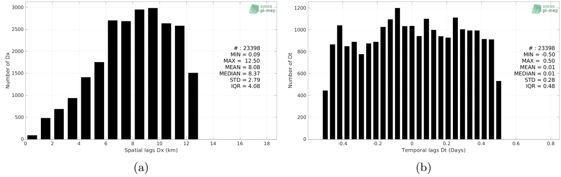
Figure 5: Histograms of the spatial (a) and temporal (b) lags between the location/time of the TSG (GOSUD-Research-vessel) measurement and the date of the corresponding CCI SSS L4 Merged-OI v3.2 - 7-day running (ESA) SSS pixel.
