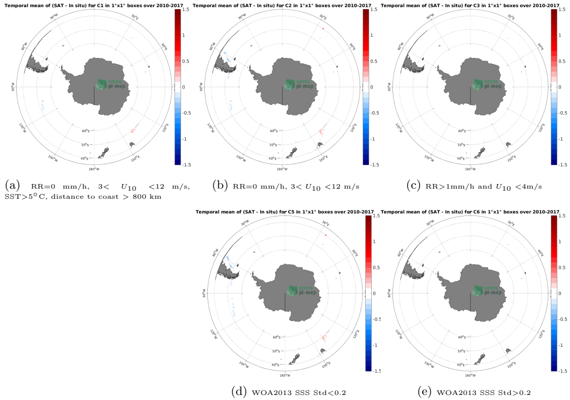
Figure 12: Temporal mean gridded over spatial boxes of size 1^\circ \times 1^\circ of \Delta SSS (CCI SSS L4 Merged-OI v3.2 - 7-day running (ESA) - TSG (GOSUD-Research-vessel)) for 5 different subdatasets corresponding to:RR=0 mm/h, 3 < U_{10} < 12 m/s, SST>5°C, distance to coast > 800 km (a), RR=0 mm/h, 3 < U_{10} < 12 m/s (b), RR>1mm/h and U_{10} < 4 m/s (c), WOA2013 SSS Std<0.2 (d), WOA2013 SSS Std>0.2 (e).
