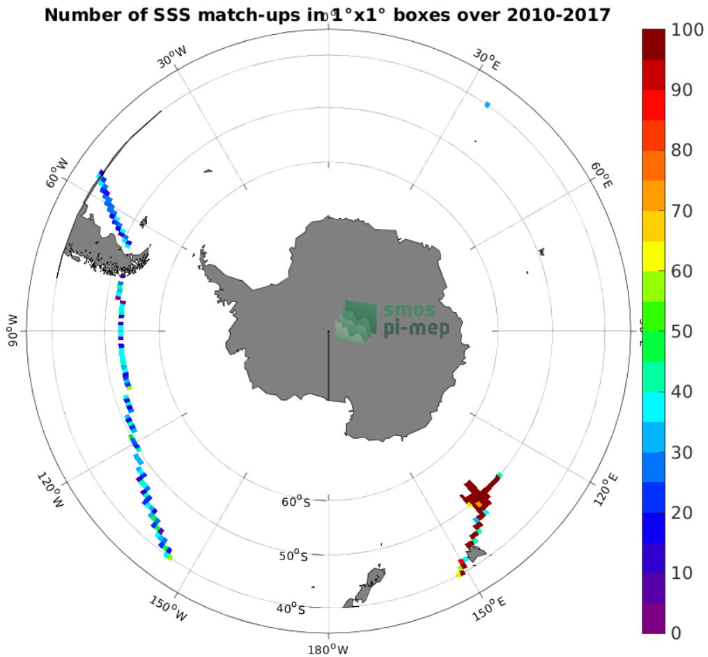
Figure 4: Number of SSS match-ups between TSG (GOSUD-Research-vessel) SSS and the CCI SSS L4 Merged-OI v3.2 - 7-day running (ESA) SSS product for the Roaring Forties and Furious Fifties Pi-MEP region over 1^\circ \times 1^\circ boxes and for the full satellite product period.
