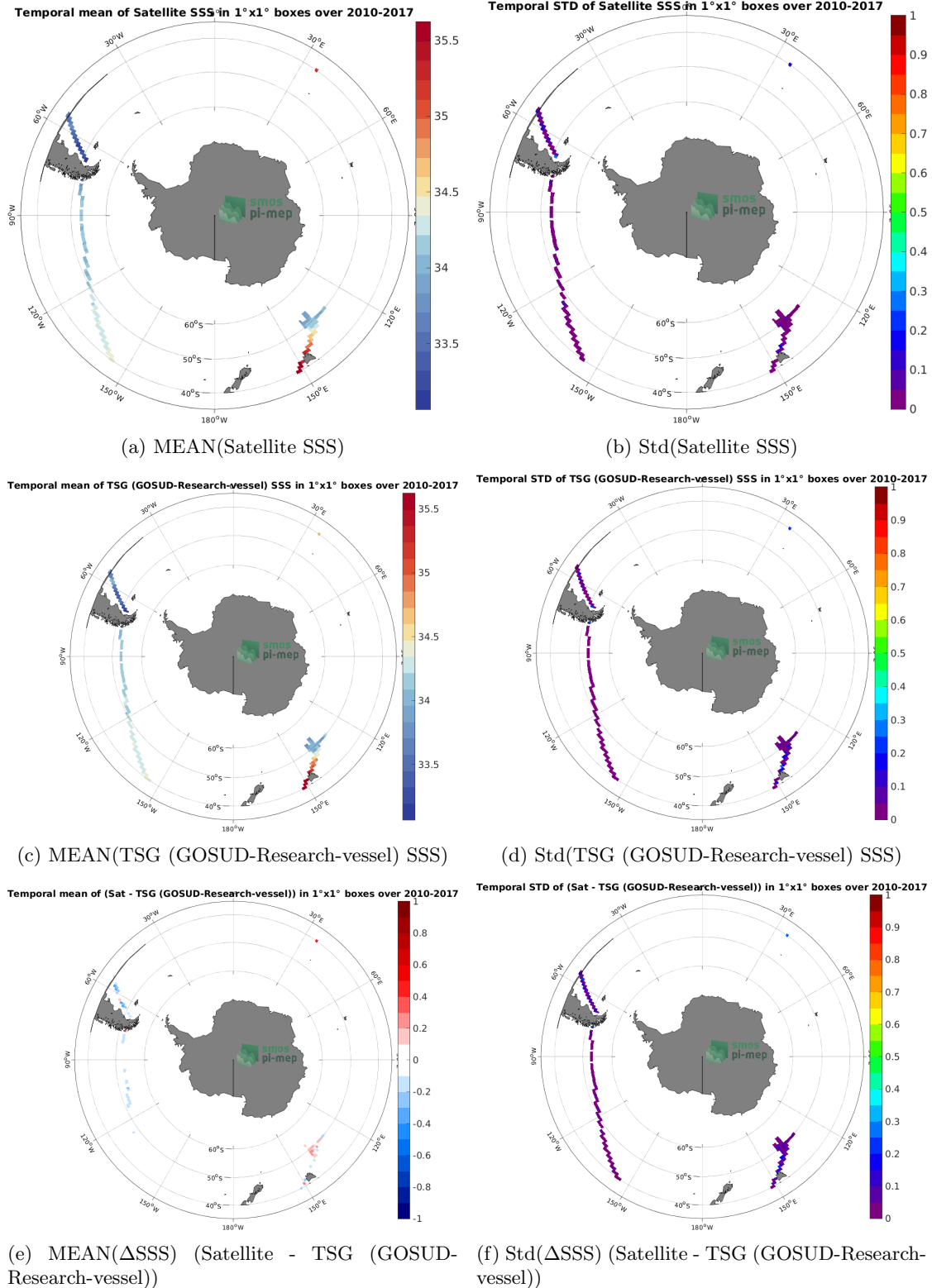
Figure 6: Temporal mean (left) and Std (right) of SSS from CCI SSS L4 Merged-OI v3.2 - 7-day running (ESA) (top), TSG (GOSUD-Research-vessel) (middle), and of \Delta SSS (Satellite - TSG (GOSUD-Research-vessel)). Only match-up pairs are used to generate these maps.
