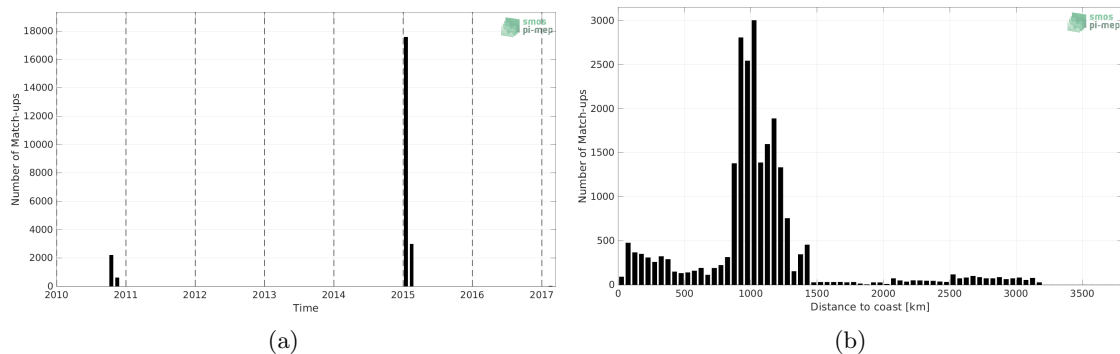
Figure 1: Number of match-ups between TSG (GOSUD-Research-vessel) and CCI SSS L4 Merged-OI v3.2 - 7-day running (ESA) SSS as a function of time (a) and as function of the distance to coast (b) over the Roaring Forties and Furious Fifties Pi-MEP region and for the full satellite product period.
