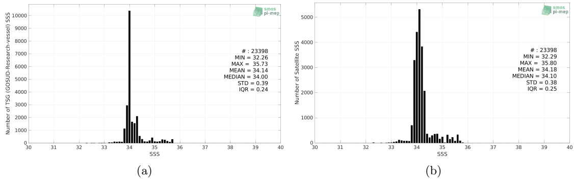
Figure 2: Histograms of SSS from TSG (GOSUD-Research-vessel) (a) and CCI SSS L4 Merged-OI v3.2 - 7-day running (ESA) (b) considering all match-up pairs per bins of 0.1 over the Roaring Forties and Furious Fifties Pi-MEP region and for the full satellite product period.
