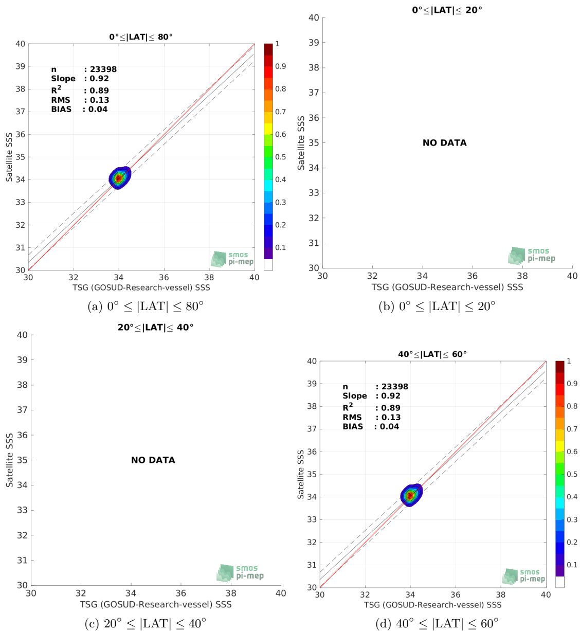
Figure 9: Contour maps of the concentration of CCI SSS L4 Merged-OI v3.2 - 7-day running (ESA) SSS (y-axis) versus TSG (GOSUD-Research-vessel) SSS (x-axis) at match-up pairs for different latitude bands. For each plot, the red line shows x=y . The black thin and dashed lines indicate a linear fit through the data cloud and the \pm 95\% confidence levels, respectively. The number match-up pairs n , the slope and R^2 coefficient of the linear fit, the root mean square (RMS) and the mean bias between satellite and in situ data are indicated for each latitude band in each plots.
