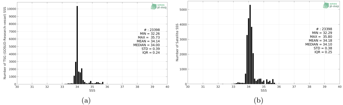
Figure 2: Histograms of SSS from TSG (GOSUD-Research-vessel) (a) and CCI SSS L4 Merged-OI v3.2 - 7-day running (ESA) (b) considering all match-up pairs per bins of 0.1 over the Roaring Forties and Furious Fifties Pi-MEP region and for the full satellite product period.
