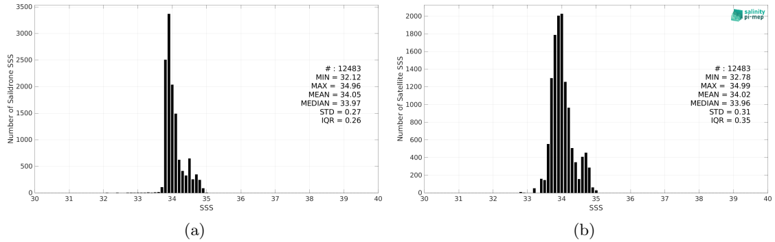
Figure 2: Histograms of SSS from Saildrone (a) and CCI SSS L4 Merged-OI v3.2 - 7-day running (ESA) (b) considering all match-up pairs per bins of 0.1 over the Roaring Forties and Furious Fifties Pi-MEP region and for the full satellite product period.
