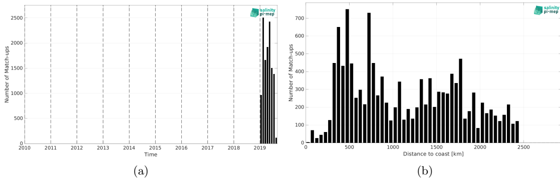
Figure 1: Number of match-ups between Saildrone and CCI SSS L4 Merged-OI v3.2 - 7-day running (ESA) SSS as a function of time (a) and as function of the distance to coast (b) over the Roaring Forties and Furious Fifties Pi-MEP region and for the full satellite product period.
