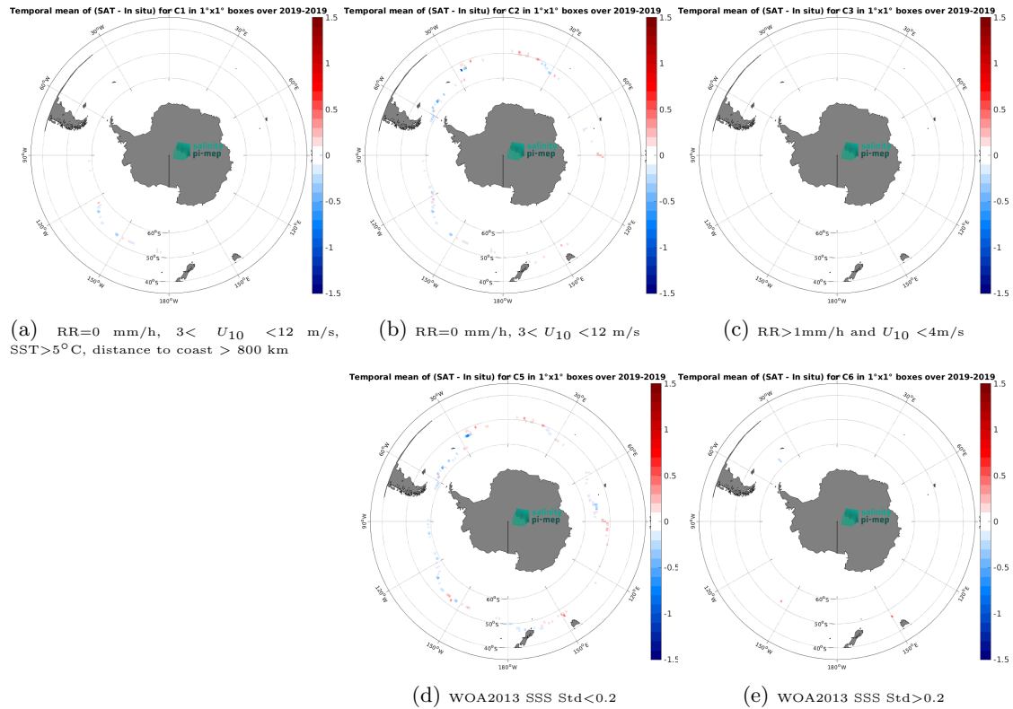
Figure 12: Temporal mean gridded over spatial boxes of size 1^{\circ}\times 1^{\circ} of \Delta\text{SSS} (CCI SSS L4 Merged-OI v3.2 - 7-day running (ESA) - Saildrone) for 5 different subdatasets corresponding to:RR=0 mm/h, 3 < U_{10} < 12 m/s, SST >5^{\circ}\text{C} , distance to coast > 800 km (a), RR=0 mm/h, 3 < U_{10} < 12 m/s (b), RR >1 mm/h and U_{10} < 4 m/s (c), WOA2013 SSS Std <0.2 (d), WOA2013 SSS Std >0.2 (e).
