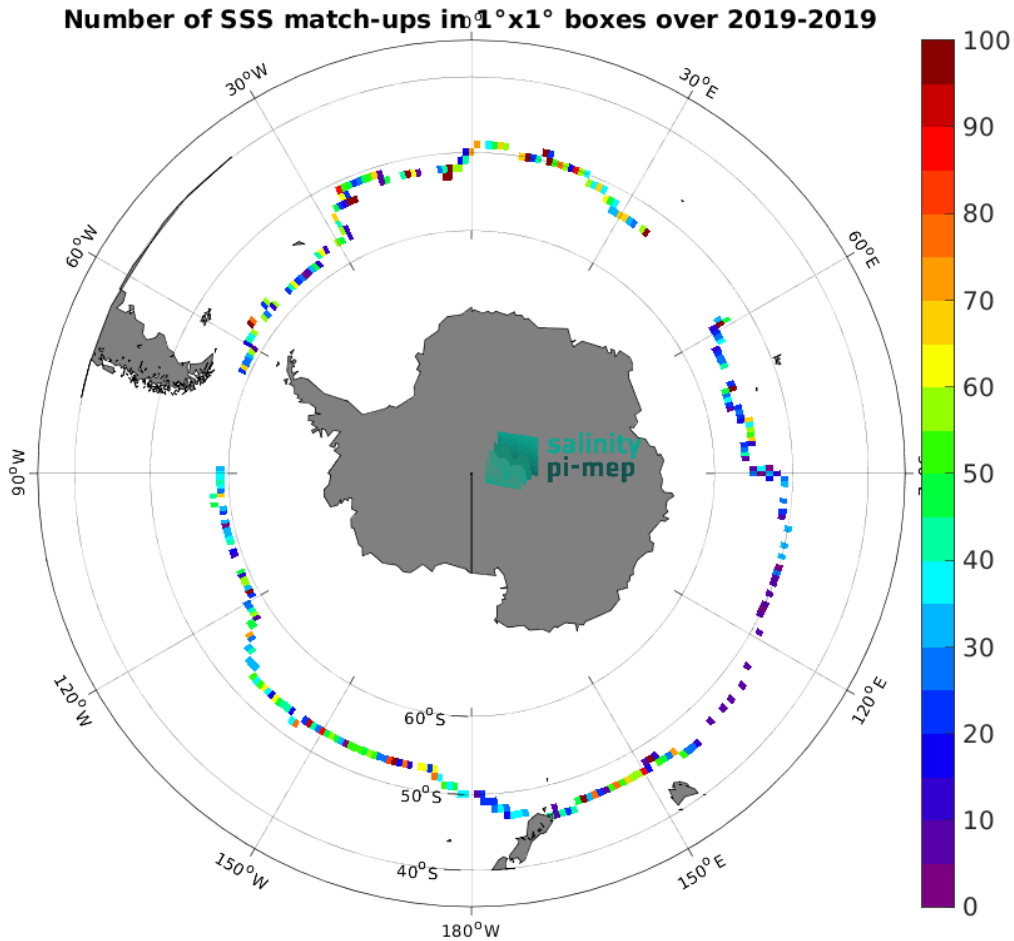
Figure 4: Number of SSS match-ups between Saildrone SSS and the CCI SSS L4 Merged-OI v3.2 - 7-day running (ESA) SSS product for the Roaring Forties and Furious Fifties Pi-MEP region over 1^\circ \times 1^\circ boxes and for the full satellite product period.
