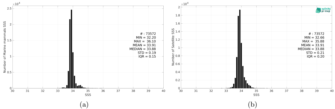
Figure 2: Histograms of SSS from Marine mammals (a) and CCI SSS L4 Merged-OI v3.2 - 7-day running (ESA) (b) considering all match-up pairs per bins of 0.1 over the Roaring Forties and Furious Fifties Pi-MEP region and for the full satellite product period.
