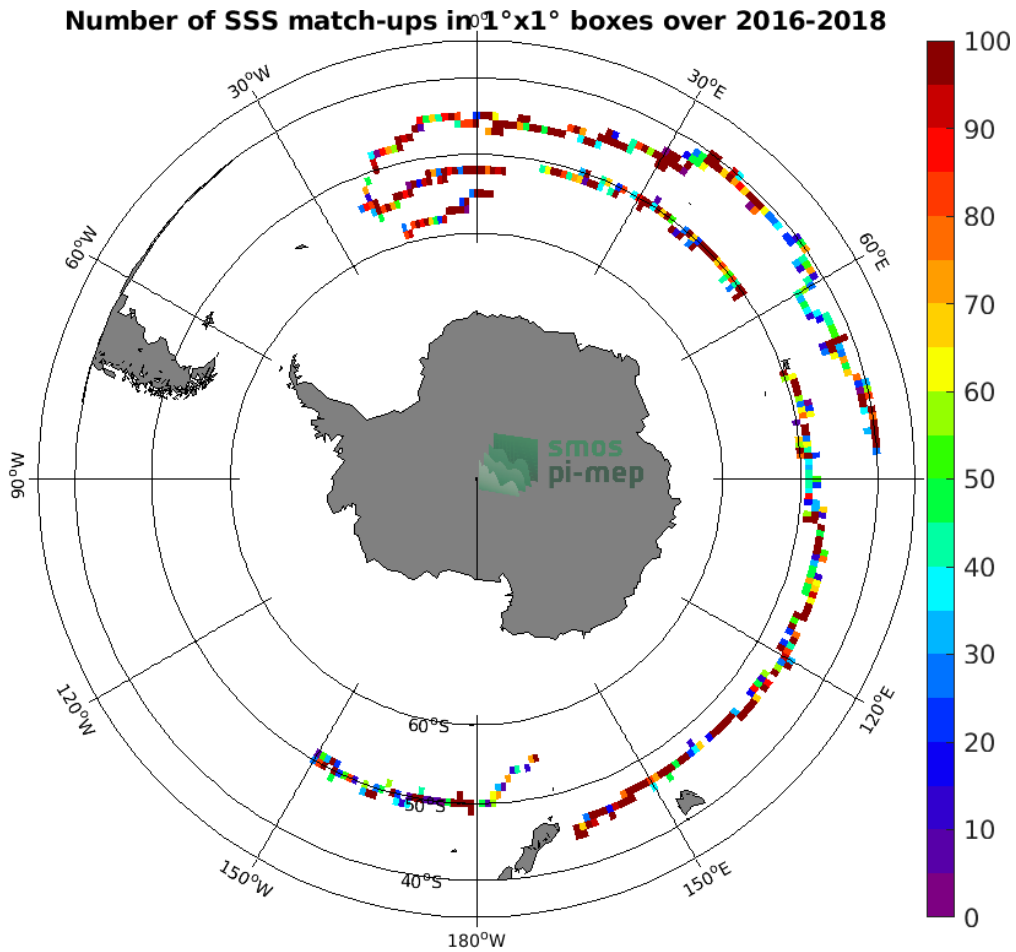
Figure 3: Number of SSS match-ups between Surface drifters SSS and the CCI SSS L4 Merged-OI v3.2 - 7-day running (ESA) SSS product for the Roaring Forties and Furious Fifties Pi-MEP region over 1^\circ \times 1^\circ boxes and for the full satellite product period.
