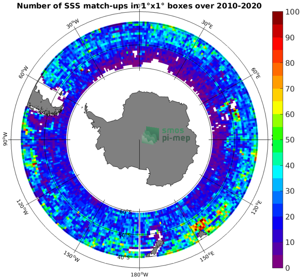
Figure 4: Number of SSS match-ups between Argo SSS and the CCI SSS L4 Merged-OI v3.2 - 7-day running (ESA) SSS product for the Roaring Forties and Furious Fifties Pi-MEP region over 1^\circ \times 1^\circ boxes and for the full satellite product period.
