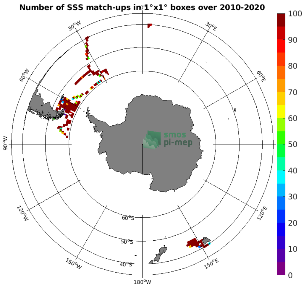
Figure 4: Number of SSS match-ups between TSG (SAMOS) SSS and the CCI SSS L4 Merged-OI v3.2 - 30-day running (ESA) SSS product for the Roaring Forties and Furious Fifties Pi-MEP region over 1^\circ \times 1^\circ boxes and for the full satellite product period.
