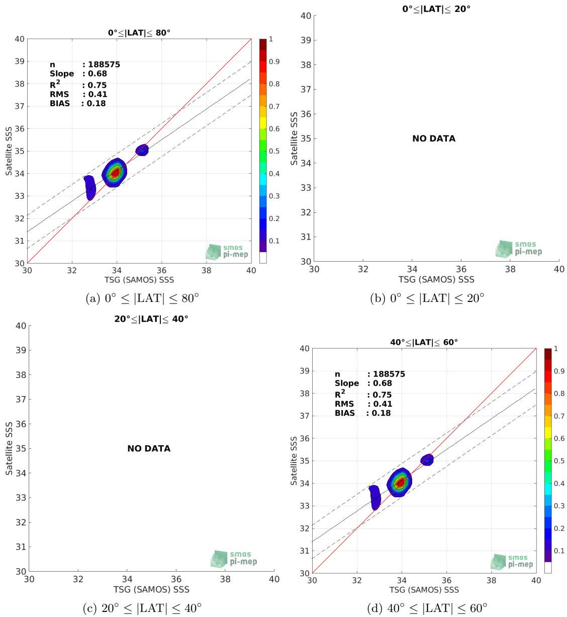
Figure 9: Contour maps of the concentration of CCI SSS L4 Merged-OI v3.2 - 30-day running (ESA) SSS (y-axis) versus TSG (SAMOS) SSS (x-axis) at match-up pairs for different latitude bands. For each plot, the red line shows x=y . The black thin and dashed lines indicate a linear fit through the data cloud and the \pm 95\% confidence levels, respectively. The number match-up pairs n , the slope and R^2 coefficient of the linear fit, the root mean square (RMS) and the mean bias between satellite and in situ data are indicated for each latitude band in each plots.
