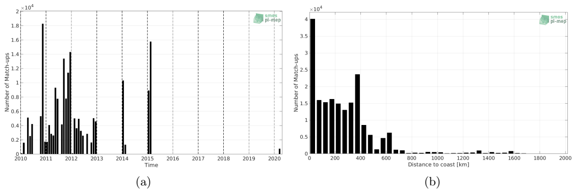
Figure 1: Number of match-ups between TSG (SAMOS) and CCI SSS L4 Merged-OI v3.2 - 30-day running (ESA) SSS as a function of time (a) and as function of the distance to coast (b) over the Roaring Forties and Furious Fifties Pi-MEP region and for the full satellite product period.
