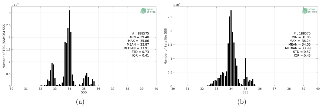
Figure 2: Histograms of SSS from TSG (SAMOS) (a) and CCI SSS L4 Merged-OI v3.2 - 30-day running (ESA) (b) considering all match-up pairs per bins of 0.1 over the Roaring Forties and Furious Fifties Pi-MEP region and for the full satellite product period.
