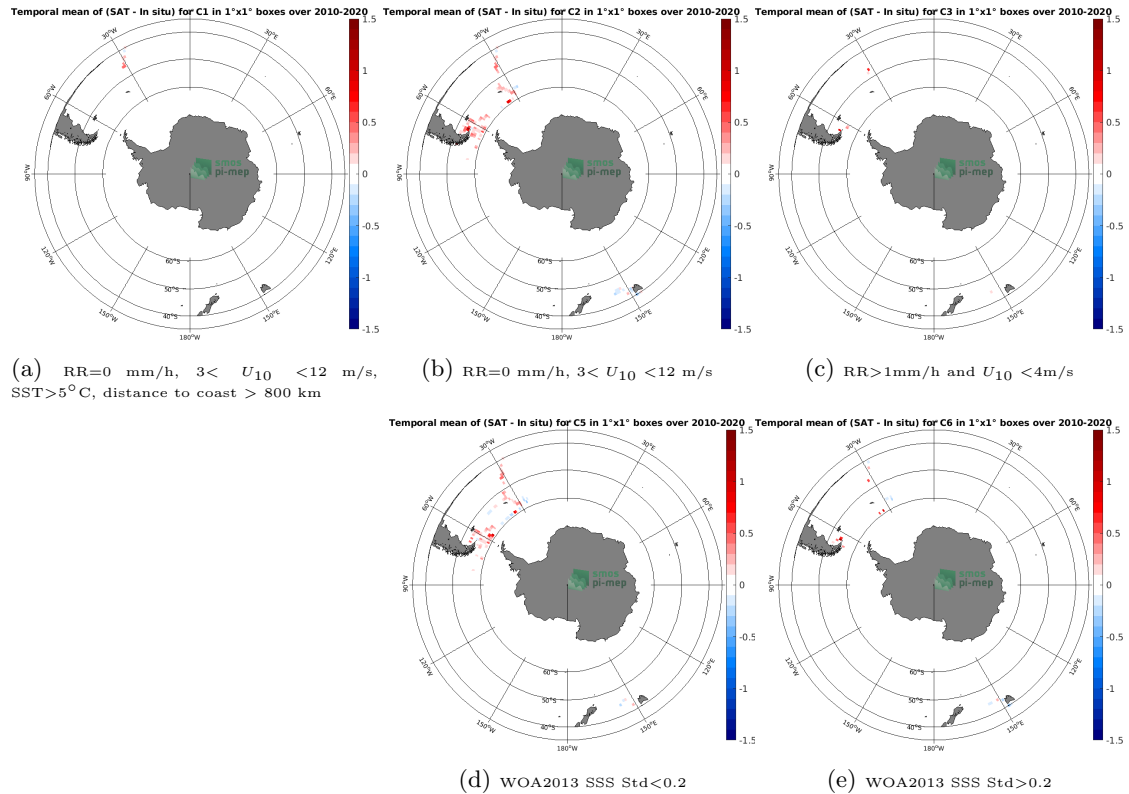
Figure 12: Temporal mean gridded over spatial boxes of size 1^{\circ}\times 1^{\circ} of \Delta\text{SSS} (CCI SSS L4 Merged-OI v3.2 - 30-day running (ESA) - TSG (SAMOS)) for 5 different subdatasets corresponding to:RR=0 mm/h, 3 < U_{10} < 12 m/s, SST >5^{\circ}\text{C} , distance to coast > 800 km (a), RR=0 mm/h, 3 < U_{10} < 12 m/s (b), RR >1 mm/h and U_{10} < 4 m/s (c), WOA2013 SSS Std <0.2 (d), WOA2013 SSS Std >0.2 (e).
