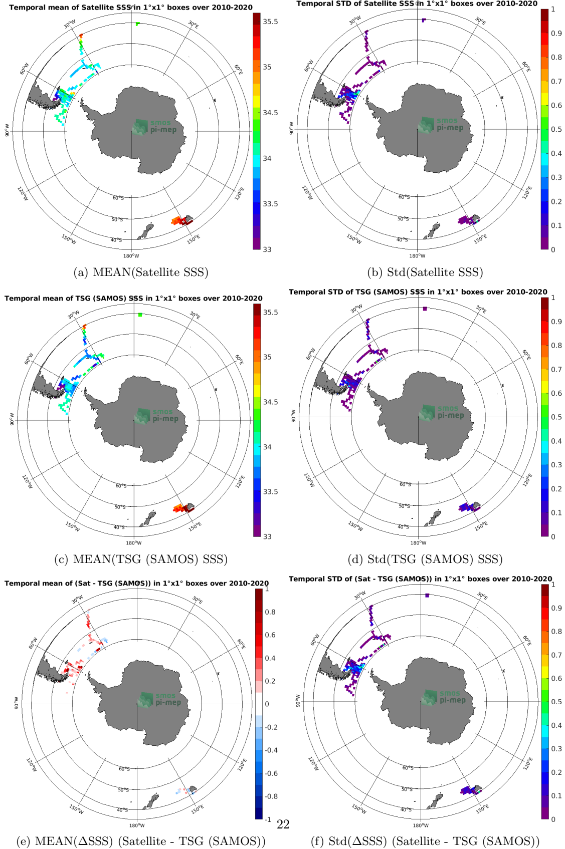
Figure 6: Temporal mean (left) and Std (right) of SSS from CCI SSS L4 Merged-OI v3.2 - 30-day running (ESA) (top), TSG (SAMOS) (middle), and of \Delta SSS (Satellite - TSG (SAMOS)). Only match-up pairs are used to generate these maps.
