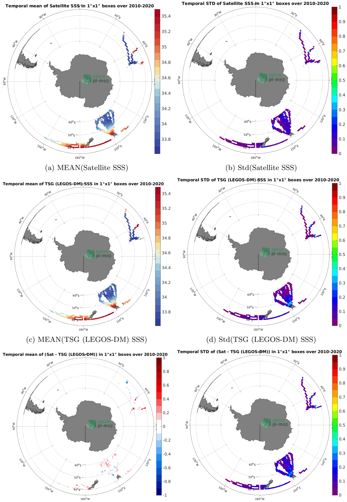
Figure 6: Temporal mean (left) and Std (right) of SSS from CCI SSS L4 Merged-OI v3.2 - 30-day running (ESA) (top), TSG (LEGOS-DM) (middle), and of \Delta SSS (Satellite - TSG (LEGOS-DM)). Only match-up pairs are used to generate these maps.
