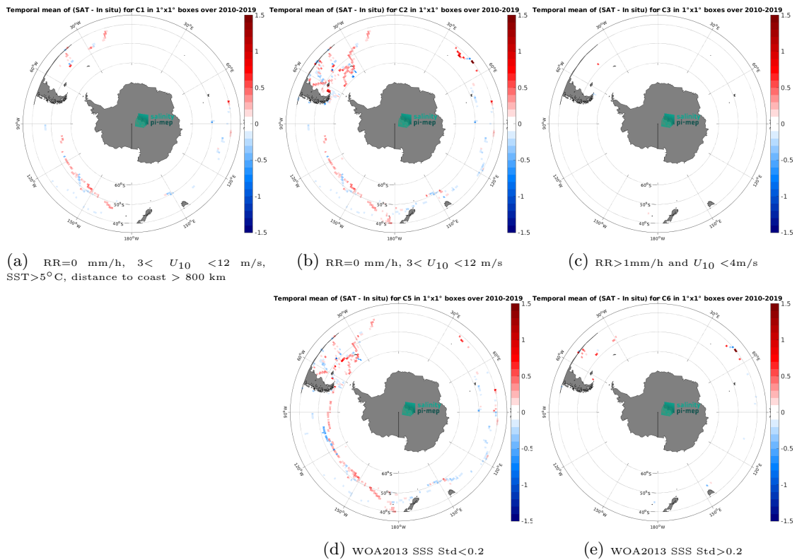
Figure 12: Temporal mean gridded over spatial boxes of size 1°×1° of \Delta SSS (CCI SSS L4 Merged-OI v3.2 - 30-day running (ESA) - TSG (GOSUD-Sailing-ship)) for 5 different subdatasets corresponding to:RR=0 mm/h, 3 < U_{10} < 12 m/s, SST>5°C, distance to coast > 800 km (a), RR=0 mm/h, 3 < U_{10} < 12 m/s (b), RR>1mm/h and U_{10} < 4 m/s (c), WOA2013 SSS Std<0.2 (d), WOA2013 SSS Std>0.2 (e).
