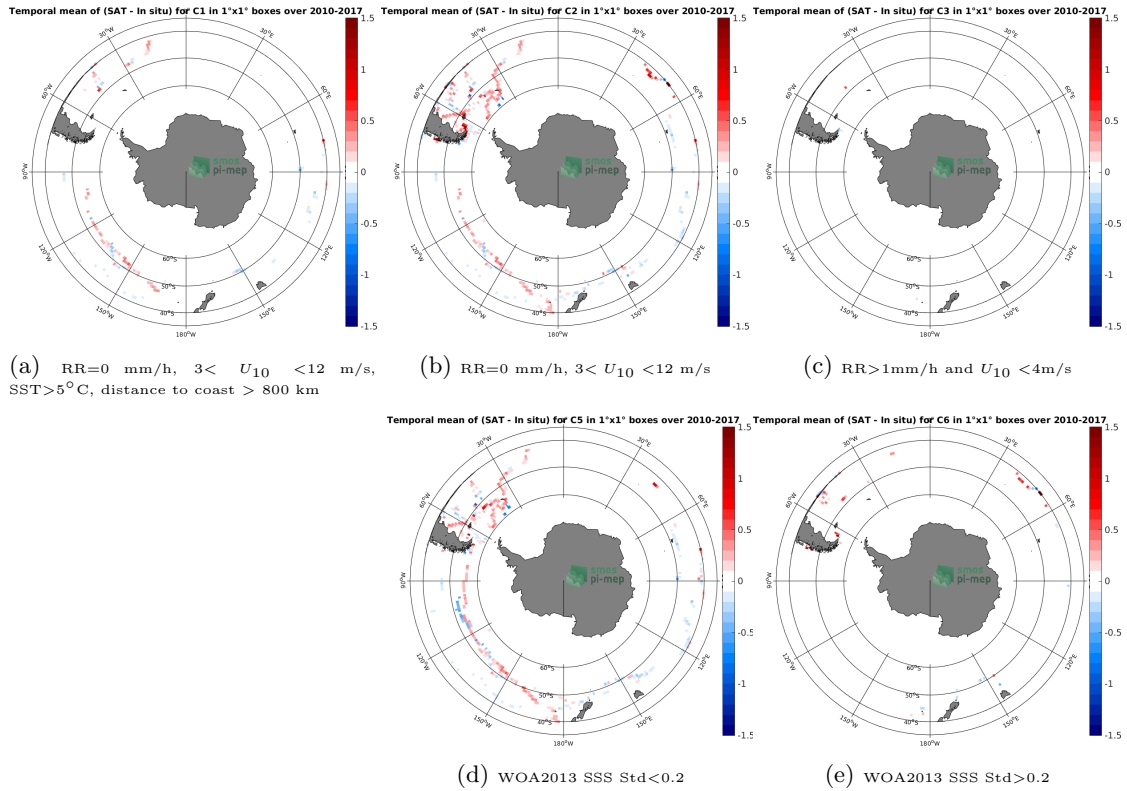
Figure 12: Temporal mean gridded over spatial boxes of size 1°x1° of \Delta SSS (CCI SSS L4 Merged-OI v3.2 - 30-day running (ESA) - TSG (GOSUD-Sailing-ship)) for 5 different subdatasets corresponding to:RR=0 mm/h, 3 < U_{10} < 12 m/s, SST>5°C, distance to coast > 800 km (a), RR=0 mm/h, 3 < U_{10} < 12 m/s (b), RR>1mm/h and U_{10} < 4 m/s (c), WOA2013 SSS Std<0.2 (d), WOA2013 SSS Std>0.2 (e).
