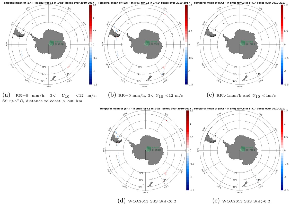
Figure 12: Temporal mean gridded over spatial boxes of size 1°x1° of \Delta SSS (CCI SSS L4 Merged-OI v3.2 - 30-day running (ESA) - TSG (GOSUD-Research-vessel)) for 5 different subdatasets corresponding to:RR=0 mm/h, 3 < U_{10} < 12 m/s, SST>5°C, distance to coast > 800 km (a), RR=0 mm/h, 3 < U_{10} < 12 m/s (b), RR>1mm/h and U_{10} < 4 m/s (c), WOA2013 SSS Std<0.2 (d), WOA2013 SSS Std>0.2 (e).
