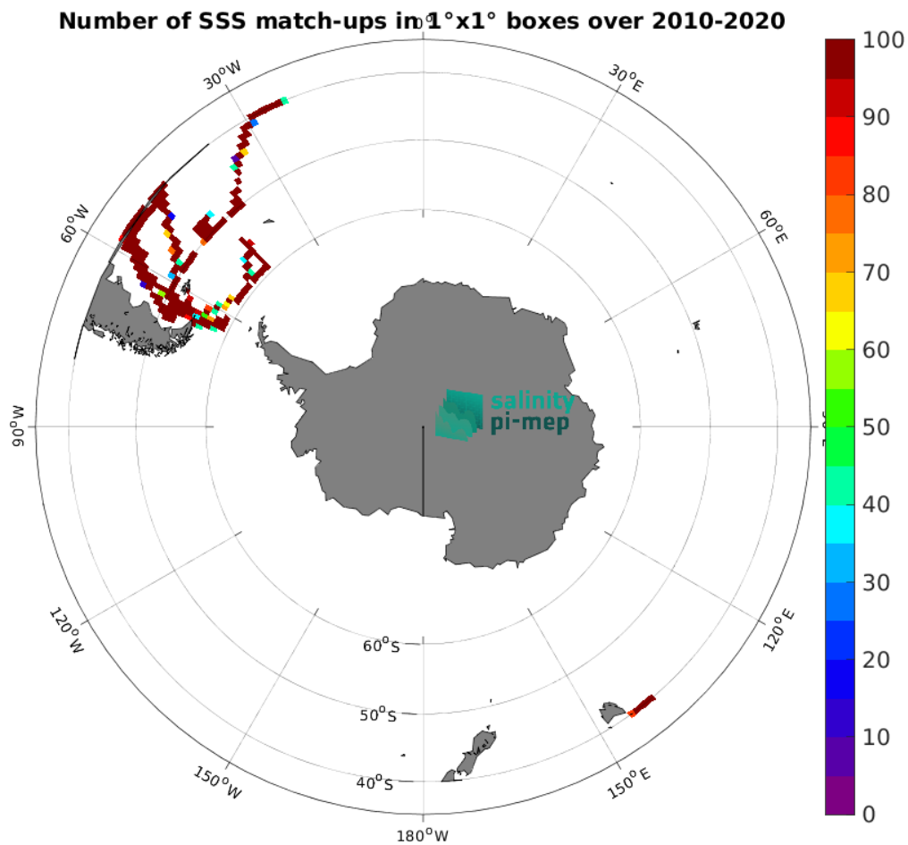
Figure 4: Number of SSS match-ups between TSG (CSIC-UTM) SSS and the CCI SSS L4 Merged-OI v3.2 - 30-day running (ESA) SSS product for the Roaring Forties and Furious Fifties Pi-MEP region over 1^\circ \times 1^\circ boxes and for the full satellite product period.
