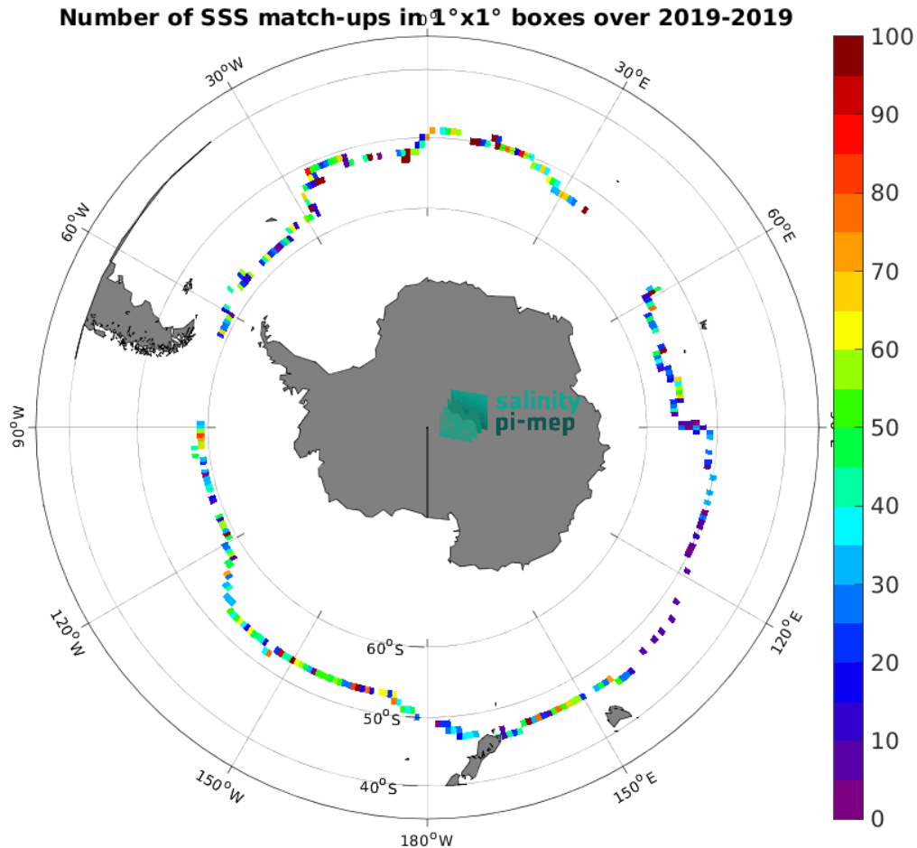
Figure 4: Number of SSS match-ups between Saildrone SSS and the CCI SSS L4 Merged-OI v3.2 - 30-day running (ESA) SSS product for the Roaring Forties and Furious Fifties Pi-MEP region over 1^\circ \times 1^\circ boxes and for the full satellite product period.
