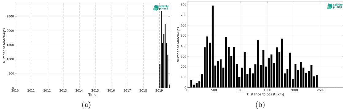
Figure 1: Number of match-ups between Saildrone and CCI SSS L4 Merged-OI v3.2 - 30-day running (ESA) SSS as a function of time (a) and as function of the distance to coast (b) over the Roaring Forties and Furious Fifties Pi-MEP region and for the full satellite product period.
