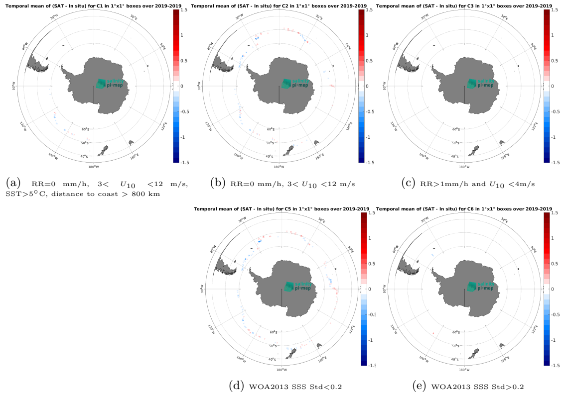
Figure 12: Temporal mean gridded over spatial boxes of size 1^{\circ}\times 1^{\circ} of \Delta\text{SSS} (CCI SSS L4 Merged-OI v3.2 - 30-day running (ESA) - Saildrone) for 5 different subdatasets corresponding to:RR=0 mm/h, 3 < U_{10} < 12 m/s, SST >5^{\circ}\text{C} , distance to coast > 800 km (a), RR=0 mm/h, 3 < U_{10} < 12 m/s (b), RR >1 mm/h and U_{10} < 4 m/s (c), WOA2013 SSS Std <0.2 (d), WOA2013 SSS Std >0.2 (e).
