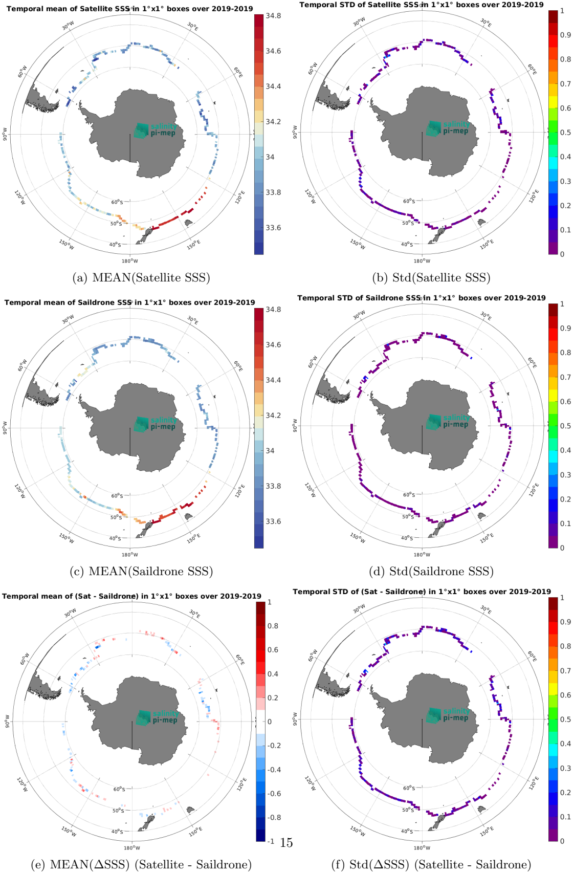
Figure 6: Temporal mean (left) and Std (right) of SSS from CCI SSS L4 Merged-OI v3.2 - 30-day running (ESA) (top), Saildrone (middle), and of \Delta SSS (Satellite - Saildrone). Only match-up pairs are used to generate these maps.
