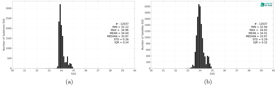
Figure 2: Histograms of SSS from Saildrone (a) and CCI SSS L4 Merged-OI v3.2 - 30-day running (ESA) (b) considering all match-up pairs per bins of 0.1 over the Roaring Forties and Furious Fifties Pi-MEP region and for the full satellite product period.
