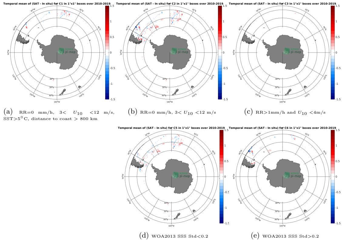
Figure 12: Temporal mean gridded over spatial boxes of size 1^{\circ}\times 1^{\circ} of \Delta\text{SSS} (CCI SSS L4 Merged-OI v2.31 - 7-day running (ESA) - TSG (Polarstern)) for 5 different subdatasets corresponding to:RR=0 mm/h, 3 < U_{10} < 12 m/s, SST >5^{\circ}\text{C} , distance to coast > 800 km (a), RR=0 mm/h, 3 < U_{10} < 12 m/s (b), RR >1 mm/h and U_{10} < 4 m/s (c), WOA2013 SSS Std <0.2 (d), WOA2013 SSS Std >0.2 (e).
