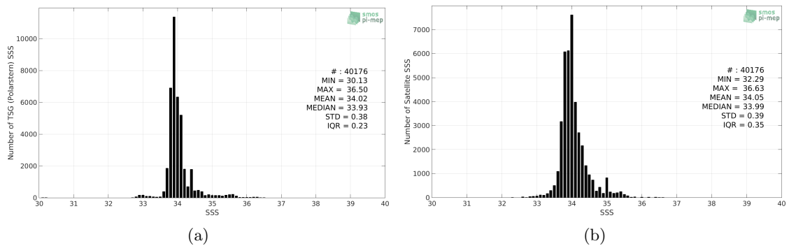
Figure 2: Histograms of SSS from TSG (Polarstern) (a) and CCI SSS L4 Merged-OI v2.31 - 7-day running (ESA) (b) considering all match-up pairs per bins of 0.1 over the Roaring Forties and Furious Fifties Pi-MEP region and for the full satellite product period.
