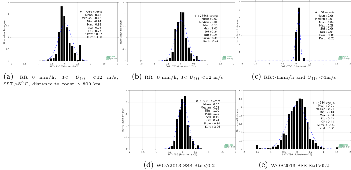
Figure 13: Normalized histogram of \Delta SSS (CCI SSS L4 Merged-OI v2.31 - 7-day running (ESA) - TSG (Polarstern)) for 5 different subdatasets corresponding to: RR=0 mm/h, 3 < U_{10} < 12 m/s, SST > 5°C, distance to coast > 800 km (a), RR=0 mm/h, 3 < U_{10} < 12 m/s (b), RR > 1mm/h and U_{10} < 4 m/s (c), WOA2013 SSS Std < 0.2 (d), WOA2013 SSS Std > 0.2 (e).
