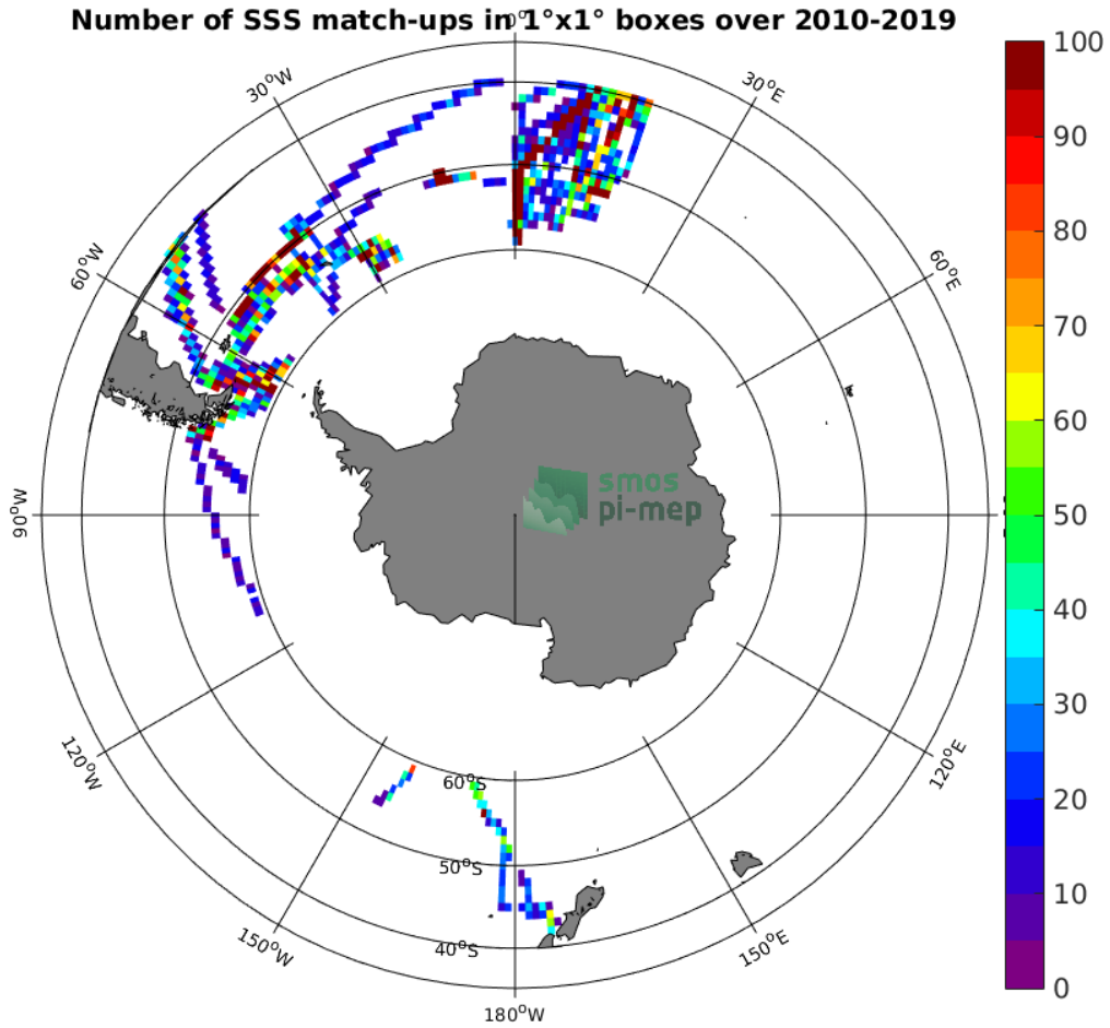
Figure 4: Number of SSS match-ups between TSG (Polarstern) SSS and the CCI SSS L4 Merged-OI v2.31 - 7-day running (ESA) SSS product for the Roaring Forties and Furious Fifties Pi-MEP region over 1°x1° boxes and for the full satellite product period.
