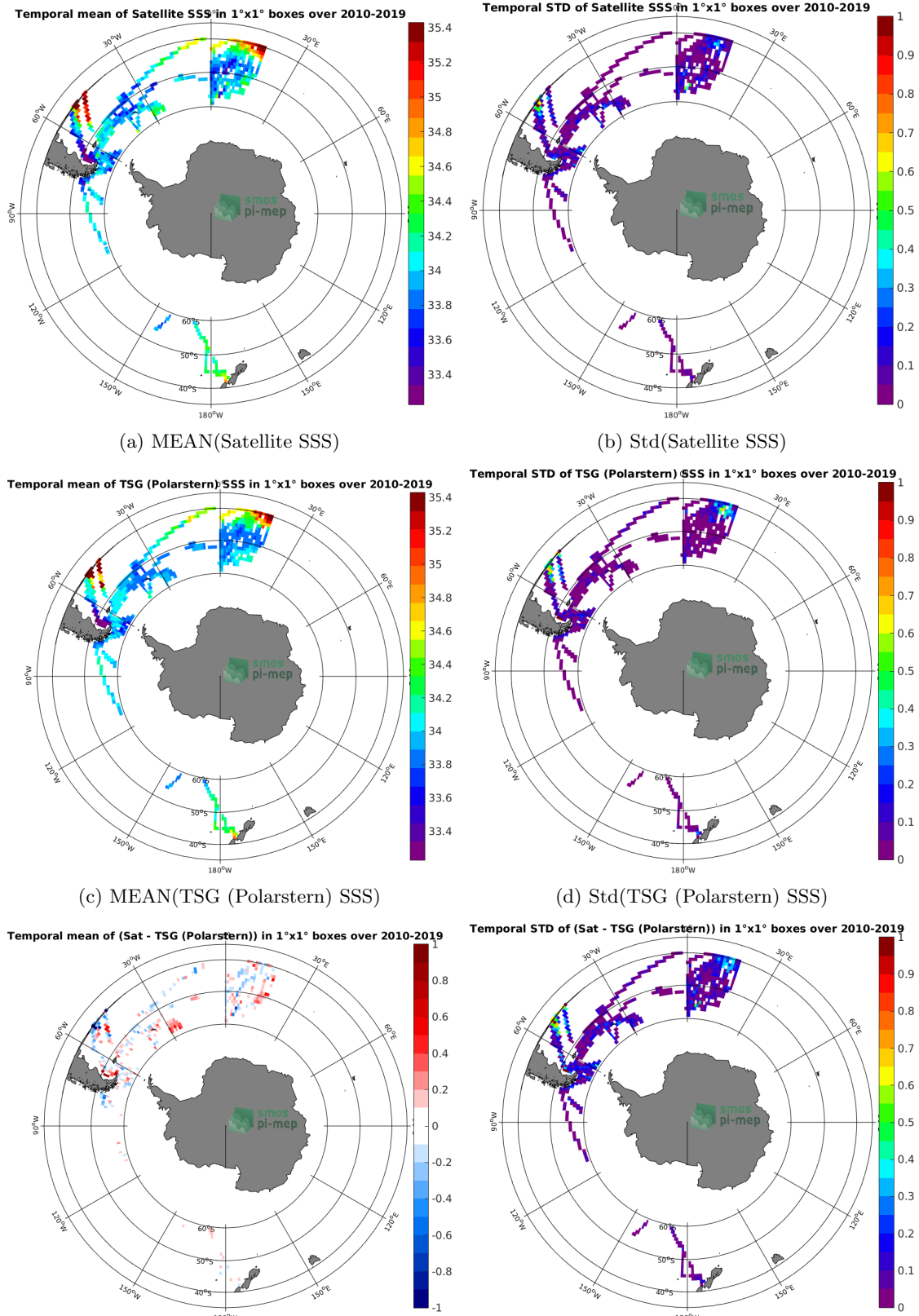
Figure 6: Temporal mean (left) and Std (right) of SSS from CCI SSS L4 Merged-OI v2.31 - 7-day running (ESA) (top), TSG (Polarstern) (middle), and of \Delta SSS (Satellite - TSG (Polarstern)). Only match-up pairs are used to generate these maps.
