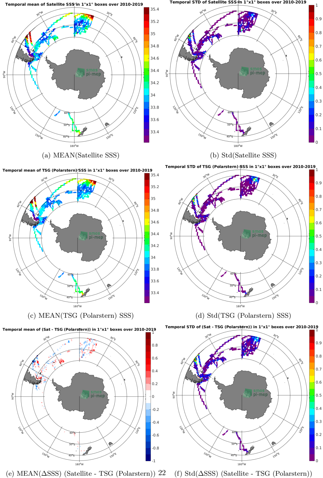
Figure 6: Temporal mean (left) and Std (right) of SSS from CCI L4 Merged-OI v2.31 - 7-day running (ESA) (top), TSG (Polarstern) (middle), and of \Delta SSS (Satellite - TSG (Polarstern)). Only match-up pairs are used to generate these maps.
