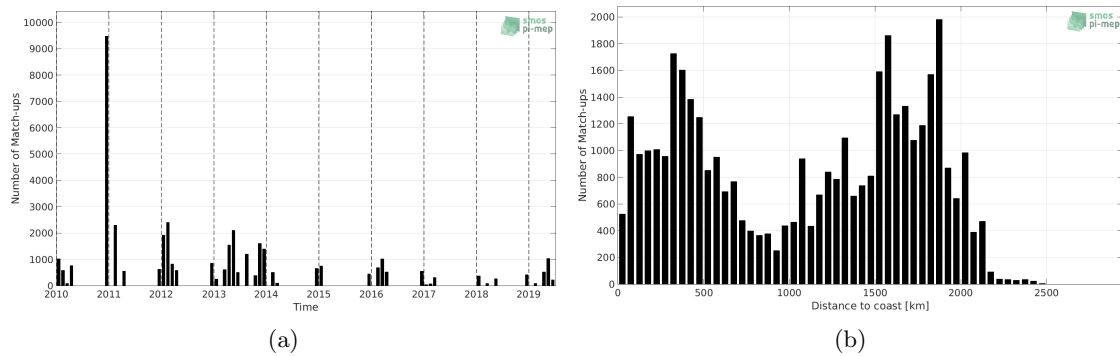
Figure 1: Number of match-ups between TSG (Polarstern) and CCI L4 Merged-OI v2.31 - 7-day running (ESA) SSS as a function of time (a) and as function of the distance to coast (b) over the Roaring Forties and Furious Fifties Pi-MEP region and for the full satellite product period.
