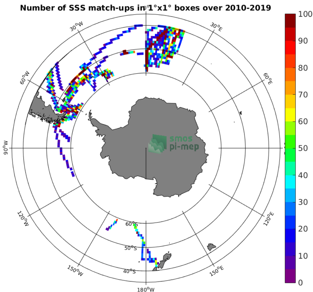
Figure 4: Number of SSS match-ups between TSG (Polarstern) SSS and the CCI L4 Merged-OI v2.31 - 7-day running (ESA) SSS product for the Roaring Forties and Furious Fifties Pi-MEP region over 1°x1° boxes and for the full satellite product period.
