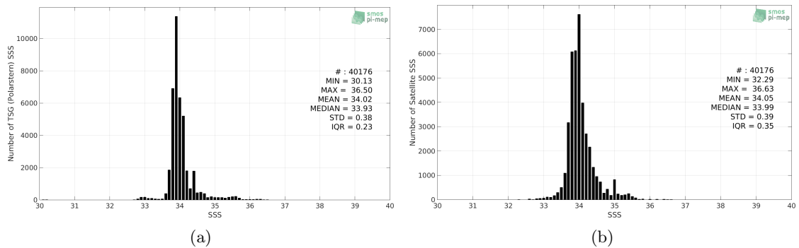
Figure 2: Histograms of SSS from TSG (Polarstern) (a) and CCI L4 Merged-OI v2.31 - 7-day running (ESA) (b) considering all match-up pairs per bins of 0.1 over the Roaring Forties and Furious Fifties Pi-MEP region and for the full satellite product period.
