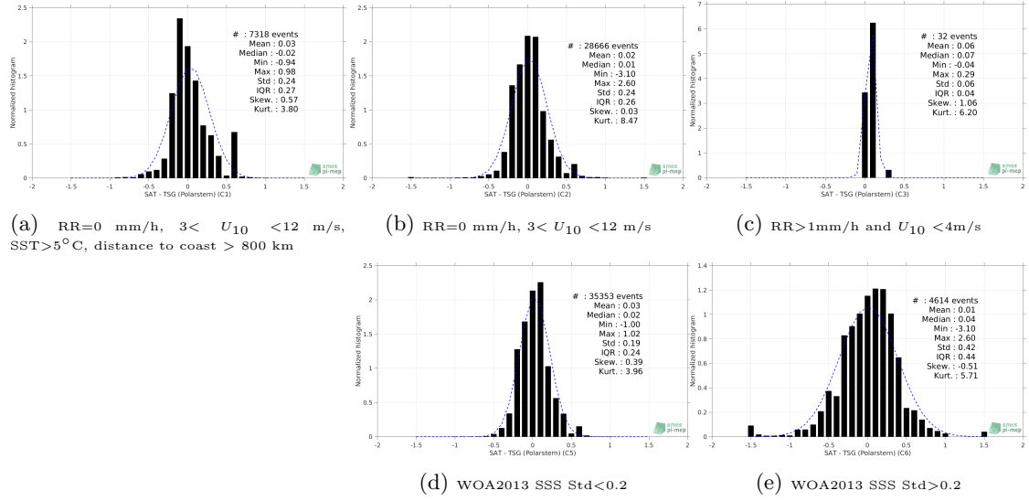
Figure 13: Normalized histogram of \Delta SSS (CCI L4 Merged-OI v2.31 - 7-day running (ESA) - TSG (Polarstern)) for 5 different subdatasets corresponding to: RR=0 mm/h, 3 < U_{10} < 12 m/s, SST > 5°C, distance to coast > 800 km (a), RR=0 mm/h, 3 < U_{10} < 12 m/s (b), RR > 1mm/h and U_{10} < 4 m/s (c), WOA2013 SSS Std < 0.2 (d), WOA2013 SSS Std > 0.2 (e).
