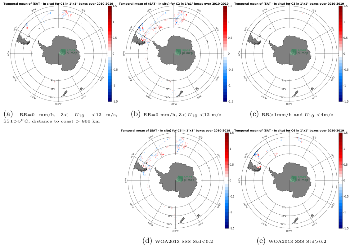
Figure 12: Temporal mean gridded over spatial boxes of size 1^{\circ}\times 1^{\circ} of \Delta\text{SSS} (CCI L4 Merged-OI v2.31 - 7-day running (ESA) - TSG (Polarstern)) for 5 different subdatasets corresponding to:RR=0 mm/h, 3 < U_{10} < 12 m/s, SST >5^{\circ}\text{C} , distance to coast > 800 km (a), RR=0 mm/h, 3 < U_{10} < 12 m/s (b), RR >1 mm/h and U_{10} < 4 m/s (c), WOA2013 SSS Std <0.2 (d), WOA2013 SSS Std >0.2 (e).
