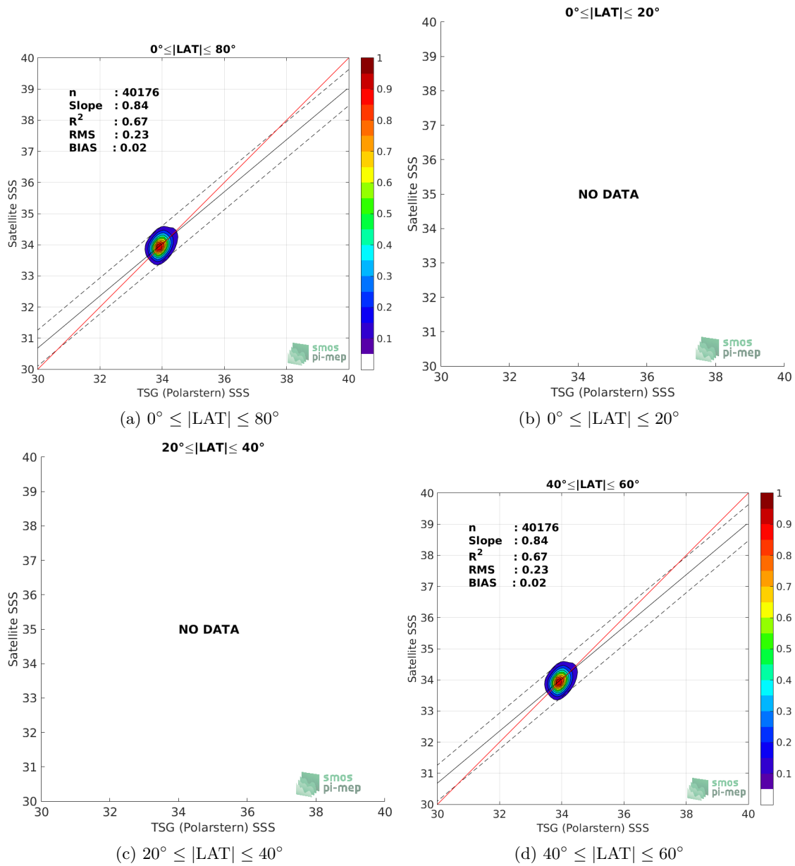
Figure 9: Contour maps of the concentration of CCI L4 Merged-OI v2.31 - 7-day running (ESA) SSS (y-axis) versus TSG (Polarstern) SSS (x-axis) at match-up pairs for different latitude bands. For each plot, the red line shows x=y . The black thin and dashed lines indicate a linear fit through the data cloud and the \pm 95\% confidence levels, respectively. The number match-up pairs n , the slope and R^2 coefficient of the linear fit, the root mean square (RMS) and the mean bias between satellite and in situ data are indicated for each latitude band in each plots.
