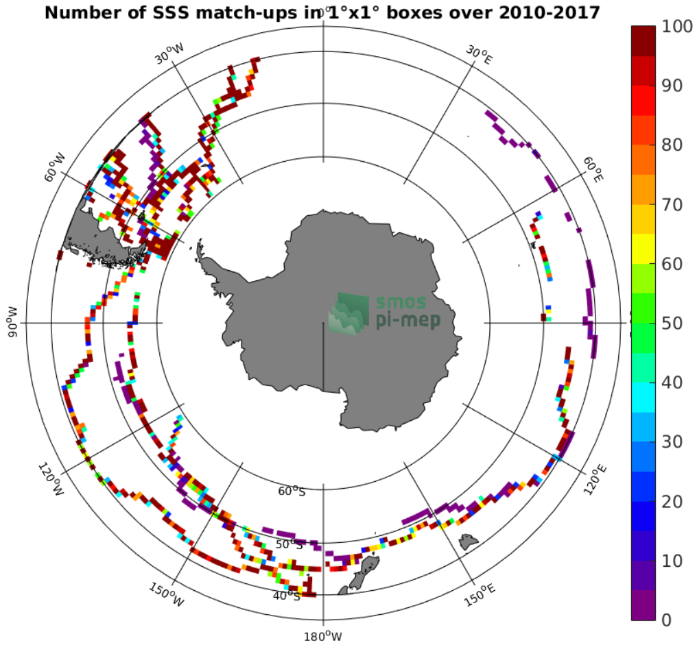
Figure 4: Number of SSS match-ups between TSG (GOSUD-Sailing-ship) SSS and the CCI SSS L4 Merged-OI v2.31 - 7-day running (ESA) SSS product for the Roaring Forties and Furious Fifties Pi-MEP region over 1^\circ \times 1^\circ boxes and for the full satellite product period.
