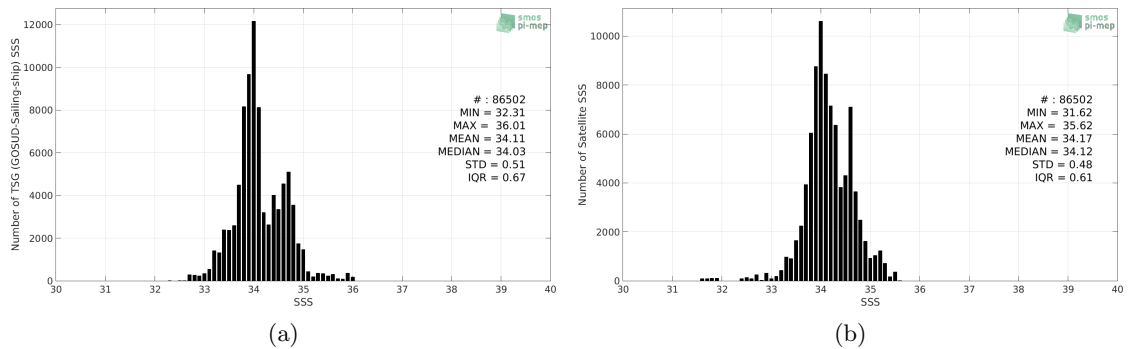
Figure 2: Histograms of SSS from TSG (GOSUD-Sailing-ship) (a) and CCI SSS L4 Merged-OI v2.31 - 7-day running (ESA) (b) considering all match-up pairs per bins of 0.1 over the Roaring Forties and Furious Fifties Pi-MEP region and for the full satellite product period.
