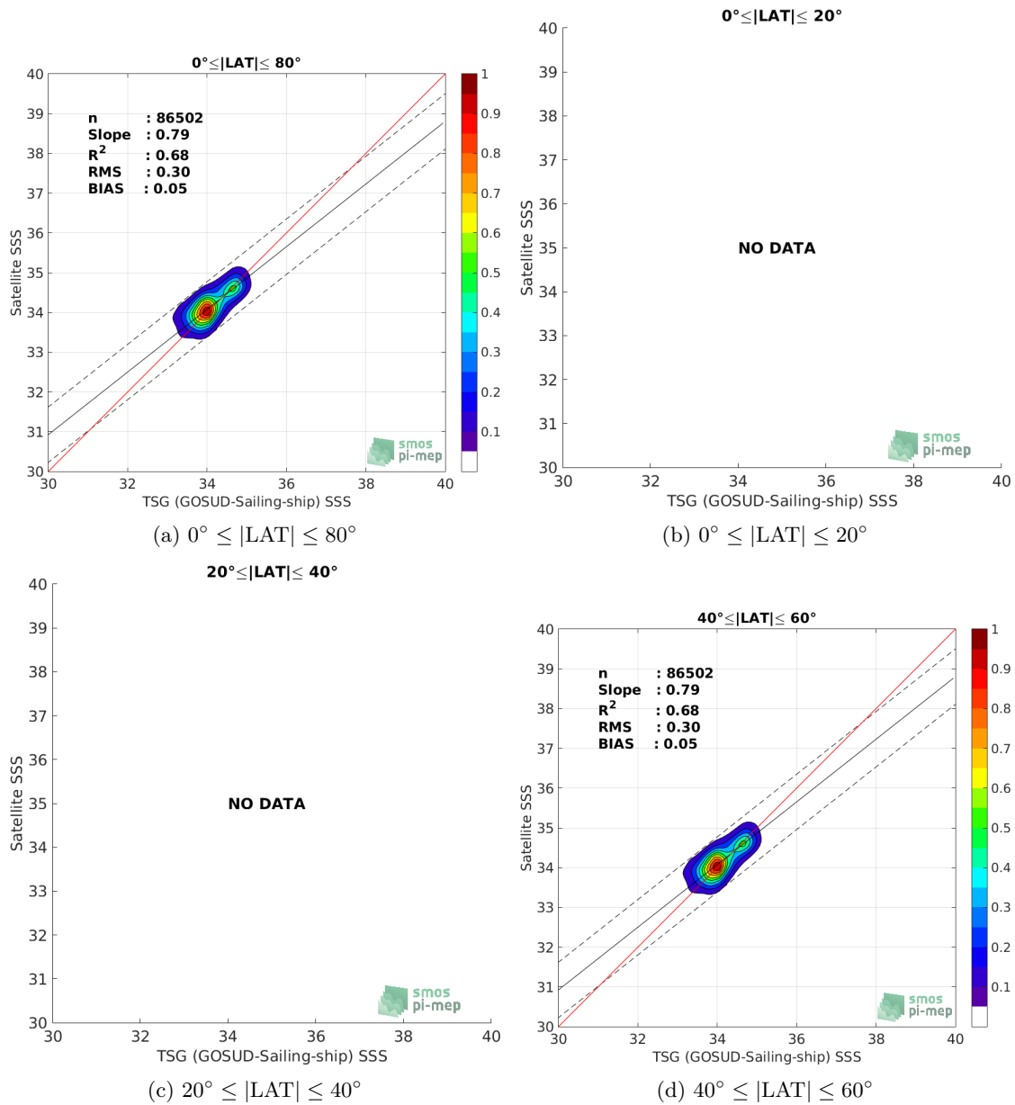
Figure 9: Contour maps of the concentration of CCI SSS L4 Merged-OI v2.31 - 7-day running (ESA) SSS (y-axis) versus TSG (GOSUD-Sailing-ship) SSS (x-axis) at match-up pairs for different latitude bands. For each plot, the red line shows x=y . The black thin and dashed lines indicate a linear fit through the data cloud and the \pm 95\% confidence levels, respectively. The number match-up pairs n , the slope and R^2 coefficient of the linear fit, the root mean square (RMS) and the mean bias between satellite and in situ data are indicated for each latitude band in each plots.
