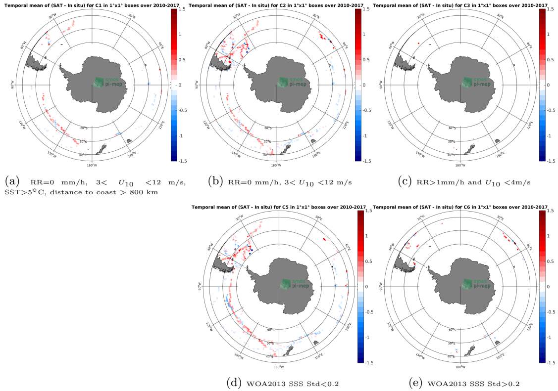
Figure 12: Temporal mean gridded over spatial boxes of size 1°x1° of \Delta SSS (CCI SSS L4 Merged-OI v2.31 - 7-day running (ESA) - TSG (GOSUD-Sailing-ship)) for 5 different subdatasets corresponding to:RR=0 mm/h, 3 < U_{10} < 12 m/s, SST>5°C, distance to coast > 800 km (a), RR=0 mm/h, 3 < U_{10} < 12 m/s (b), RR>1mm/h and U_{10} < 4 m/s (c), WOA2013 SSS Std<0.2 (d), WOA2013 SSS Std>0.2 (e).
