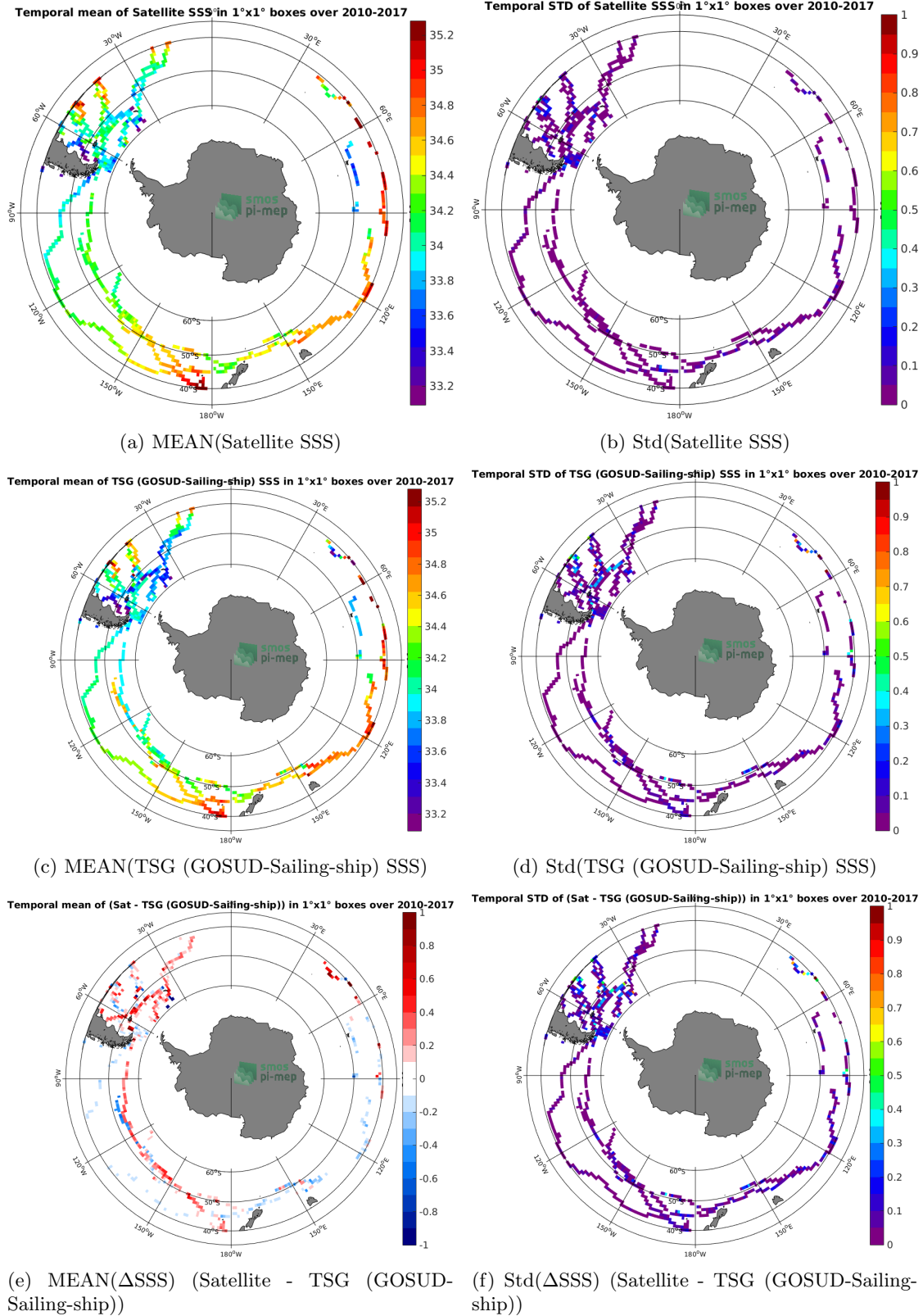
Figure 6: Temporal mean (left) and Std (right) of SSS from CCI SSS L4 Merged-OI v2.31 - 7-day running (ESA) (top), TSG (GOSUD-Sailing-ship) (middle), and of \Delta SSS (Satellite - TSG (GOSUD-Sailing-ship)). Only match-up pairs are used to generate these maps.
