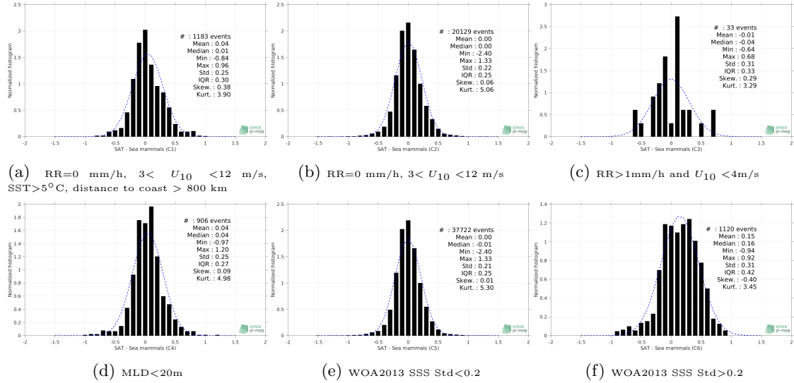
Figure 13: Normalized histogram of \Delta SSS (CCI SSS L4 Merged-OI v2.31 - 7-day running (ESA) - Sea mammals) for 6 different subdatasets corresponding to: RR=0 mm/h, 3 < U_{10} < 12 m/s, SST>5°C, distance to coast > 800 km (a), RR=0 mm/h, 3 < U_{10} < 12 m/s (b), RR>1mm/h and U_{10} < 4 m/s (c), MLD<20m (d), WOA2013 SSS Std<0.2 (e), WOA2013 SSS Std>0.2 (f).
