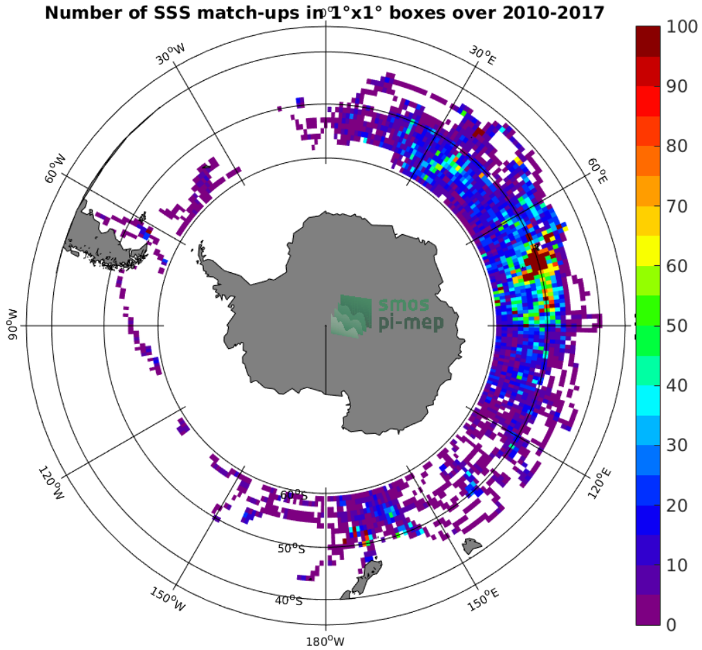
Figure 4: Number of SSS match-ups between Sea mammals SSS and the CCI SSS L4 Merged-OI v2.31 - 7-day running (ESA) SSS product for the Roaring Forties and Furious Fifties Pi-MEP region over 1°x1° boxes and for the full satellite product period.
