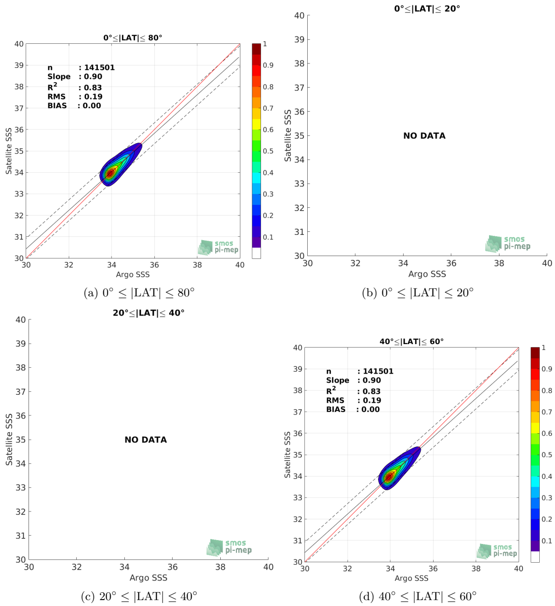
Figure 9: Contour maps of the concentration of CCI SSS L4 Merged-OI v2.31 - 7-day running (ESA) SSS (y-axis) versus Argo SSS (x-axis) at match-up pairs for different latitude bands. For each plot, the red line shows x=y . The black thin and dashed lines indicate a linear fit through the data cloud and the \pm 95\% confidence levels, respectively. The number match-up pairs n , the slope and R^2 coefficient of the linear fit, the root mean square (RMS) and the mean bias between satellite and in situ data are indicated for each latitude band in each plots.
