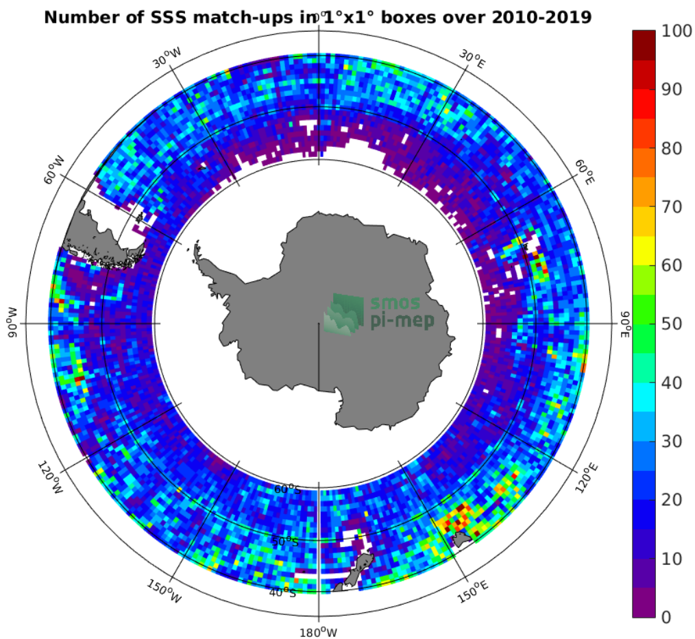
Figure 4: Number of SSS match-ups between Argo SSS and the CCI SSS L4 Merged-OI v2.31 - 7-day running (ESA) SSS product for the Roaring Forties and Furious Fifties Pi-MEP region over 1^\circ \times 1^\circ boxes and for the full satellite product period.
