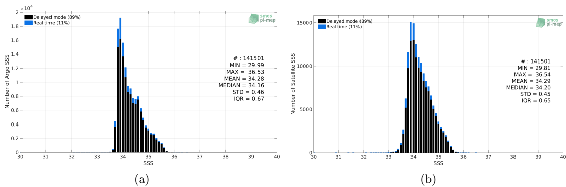
Figure 2: Histograms of SSS from Argo (a) and CCI SSS L4 Merged-OI v2.31 - 7-day running (ESA) (b) considering all match-up pairs per bins of 0.1 over the Roaring Forties and Furious Fifties Pi-MEP region and for the full satellite product period.
