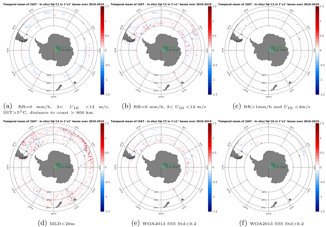
Figure 12: Temporal mean gridded over spatial boxes of size 1^{\circ}\times 1^{\circ} of \Delta\text{SSS} (CCI SSS L4 Merged-OI v2.31 - 7-day running (ESA) - Argo) for 6 different subdatasets corresponding to: \text{RR}=0 mm/h, 3 < U_{10} < 12 m/s, \text{SST}>5^{\circ}\text{C} , distance to coast > 800 km (a), \text{RR}=0 mm/h, 3 < U_{10} < 12 m/s (b), \text{RR}>1\text{mm/h} and U_{10} < 4\text{m/s} (c), \text{MLD}<20\text{m} (d), WOA2013 SSS Std < 0.2 (e), WOA2013 SSS Std > 0.2 (f).
