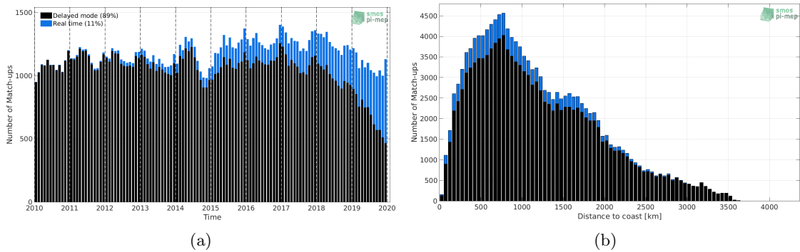
Figure 1: Number of match-ups between Argo and CCI SSS L4 Merged-OI v2.31 - 7-day running (ESA) SSS as a function of time (a) and as function of the distance to coast (b) over the Roaring Forties and Furious Fifties Pi-MEP region and for the full satellite product period.
