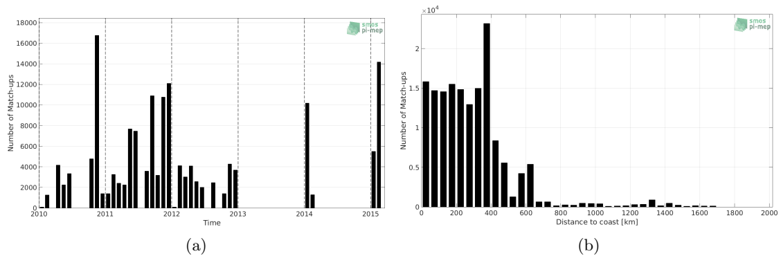
Figure 1: Number of match-ups between TSG (SAMOS) and CCI L4 Merged-OI v2.31 - 30-day running (ESA) SSS as a function of time (a) and as function of the distance to coast (b) over the Roaring Forties and Furious Fifties Pi-MEP region and for the full satellite product period.
