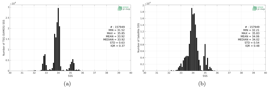
Figure 2: Histograms of SSS from TSG (SAMOS) (a) and CCI L4 Merged-OI v2.31 - 30-day running (ESA) (b) considering all match-up pairs per bins of 0.1 over the Roaring Forties and Furious Fifties Pi-MEP region and for the full satellite product period.
