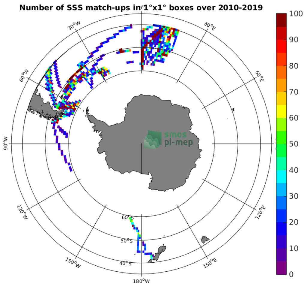
Figure 4: Number of SSS match-ups between TSG (Polarstern) SSS and the CCI L4 Merged-OI v2.31 - 30-day running (ESA) SSS product for the Roaring Forties and Furious Fifties Pi-MEP region over 1^\circ \times 1^\circ boxes and for the full satellite product period.
