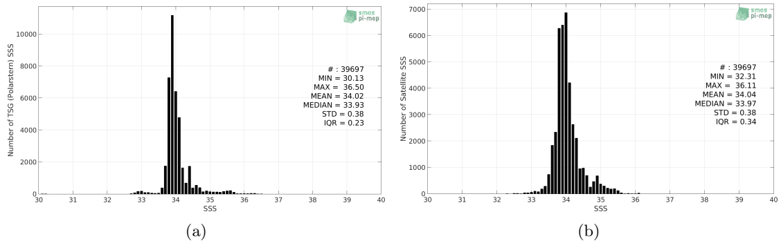
Figure 2: Histograms of SSS from TSG (Polarstern) (a) and CCI L4 Merged-OI v2.31 - 30-day running (ESA) (b) considering all match-up pairs per bins of 0.1 over the Roaring Forties and Furious Fifties Pi-MEP region and for the full satellite product period.
