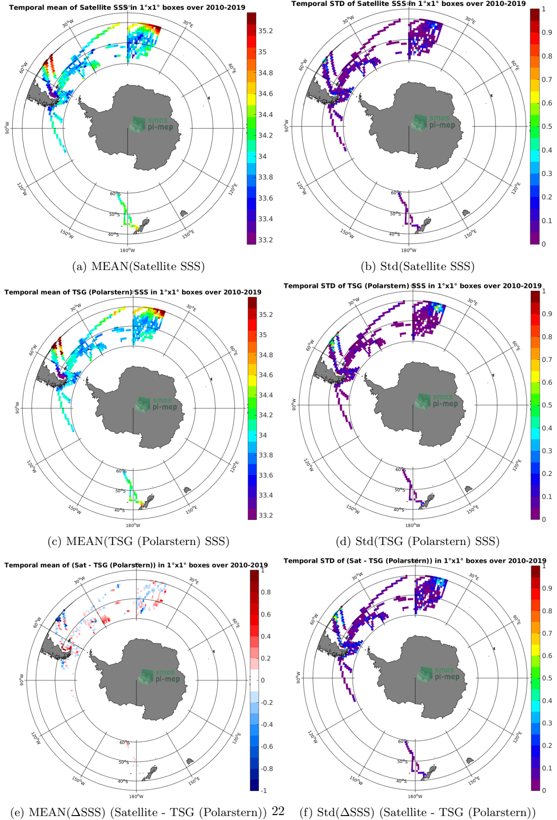
Figure 6: Temporal mean (left) and Std (right) of SSS from CCI L4 Merged-OI v2.31 - 30-day running (ESA) (top), TSG (Polarstern) (middle), and of \Delta SSS (Satellite - TSG (Polarstern)). Only match-up pairs are used to generate these maps.
