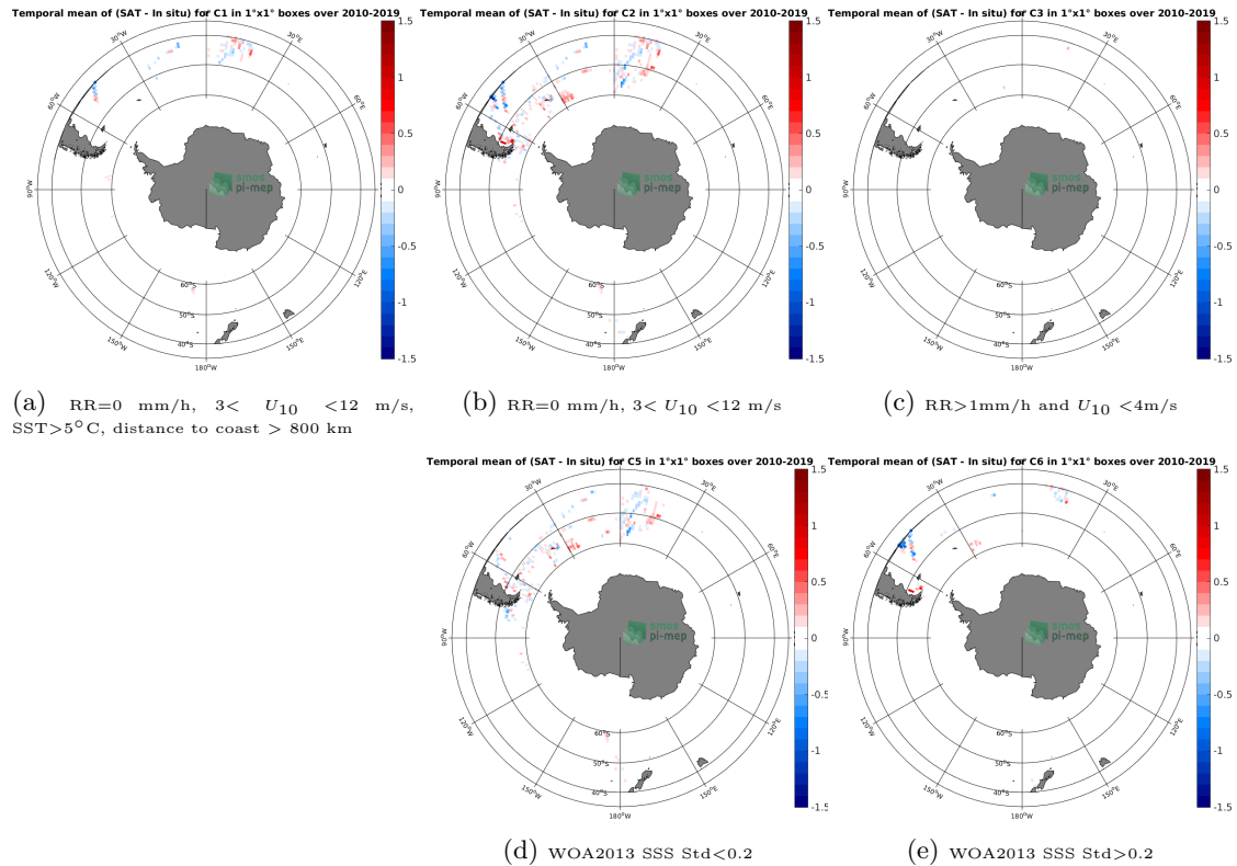
Figure 12: Temporal mean gridded over spatial boxes of size 1^{\circ}\times 1^{\circ} of \Delta\text{SSS} (CCI L4 Merged-OI v2.31 - 30-day running (ESA) - TSG (Polarstern)) for 5 different subdatasets corresponding to:RR=0 mm/h, 3 < U_{10} < 12 m/s, SST >5^{\circ}\text{C} , distance to coast > 800 km (a), RR=0 mm/h, 3 < U_{10} < 12 m/s (b), RR >1 mm/h and U_{10} < 4 m/s (c), WOA2013 SSS Std <0.2 (d), WOA2013 SSS Std >0.2 (e).
