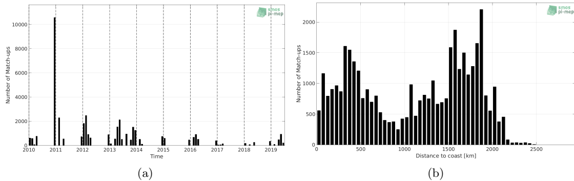
Figure 1: Number of match-ups between TSG (Polarstern) and CCI L4 Merged-OI v2.31 - 30-day running (ESA) SSS as a function of time (a) and as function of the distance to coast (b) over the Roaring Forties and Furious Fifties Pi-MEP region and for the full satellite product period.
