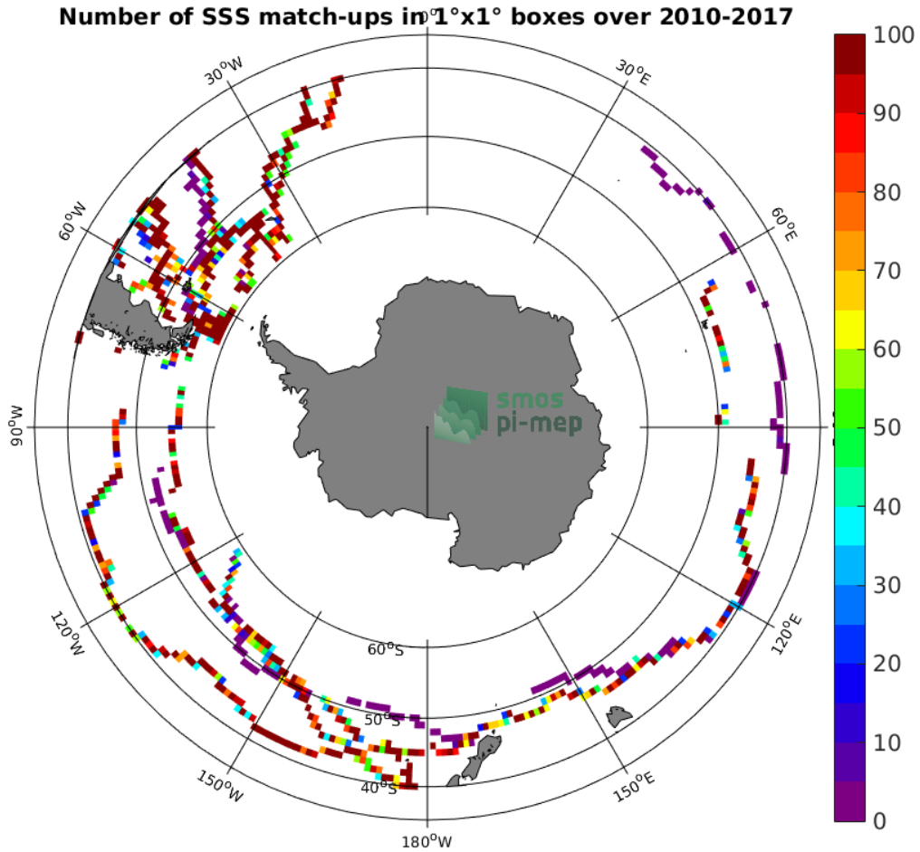
Figure 4: Number of SSS match-ups between TSG (GOSUD-Sailing-ship) SSS and the CCI SSS L4 Merged-OI v2.31 - 30-day running (ESA) SSS product for the Roaring Forties and Furious Fifties Pi-MEP region over 1°x1° boxes and for the full satellite product period.
