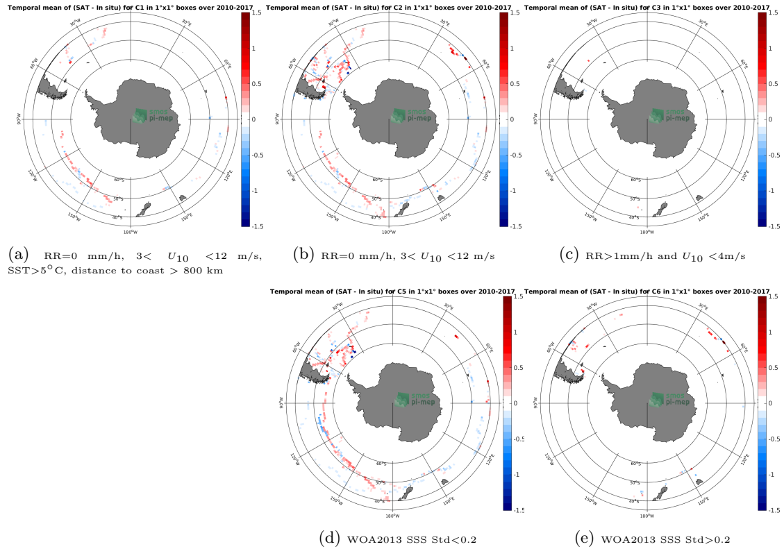
Figure 12: Temporal mean gridded over spatial boxes of size 1°x1° of \Delta SSS (CCI SSS L4 Merged-OI v2.31 - 30-day running (ESA) - TSG (GOSUD-Sailing-ship)) for 5 different subdatasets corresponding to: RR=0 mm/h, 3 < U_{10} < 12 m/s, SST > 5°C, distance to coast > 800 km (a), RR=0 mm/h, 3 < U_{10} < 12 m/s (b), RR > 1mm/h and U_{10} < 4 m/s (c), WOA2013 SSS Std < 0.2 (d), WOA2013 SSS Std > 0.2 (e).
