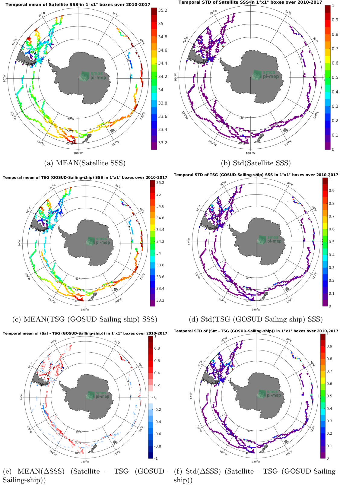
Figure 6: Temporal mean (left) and Std (right), of SSS from CCI SSS L4 Merged-OI v2.31 - 30-day running (ESA) (top), TSG (GOSUD-Sailing-ship) (middle), and of \Delta SSS (Satellite - TSG (GOSUD-Sailing-ship)). Only match-up pairs are used to generate these maps.
