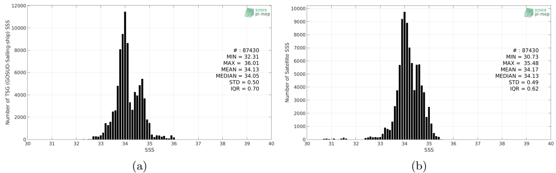
Figure 2: Histograms of SSS from TSG (GOSUD-Sailing-ship) (a) and CCI SSS L4 Merged-OI v2.31 - 30-day running (ESA) (b) considering all match-up pairs per bins of 0.1 over the Roaring Forties and Furious Fifties Pi-MEP region and for the full satellite product period.
