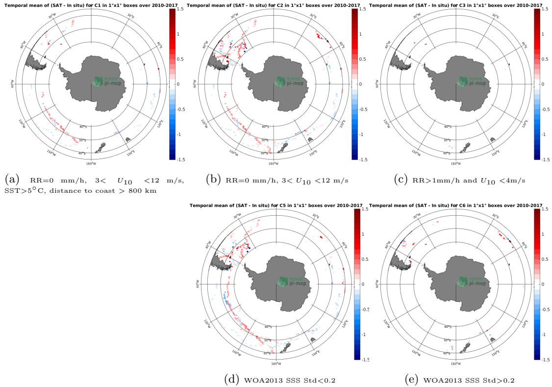
Figure 12: Temporal mean gridded over spatial boxes of size 1°x1° of \Delta SSS (CCI L4 Merged-OI v2.31 - 30-day running (ESA) - TSG (GOSUD-Sailing-ship)) for 5 different subdatasets corresponding to: RR=0 mm/h, 3 < U_{10} < 12 m/s, SST > 5°C, distance to coast > 800 km (a), RR=0 mm/h, 3 < U_{10} < 12 m/s (b), RR > 1mm/h and U_{10} < 4 m/s (c), WOA2013 SSS Std < 0.2 (d), WOA2013 SSS Std > 0.2 (e).
