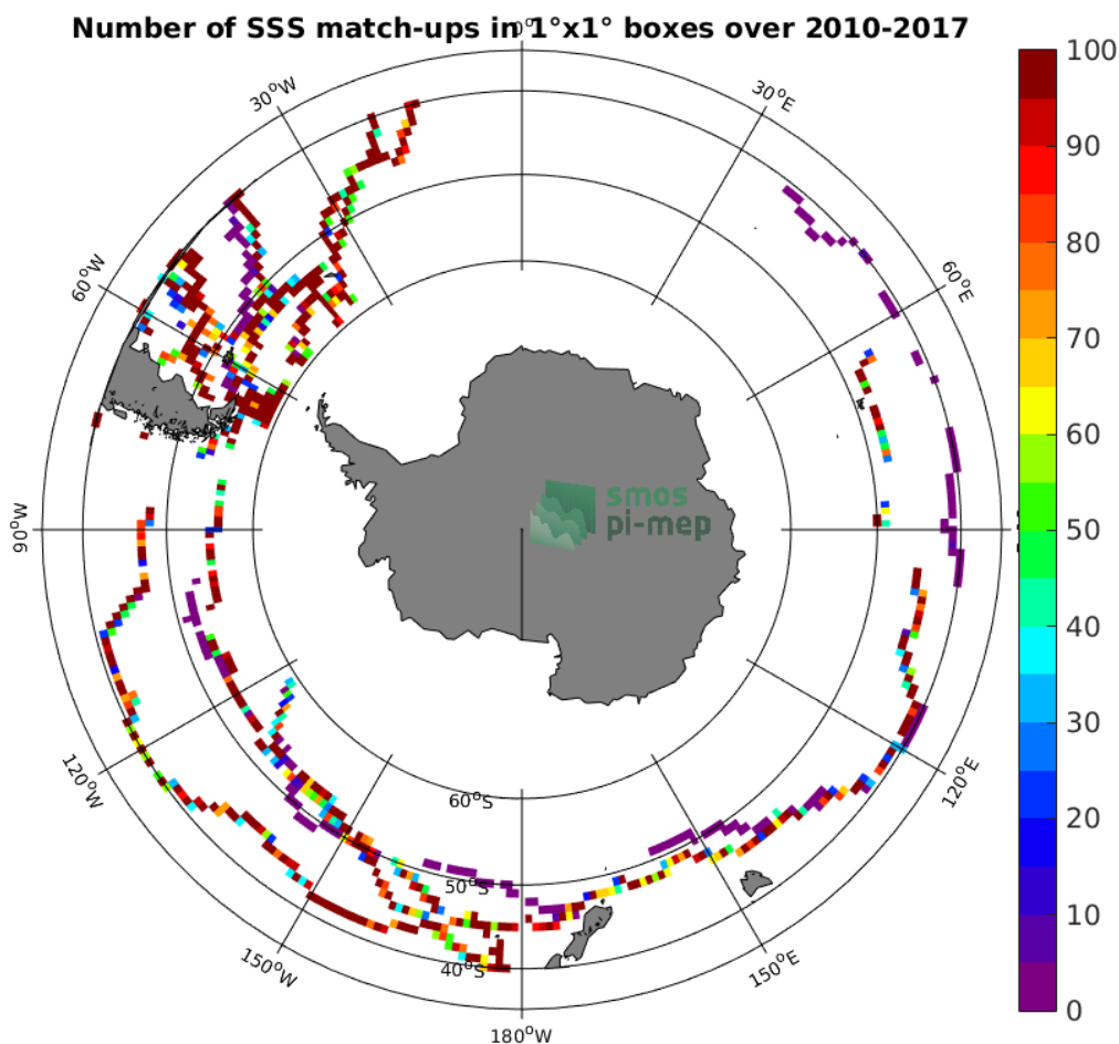
Figure 4: Number of SSS match-ups between TSG (GOSUD-Sailing-ship) SSS and the CCI L4 Merged-OI v2.31 - 30-day running (ESA) SSS product for the Roaring Forties and Furious Fifties Pi-MEP region over 1°x1° boxes and for the full satellite product period.
