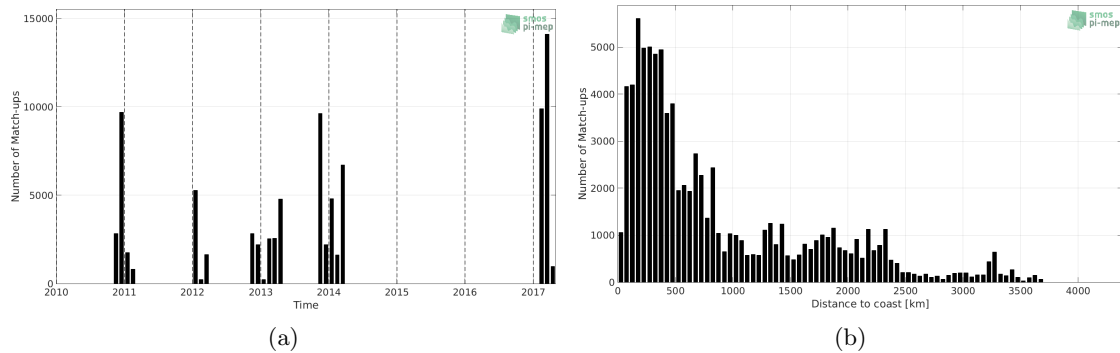
Figure 1: Number of match-ups between TSG (GOSUD-Sailing-ship) and CCI L4 Merged-OI v2.31 - 30-day running (ESA) SSS as a function of time (a) and as function of the distance to coast (b) over the Roaring Forties and Furious Fifties Pi-MEP region and for the full satellite product period.
