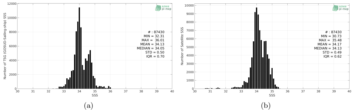
Figure 2: Histograms of SSS from TSG (GOSUD-Sailing-ship) (a) and CCI L4 Merged-OI v2.31 - 30-day running (ESA) (b) considering all match-up pairs per bins of 0.1 over the Roaring Forties and Furious Fifties Pi-MEP region and for the full satellite product period.
