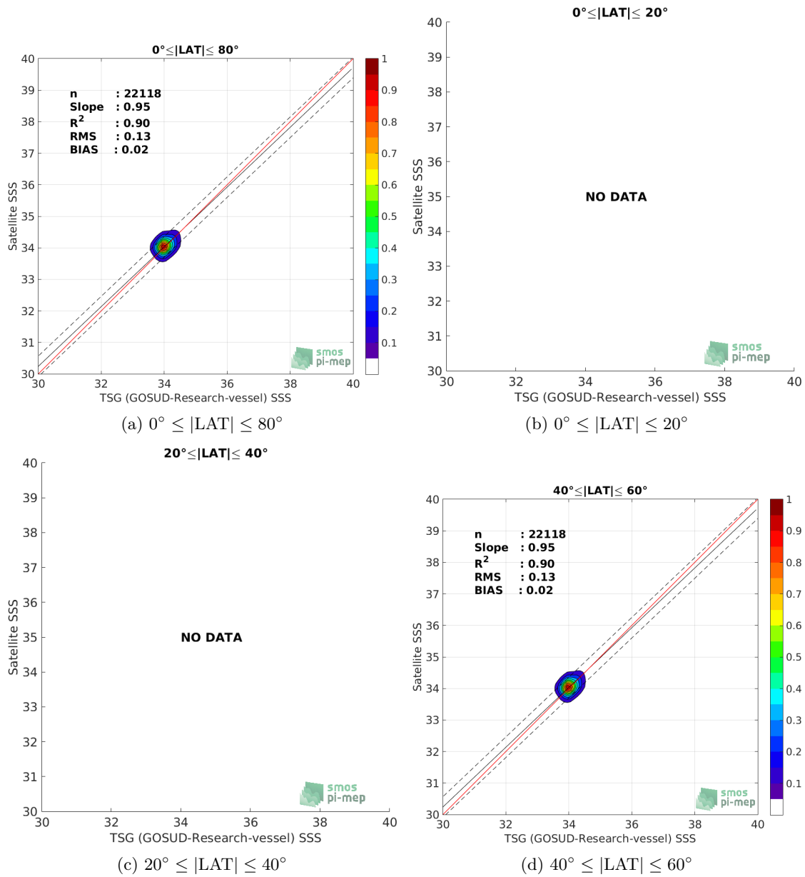
Figure 9: Contour maps of the concentration of CCI SSS L4 Merged-OI v2.31 - 30-day running (ESA) SSS ( y -axis) versus TSG (GOSUD-Research-vessel) SSS ( x -axis) at match-up pairs for different latitude bands. For each plot, the red line shows x=y . The black thin and dashed lines indicate a linear fit through the data cloud and the \pm 95\% confidence levels, respectively. The number match-up pairs n , the slope and R^2 coefficient of the linear fit, the root mean square (RMS) and the mean bias between satellite and in situ data are indicated for each latitude band in each plots.
