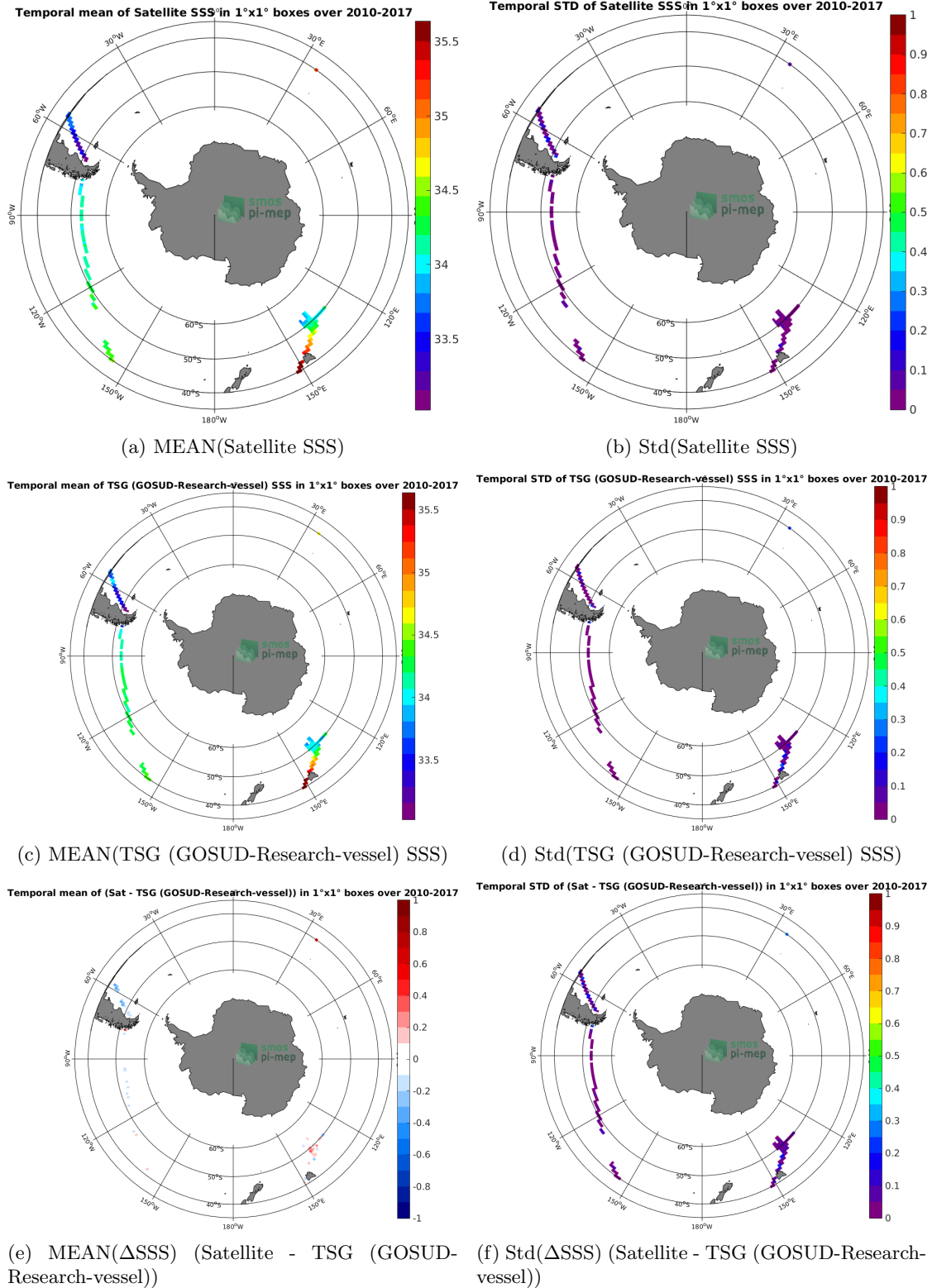
Figure 6: Temporal mean (left) and Std (right) of SSS from CCI SSS L4 Merged-OI v2.31 - 30-day running (ESA) (top), TSG (GOSUD-Research-vessel) (middle), and of \Delta SSS (Satellite - TSG (GOSUD-Research-vessel)). Only match-up pairs are used to generate these maps.
