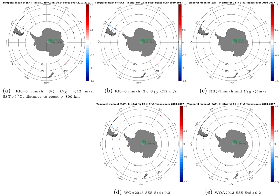
Figure 12: Temporal mean gridded over spatial boxes of size 1^\circ \times 1^\circ of \Delta SSS (CCI SSS L4 Merged-OI v2.31 - 30-day running (ESA) - TSG (GOSUD-Research-vessel)) for 5 different subdatasets corresponding to: RR=0 mm/h, 3 < U_{10} < 12 m/s, SST > 5°C, distance to coast > 800 km (a), RR=0 mm/h, 3 < U_{10} < 12 m/s (b), RR > 1mm/h and U_{10} < 4 m/s (c), WOA2013 SSS Std < 0.2 (d), WOA2013 SSS Std > 0.2 (e).
