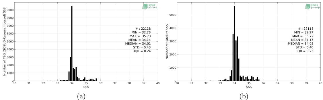
Figure 2: Histograms of SSS from TSG (GOSUD-Research-vessel) (a) and CCI SSS L4 Merged-OI v2.31 - 30-day running (ESA) (b) considering all match-up pairs per bins of 0.1 over the Roaring Forties and Furious Fifties Pi-MEP region and for the full satellite product period.
