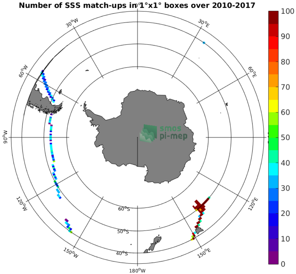
Figure 4: Number of SSS match-ups between TSG (GOSUD-Research-vessel) SSS and the CCI SSS L4 Merged-OI v2.31 - 30-day running (ESA) SSS product for the Roaring Forties and Furious Fifties Pi-MEP region over 1°x1° boxes and for the full satellite product period.
