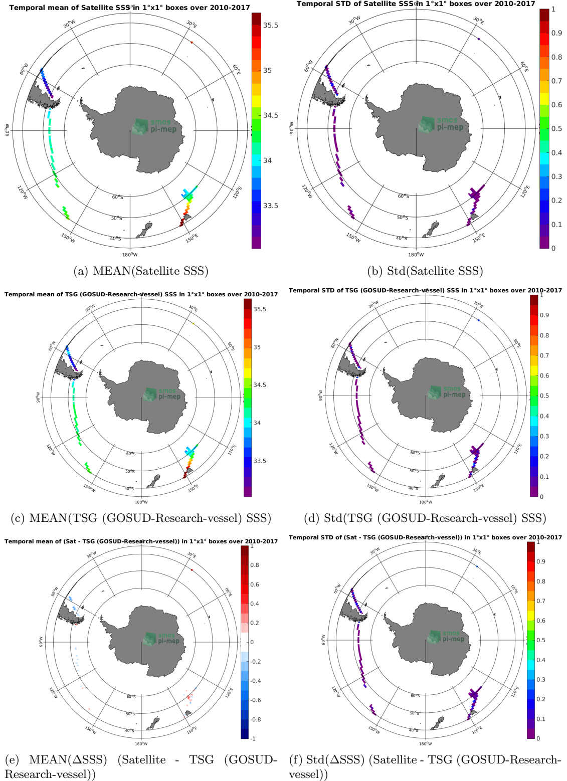
Figure 6: Temporal mean (left) and Std (right) of SSS from CCI L4 Merged-OI v2.31 - 30-day running (ESA) (top), TSG (GOSUD-Research-vessel) (middle), and of \Delta SSS (Satellite - TSG (GOSUD-Research-vessel)). Only match-up pairs are used to generate these maps.
