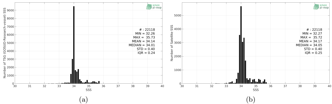
Figure 2: Histograms of SSS from TSG (GOSUD-Research-vessel) (a) and CCI L4 Merged-OI v2.31 - 30-day running (ESA) (b) considering all match-up pairs per bins of 0.1 over the Roaring Forties and Furious Fifties Pi-MEP region and for the full satellite product period.
