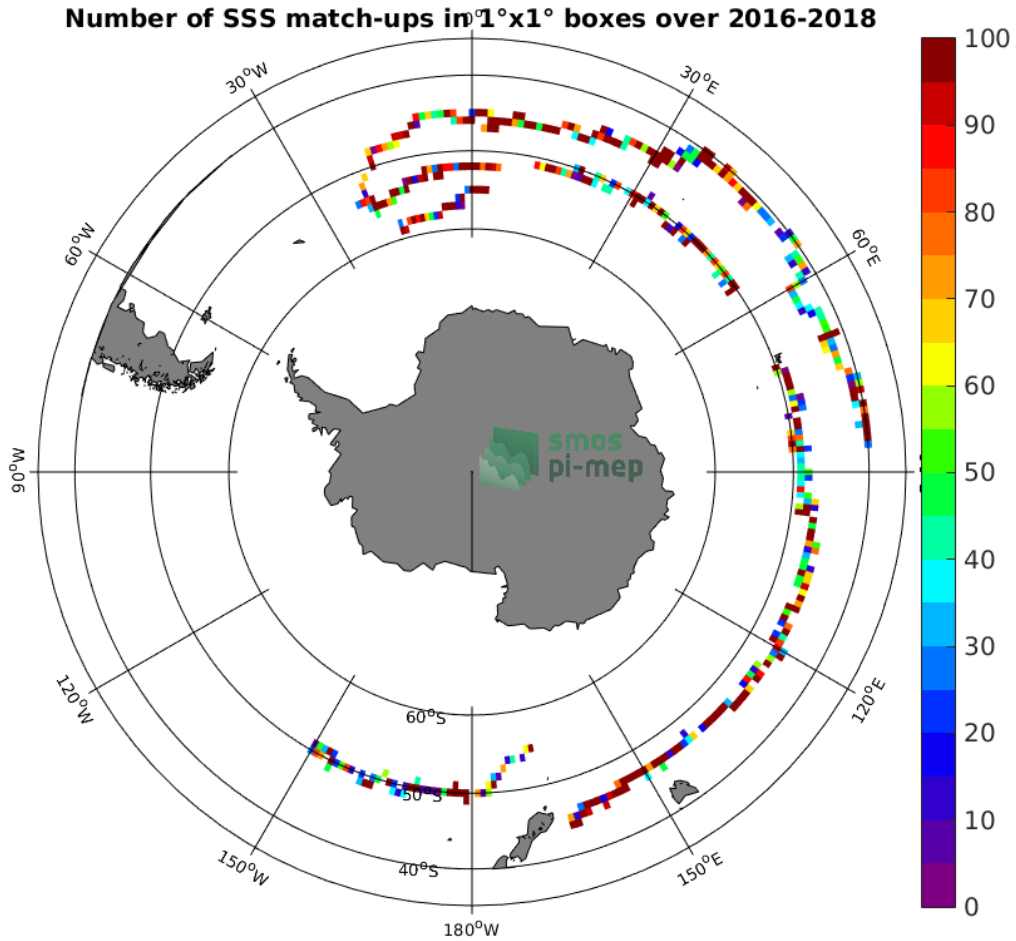
Figure 3: Number of SSS match-ups between Surface drifters SSS and the CCI SSS L4 Merged-OI v2.31 - 30-day running (ESA) SSS product for the Roaring Forties and Furious Fifties Pi-MEP region over 1°x1° boxes and for the full satellite product period.
