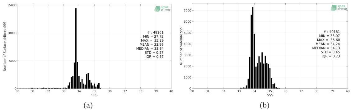
Figure 2: Histograms of SSS from Surface drifters (a) and CCI SSS L4 Merged-OI v2.31 - 30-day running (ESA) (b) considering all match-up pairs per bins of 0.1 over the Roaring Forties and Furious Fifties Pi-MEP region and for the full satellite product period.
