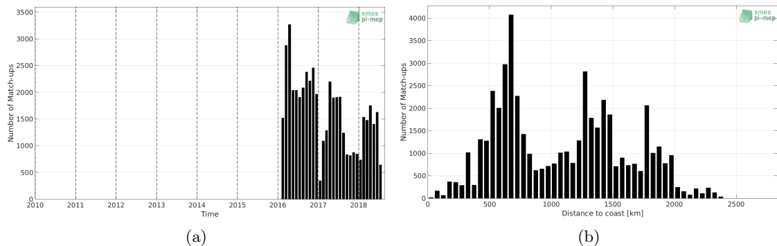
Figure 1: Number of match-ups between Surface drifters and CCI SSS L4 Merged-OI v2.31 - 30-day running (ESA) SSS as a function of time (a) and as function of the distance to coast (b) over the Roaring Forties and Furious Fifties Pi-MEP region and for the full satellite product period.
