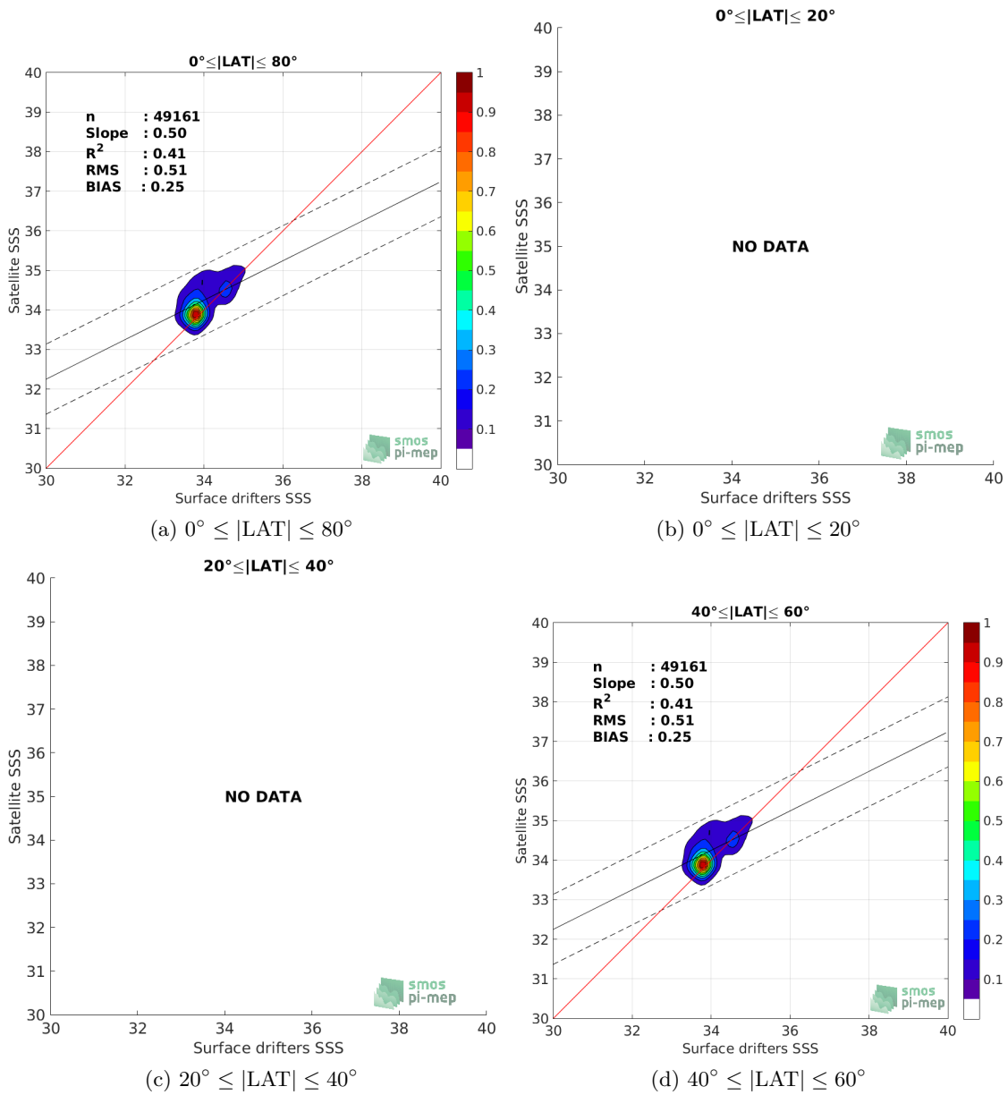
Figure 8: Contour maps of the concentration of CCI SSS L4 Merged-OI v2.31 - 30-day running (ESA) SSS (y-axis) versus Surface drifters SSS (x-axis) at match-up pairs for different latitude bands. For each plot, the red line shows x=y . The black thin and dashed lines indicate a linear fit through the data cloud and the \pm 95\% confidence levels, respectively. The number match-up pairs n , the slope and R^2 coefficient of the linear fit, the root mean square (RMS) and the mean bias between satellite and in situ data are indicated for each latitude band in each plots.
