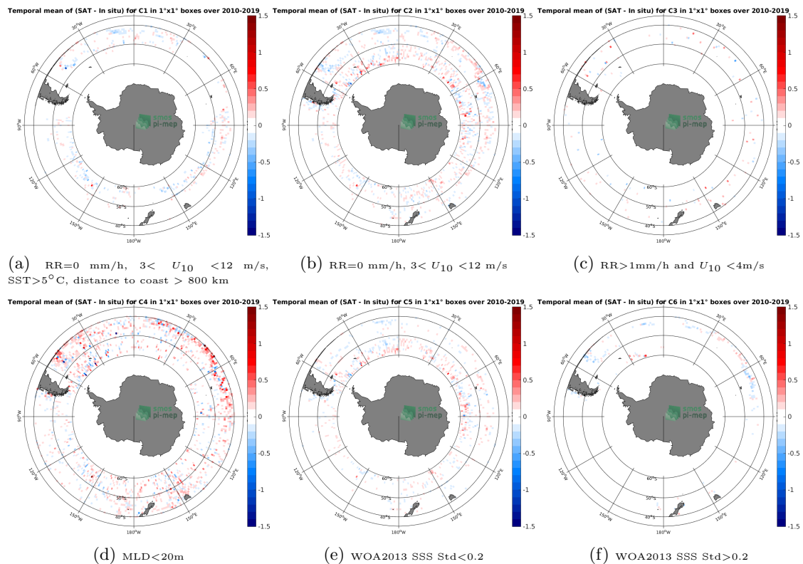
Figure 12: Temporal mean gridded over spatial boxes of size 1^{\circ}\times 1^{\circ} of \Delta\text{SSS} (CCI L4 Merged-OI v2.31 - 30-day running (ESA) - Argo) for 6 different subdatasets corresponding to:RR=0 mm/h, 3 < U_{10} < 12 m/s, SST >5^{\circ}\text{C} , distance to coast > 800 km (a), RR=0 mm/h, 3 < U_{10} < 12 m/s (b), RR >1 mm/h and U_{10} < 4 m/s (c),MLD <20 m (d),WOA2013 SSS Std <0.2 (e),WOA2013 SSS Std >0.2 (f).
