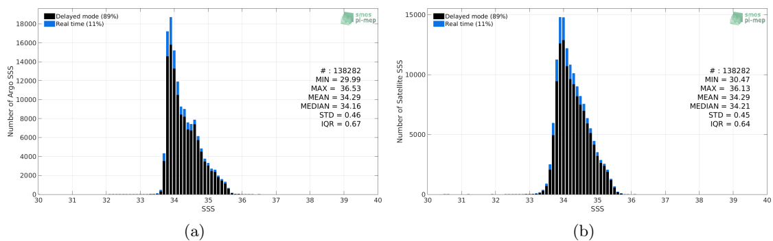
Figure 2: Histograms of SSS from Argo (a) and CCI L4 Merged-OI v2.31 - 30-day running (ESA) (b) considering all match-up pairs per bins of 0.1 over the Roaring Forties and Furious Fifties Pi-MEP region and for the full satellite product period.
