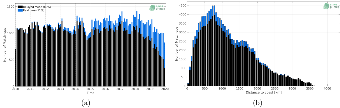
Figure 1: Number of match-ups between Argo and CCI L4 Merged-OI v2.31 - 30-day running (ESA) SSS as a function of time (a) and as function of the distance to coast (b) over the Roaring Forties and Furious Fifties Pi-MEP region and for the full satellite product period.
