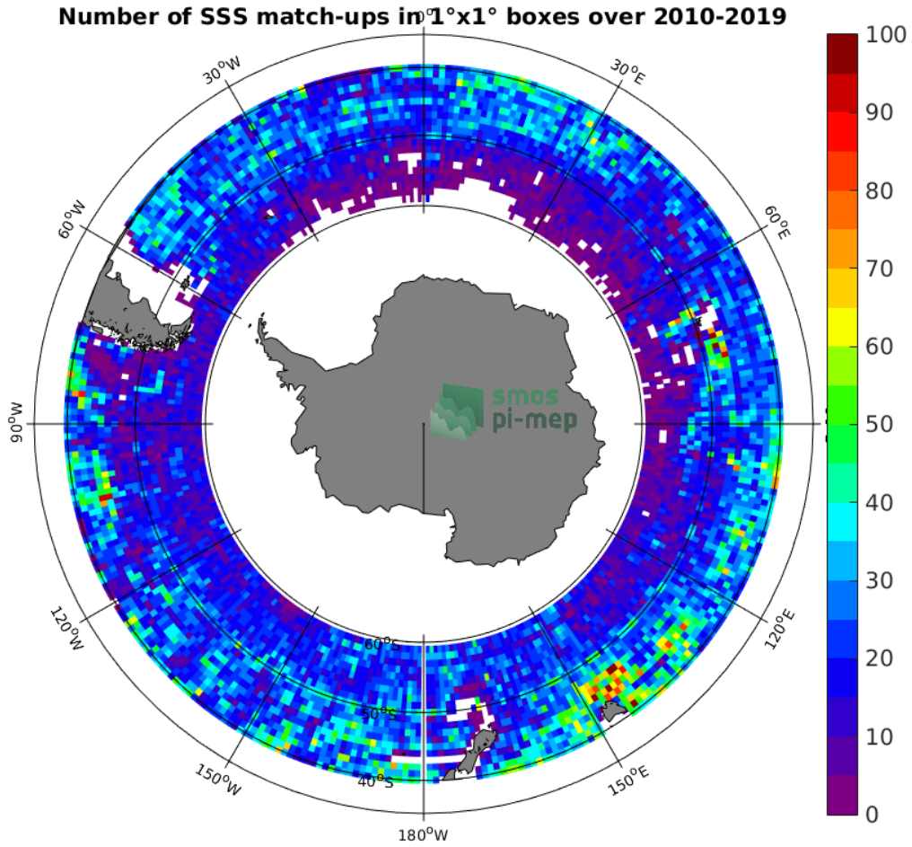
Figure 4: Number of SSS match-ups between Argo SSS and the CCI L4 Merged-OI v2.31 - 30-day running (ESA) SSS product for the Roaring Forties and Furious Fifties Pi-MEP region over 1°x1° boxes and for the full satellite product period.
