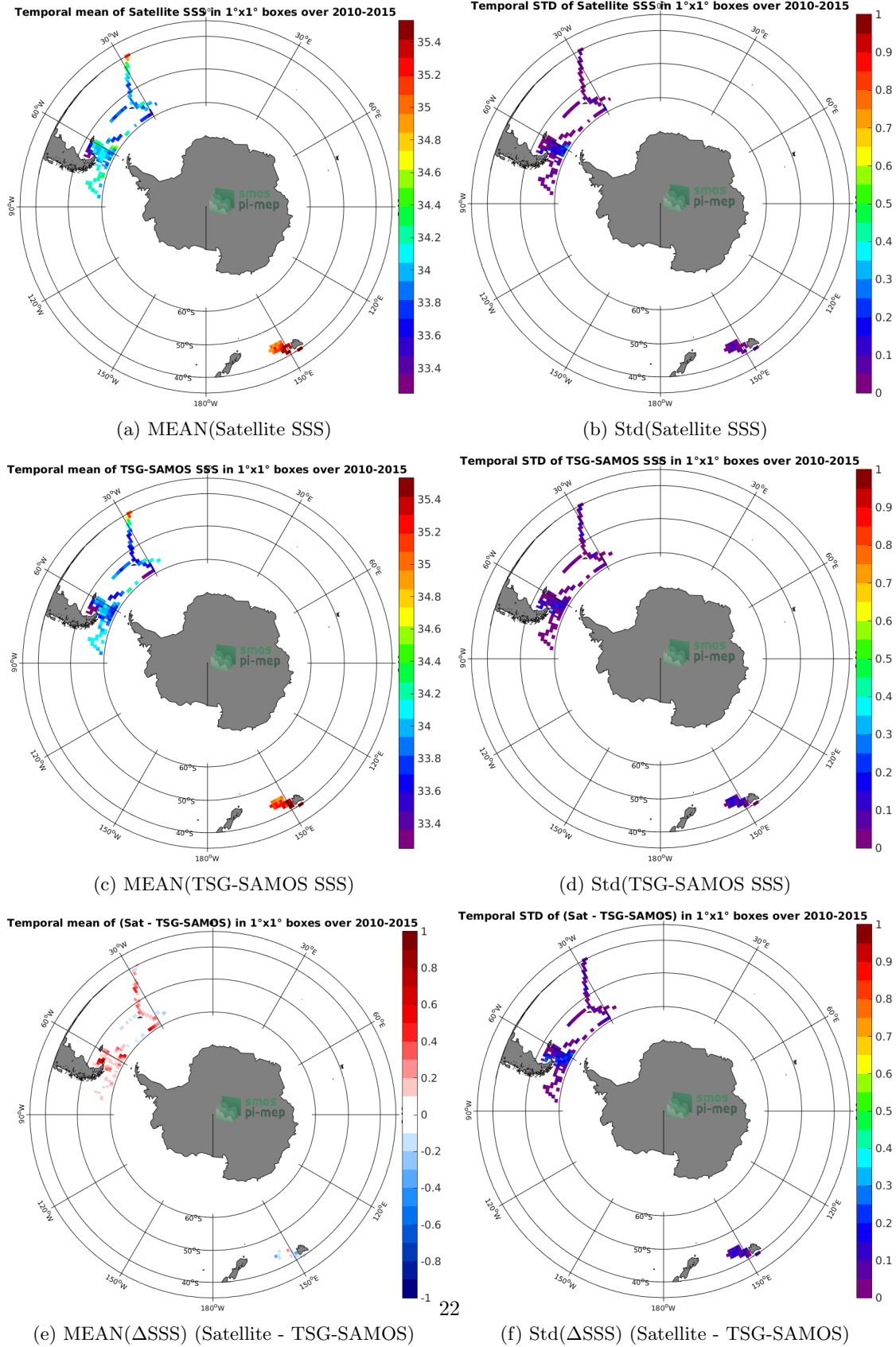
Figure 6: Temporal mean (left) and Std (right) of SSS from CCI-L4-ESA-MERGED-OI-V1.8-7DAY-RUNNING (top), TSG-SAMOS (middle), and of \Delta SSS (Satellite - TSG-SAMOS). Only match-up pairs are used to generate these maps.
