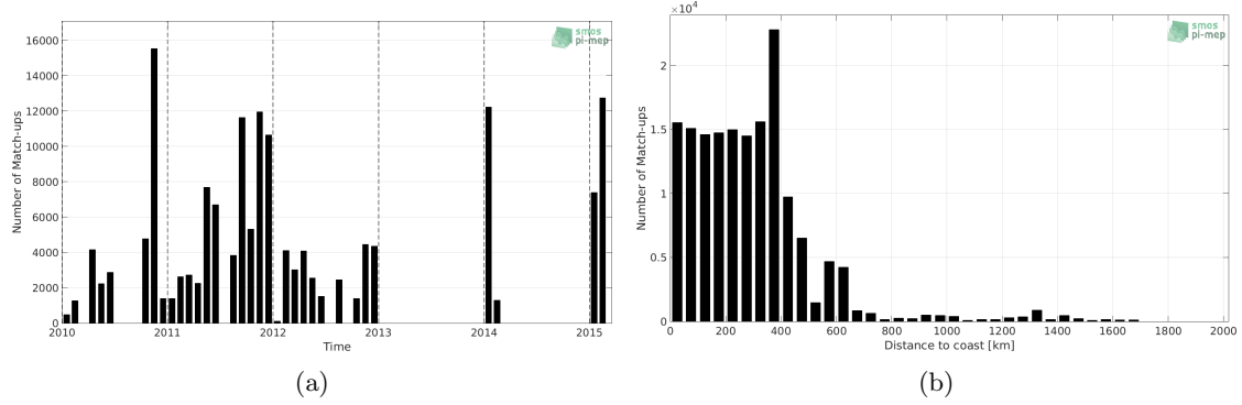
Figure 1: Number of match-ups between TSG-SAMOS and CCI-L4-ESA-MERGED-OI-V1.8-7DAY-RUNNING SSS as a function of time (a) and as function of the distance to coast (b) over the Roaring Forties and Furious Fifties Pi-MEP region and for the full satellite product period.
