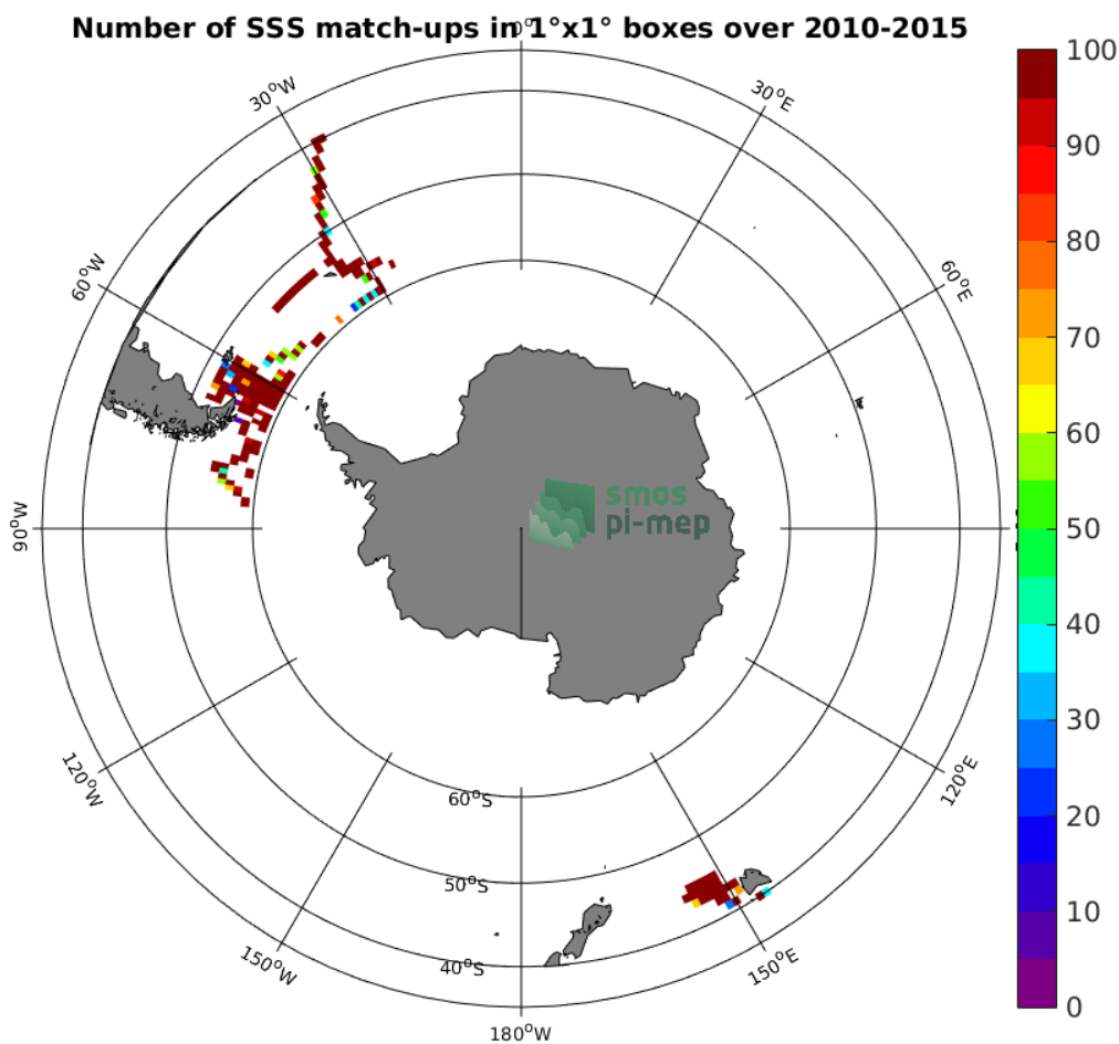
Figure 4: Number of SSS match-ups between TSG-SAMOS SSS and the CCI-L4-ESA-MERGED-OI-V1.8-7DAY-RUNNING SSS product for the Roaring Forties and Furious Fifties Pi-MEP region over 1°x1° boxes and for the full satellite product period.
