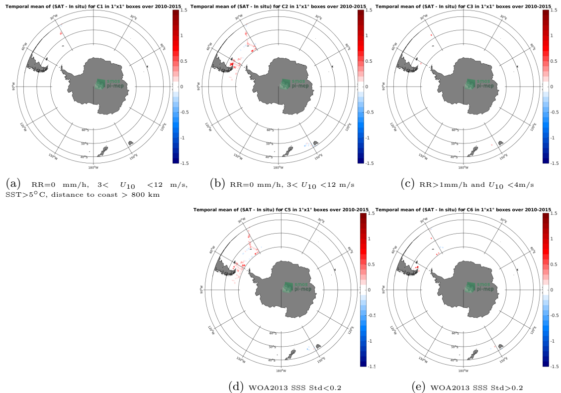
Figure 12: Temporal mean gridded over spatial boxes of size 1^\circ \times 1^\circ of \Delta SSS (CCI-L4-ESA-MERGED-OI-V1.8-7DAY-RUNNING - TSG-SAMOS) for 5 different subdatasets corresponding to:RR=0 mm/h, 3 < U_{10} < 12 m/s, SST >5^\circ\text{C} , distance to coast > 800 km (a), RR=0 mm/h, 3 < U_{10} < 12 m/s (b), RR >1 mm/h and U_{10} < 4 m/s (c), WOA2013 SSS Std <0.2 (d), WOA2013 SSS Std >0.2 (e).
