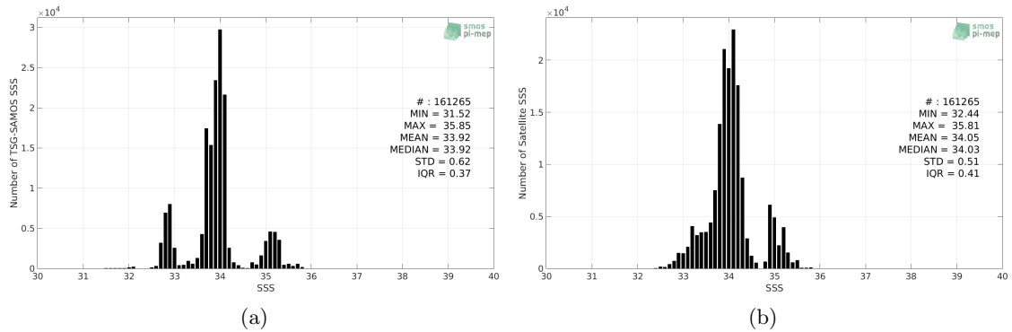
Figure 2: Histograms of SSS from TSG-SAMOS (a) and CCI-L4-ESA-MERGED-OI-V1.8-7DAY-RUNNING (b) considering all match-up pairs per bins of 0.1 over the Roaring Forties and Furious Fifties Pi-MEP region and for the full satellite product period.
