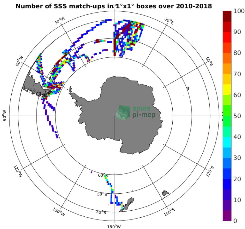
Figure 4: Number of SSS match-ups between TSG-POLARSTERN SSS and the CCI-L4-ESA-MERGED-OI-V1.8-7DAY-RUNNING SSS product for the Roaring Forties and Furious Fifties Pi-MEP region over 1^\circ \times 1^\circ boxes and for the full satellite product period.
