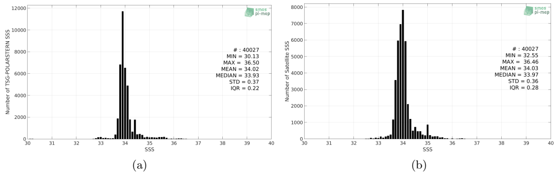
Figure 2: Histograms of SSS from TSG-POLARSTERN (a) and CCI-L4-ESA-MERGED-OI-V1.8-7DAY-RUNNING (b) considering all match-up pairs per bins of 0.1 over the Roaring Forties and Furious Fifties Pi-MEP region and for the full satellite product period.
