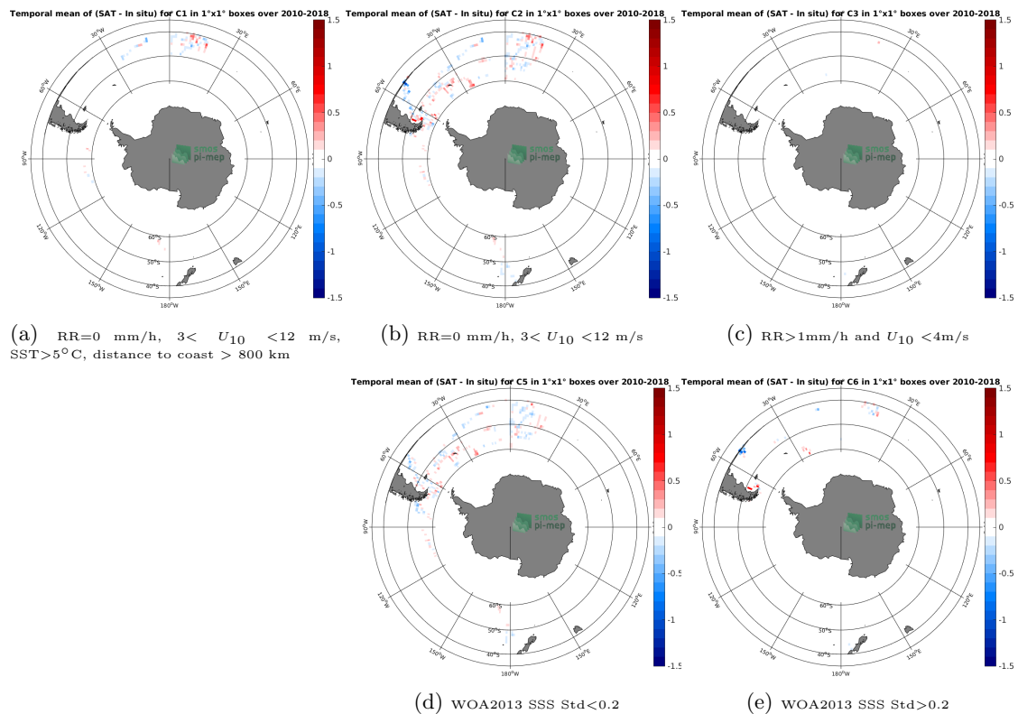
Figure 12: Temporal mean gridded over spatial boxes of size 1^\circ \times 1^\circ of \Delta SSS (CCI-L4-ESA-MERGED-OI-V1.8-7DAY-RUNNING - TSG-POLARSTERN) for 5 different subdatasets corresponding to:RR=0 mm/h, 3 < U_{10} < 12 m/s, SST >5^\circ C, distance to coast > 800 km (a), RR=0 mm/h, 3 < U_{10} < 12 m/s (b), RR >1 mm/h and U_{10} < 4 m/s (c), WOA2013 SSS Std <0.2 (d), WOA2013 SSS Std >0.2 (e).
