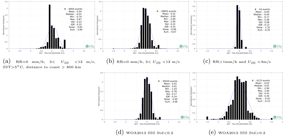
Figure 13: Normalized histogram of \Delta SSS (CCI-L4-ESA-MERGED-OI-V1.8-7DAY-RUNNING - TSG-POLARSTERN) for 5 different subdatasets corresponding to: RR=0 mm/h, 3 < U_{10} < 12 m/s, SST>5°C, distance to coast > 800 km (a), RR=0 mm/h, 3 < U_{10} < 12 m/s (b), RR>1mm/h and U_{10} < 4 m/s (c), WOA2013 SSS Std<0.2 (d), WOA2013 SSS Std>0.2 (e).
