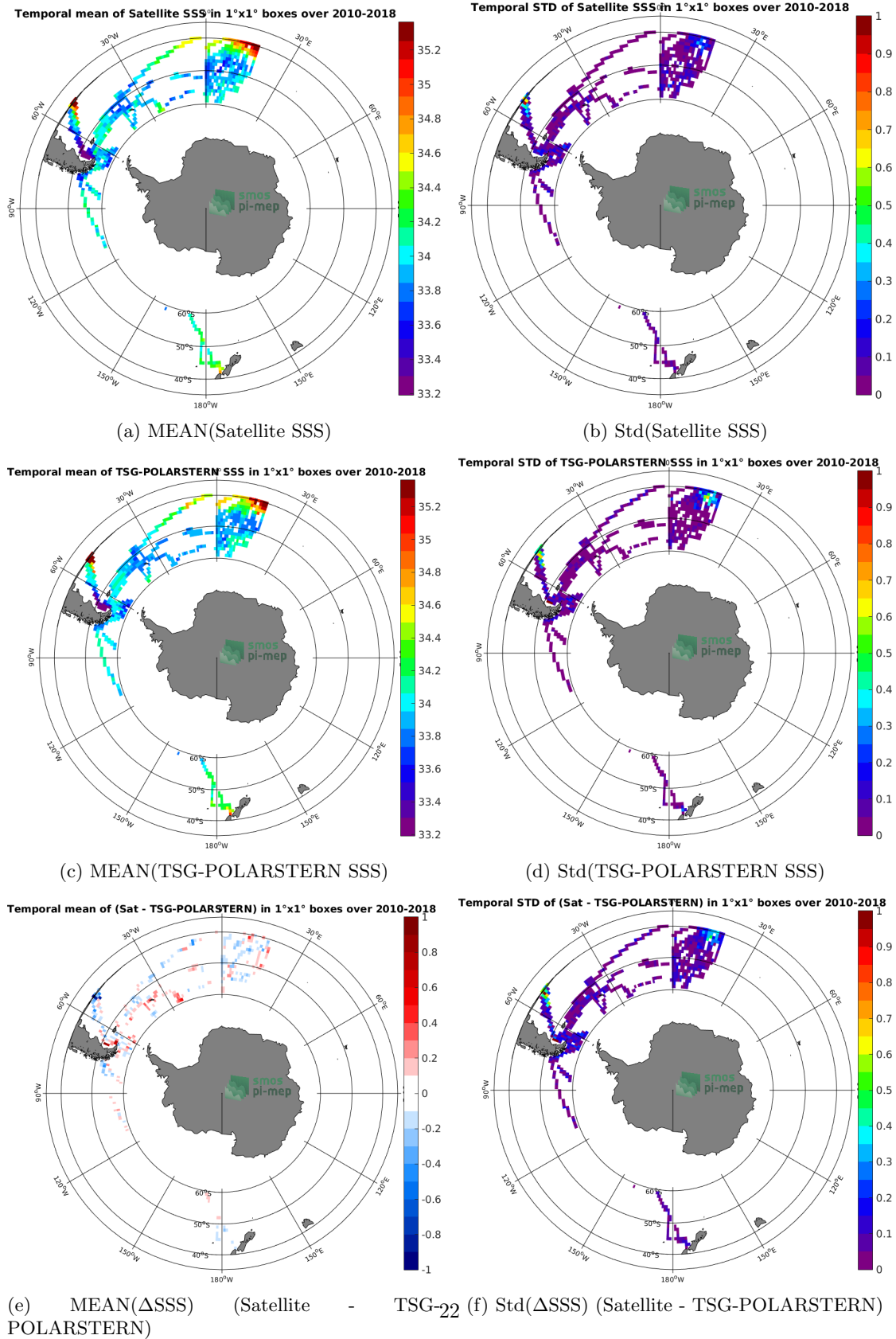
Figure 6: Temporal mean (left) and Std (right) of SSS from CCI-L4-ESA-MERGED-OI-V1.8-7DAY-RUNNING (top), TSG-POLARSTERN (middle), and of \Delta SSS (Satellite - TSG-POLARSTERN). Only match-up pairs are used to generate these maps.
