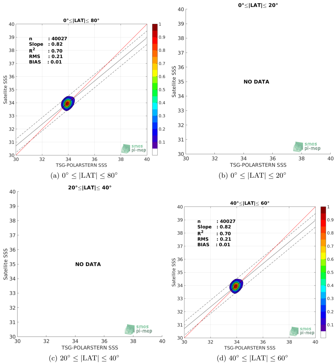
Figure 9: Contour maps of the concentration of CCI-L4-ESA-MERGED-OI-V1.8-7DAY-RUNNING SSS (y-axis) versus TSG-POLARSTERN SSS (x-axis) at match-up pairs for different latitude bands. For each plot, the red line shows x=y . The black thin and dashed lines indicate a linear fit through the data cloud and the \pm 95\% confidence levels, respectively. The number match-up pairs n , the slope and R^2 coefficient of the linear fit, the root mean square (RMS) and the mean bias between satellite and in situ data are indicated for each latitude band in each plots.
