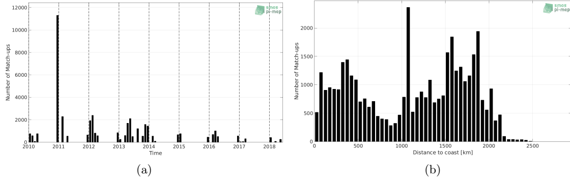
Figure 1: Number of match-ups between TSG-POLARSTERN and CCI-L4-ESA-MERGED-OI-V1.8-7DAY-RUNNING SSS as a function of time (a) and as function of the distance to coast (b) over the Roaring Forties and Furious Fifties Pi-MEP region and for the full satellite product period.
