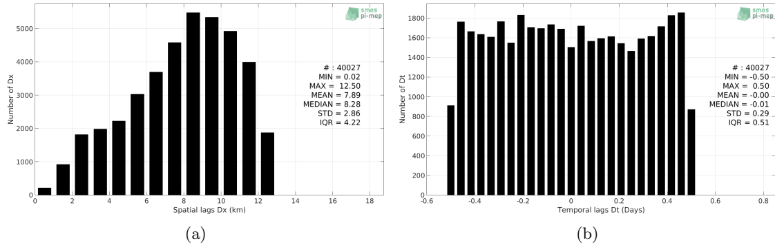
Figure 5: Histograms of the spatial (a) and temporal (b) lags between the time of the TSG-POLARSTERN measurements and the date of the corresponding CCI-L4-ESA-MERGED-OI-V1.8-7DAY-RUNNING SSS product.
