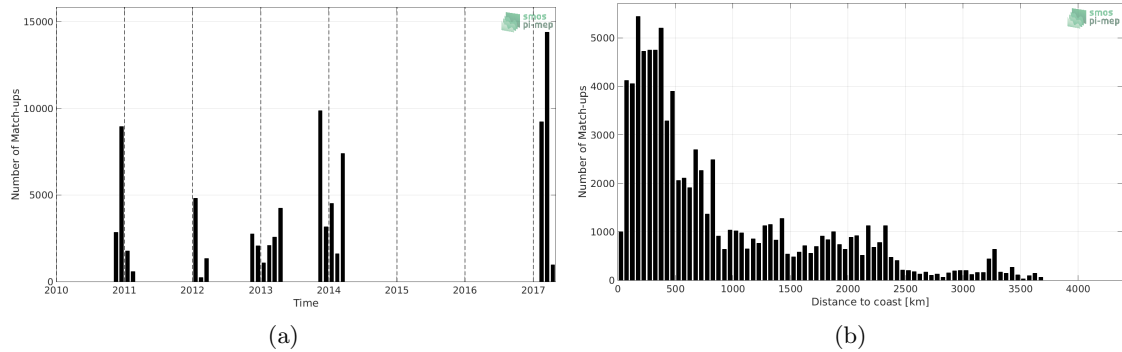
Figure 1: Number of match-ups between TSG-GOSUD-Sailing-ship and CCI-L4-ESA-MERGED-OI-V1.8-7DAY-RUNNING SSS as a function of time (a) and as function of the distance to coast (b) over the Roaring Forties and Furious Fifties Pi-MEP region and for the full satellite product period.
