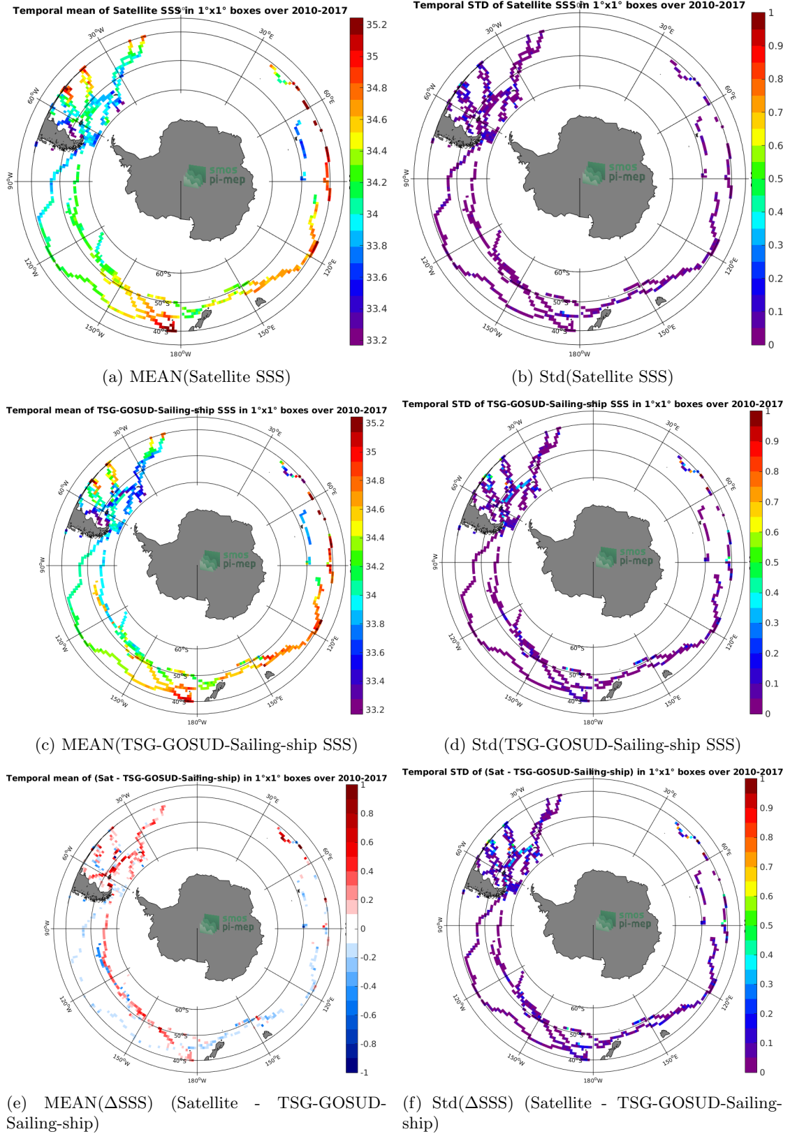
Figure 6: Temporal mean (left) and Std (right) of SSS from CCI-L4-ESA-MERGED-OI-V1.8-7DAY-RUNNING (top), TSG-GOSUD-Sailing-ship (middle), and of \Delta SSS (Satellite - TSG-GOSUD-Sailing-ship). Only match-up pairs are used to generate these maps.
