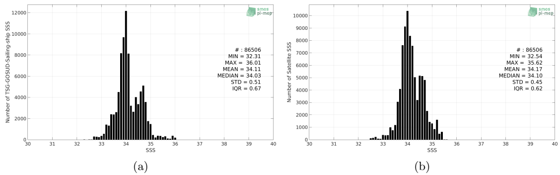
Figure 2: Histograms of SSS from TSG-GOSUD-Sailing-ship (a) and CCI-L4-ESA-MERGED-OI-V1.8-7DAY-RUNNING (b) considering all match-up pairs per bins of 0.1 over the Roaring Forties and Furious Fifties Pi-MEP region and for the full satellite product period.
