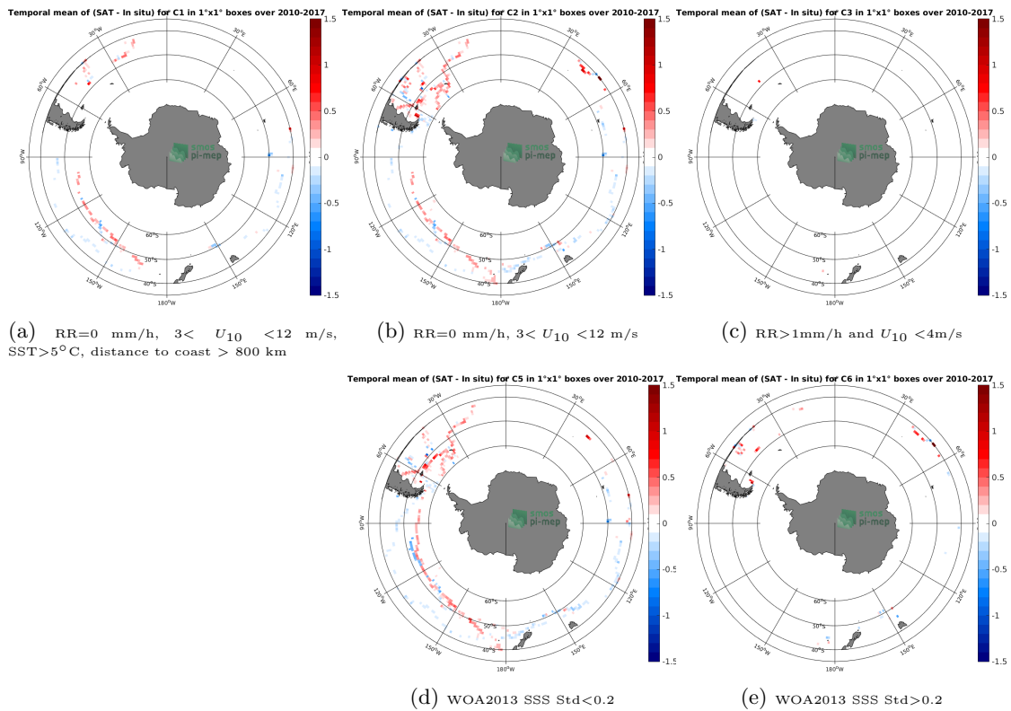
Figure 12: Temporal mean gridded over spatial boxes of size 1°x1° of \Delta SSS (CCI-L4-ESA-MERGED-OI-V1.8-7DAY-RUNNING - TSG-GOSUD-Sailing-ship) for 5 different subdatasets corresponding to:RR=0 mm/h, 3 < U_{10} < 12 m/s, SST>5°C, distance to coast > 800 km (a), RR=0 mm/h, 3 < U_{10} < 12 m/s (b), RR>1mm/h and U_{10} < 4 m/s (c), WOA2013 SSS Std<0.2 (d), WOA2013 SSS Std>0.2 (e).
