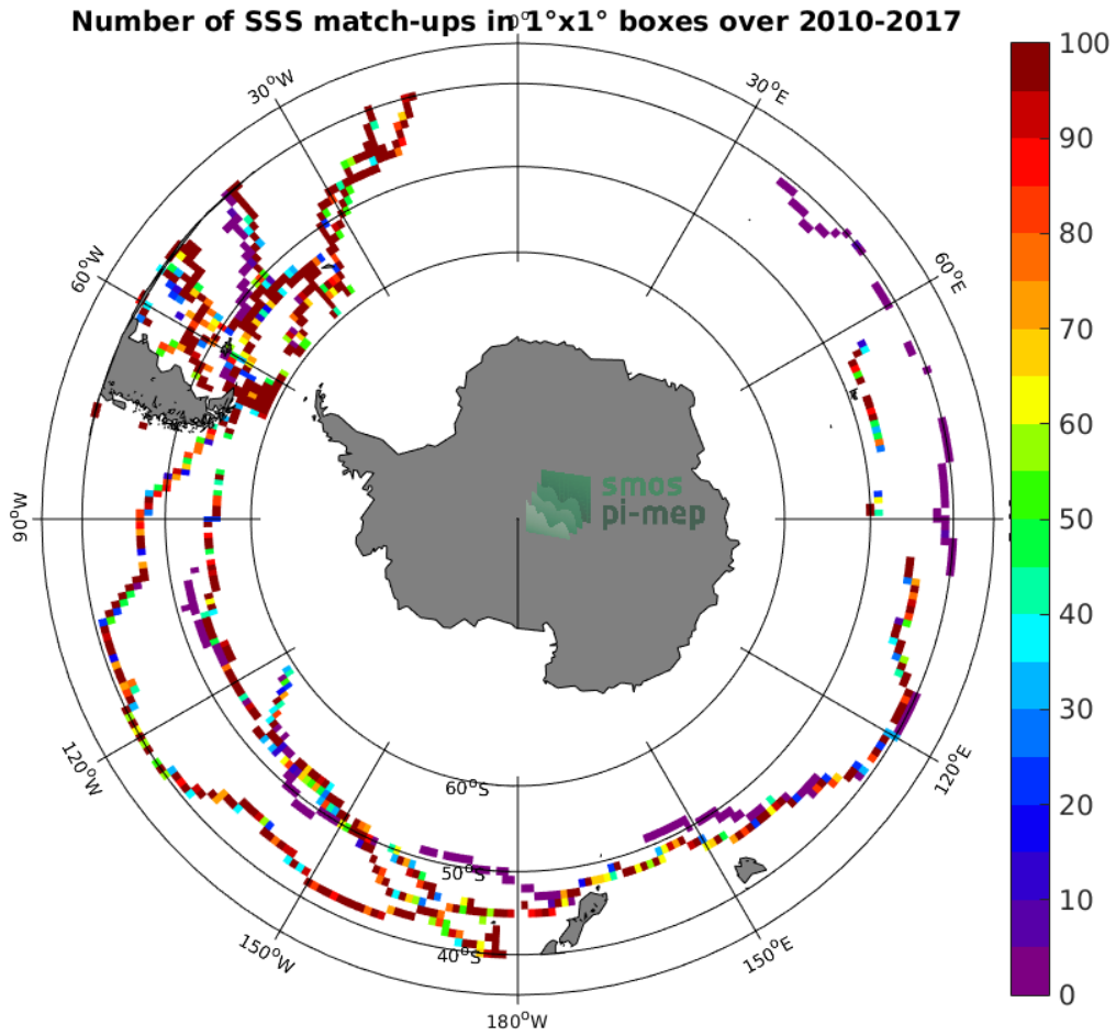
Figure 4: Number of SSS match-ups between TSG-GOSUD-Sailing-ship SSS and the CCI-L4-ESA-MERGED-OI-V1.8-7DAY-RUNNING SSS product for the Roaring Forties and Furious Fifties Pi-MEP region over 1°x1° boxes and for the full satellite product period.
