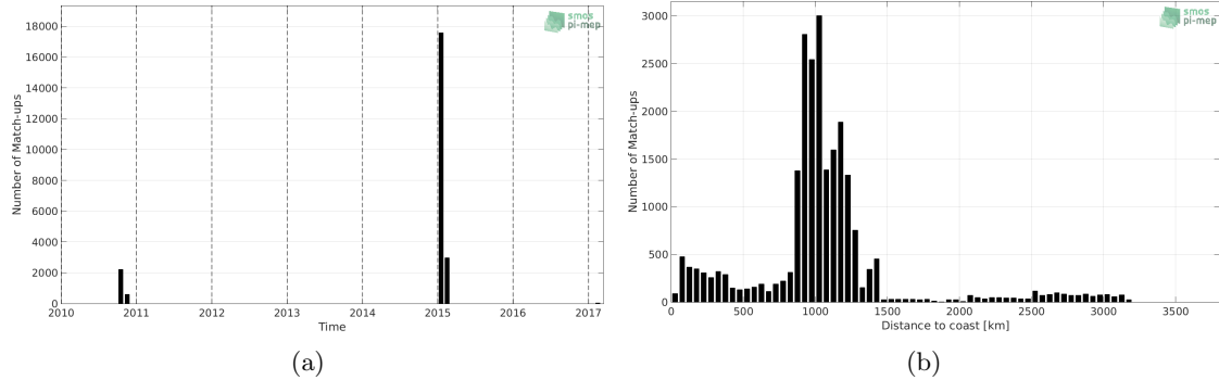
Figure 1: Number of match-ups between TSG-GOSUD-Research-vessel and CCI L4 Merged-OI v1.8 - 7-day running (ESA) SSS as a function of time (a) and as function of the distance to coast (b) over the Roaring Forties and Furious Fifties Pi-MEP region and for the full satellite product period.
