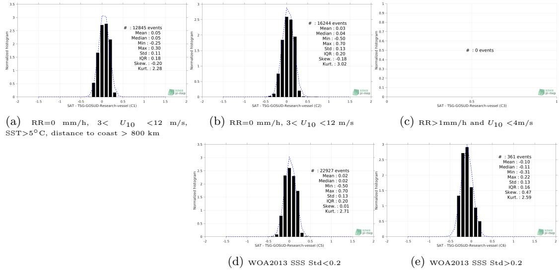
Figure 13: Normalized histogram of \Delta SSS (CCI L4 Merged-OI v1.8 - 7-day running (ESA) - TSG-GOSUD-Research-vessel) for 5 different subdatasets corresponding to: RR=0 mm/h, 3 < U_{10} < 12 m/s, SST > 5°C, distance to coast > 800 km (a), RR=0 mm/h, 3 < U_{10} < 12 m/s (b), RR > 1mm/h and U_{10} < 4 m/s (c), WOA2013 SSS Std < 0.2 (d), WOA2013 SSS Std > 0.2 (e).
