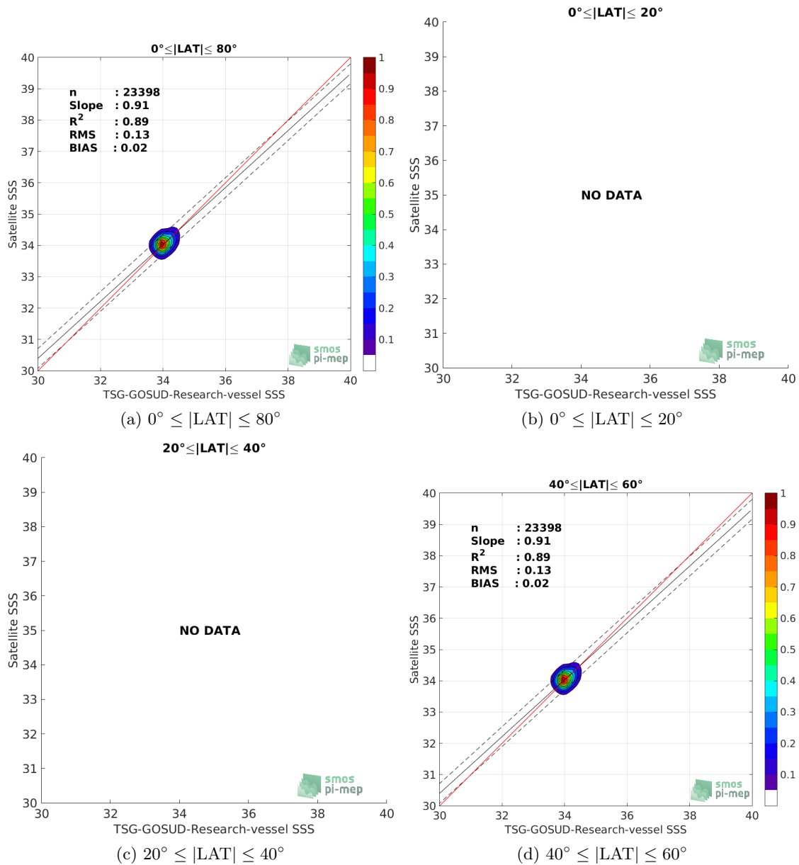
Figure 9: Contour maps of the concentration of CCI L4 Merged-OI v1.8 - 7-day running (ESA) SSS (y-axis) versus TSG-GOSUD-Research-vessel SSS (x-axis) at match-up pairs for different latitude bands. For each plot, the red line shows x=y . The black thin and dashed lines indicate a linear fit through the data cloud and the \pm 95\% confidence levels, respectively. The number match-up pairs n , the slope and R^2 coefficient of the linear fit, the root mean square (RMS) and the mean bias between satellite and in situ data are indicated for each latitude band in each plots.
