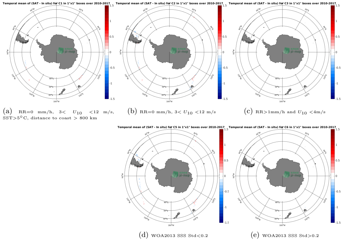
Figure 12: Temporal mean gridded over spatial boxes of size 1°x1° of \Delta SSS (CCI L4 Merged-OI v1.8 - 7-day running (ESA) - TSG-GOSUD-Research-vessel) for 5 different subdatasets corresponding to:RR=0 mm/h, 3 < U_{10} < 12 m/s, SST>5°C, distance to coast > 800 km (a), RR=0 mm/h, 3 < U_{10} < 12 m/s (b), RR>1mm/h and U_{10} < 4 m/s (c), WOA2013 SSS Std<0.2 (d), WOA2013 SSS Std>0.2 (e).
