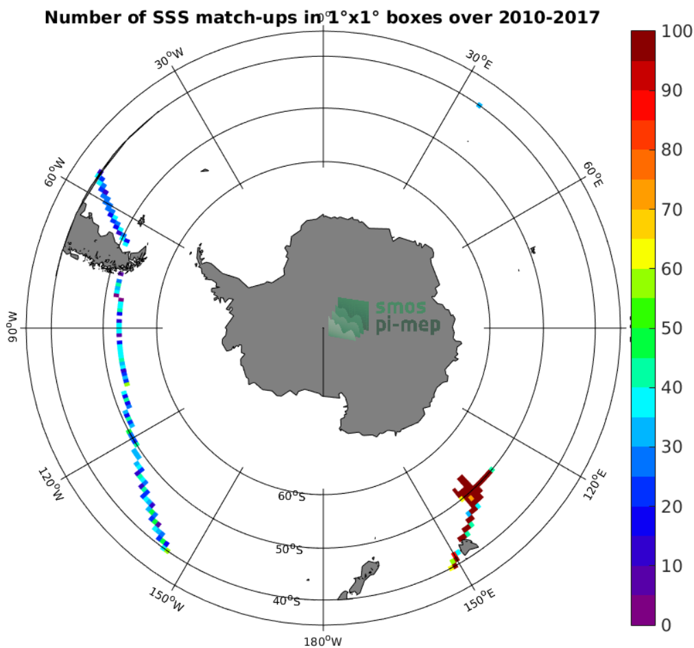
Figure 4: Number of SSS match-ups between TSG-GOSUD-Research-vessel SSS and the CCI L4 Merged-OI v1.8 - 7-day running (ESA) SSS product for the Roaring Forties and Furious Fifties Pi-MEP region over 1°x1° boxes and for the full satellite product period.
