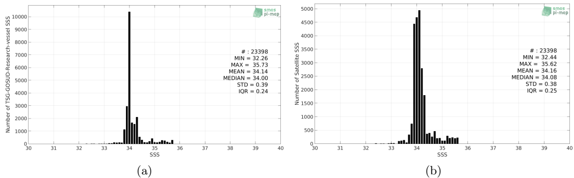
Figure 2: Histograms of SSS from TSG-GOSUD-Research-vessel (a) and CCI L4 Merged-OI v1.8 - 7-day running (ESA) (b) considering all match-up pairs per bins of 0.1 over the Roaring Forties and Furious Fifties Pi-MEP region and for the full satellite product period.
