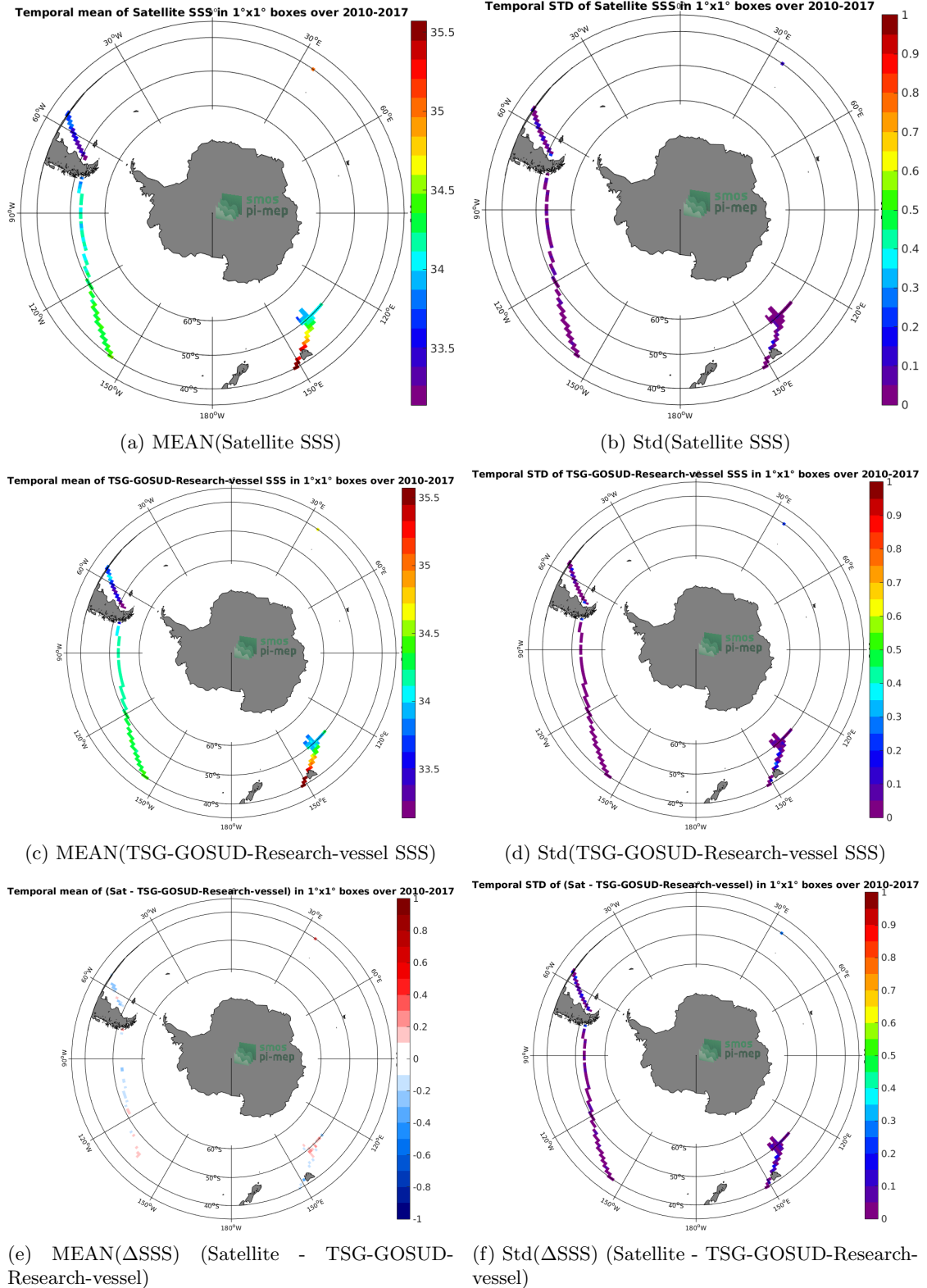
Figure 6: Temporal mean (left) and Std (right) of SSS from CCI L4 Merged-OI v1.8 - 7-day running (ESA) (top), TSG-GOSUD-Research-vessel (middle), and of \Delta SSS (Satellite - TSG-GOSUD-Research-vessel). Only match-up pairs are used to generate these maps.
